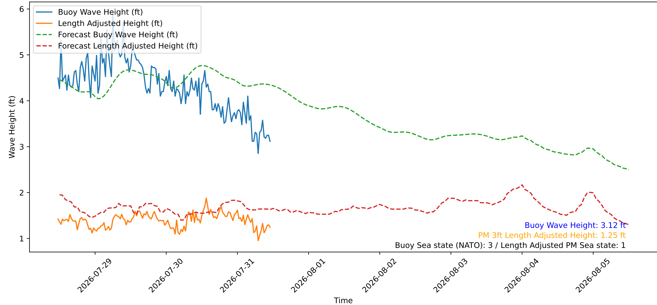
Wave Heights over Time for Oceanside Harbor at 2026-07-31 11:40:26
