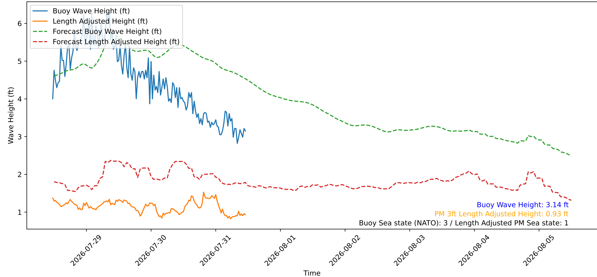
Wave Heights over Time for Green Beach at 2026-07-31 11:41:09
