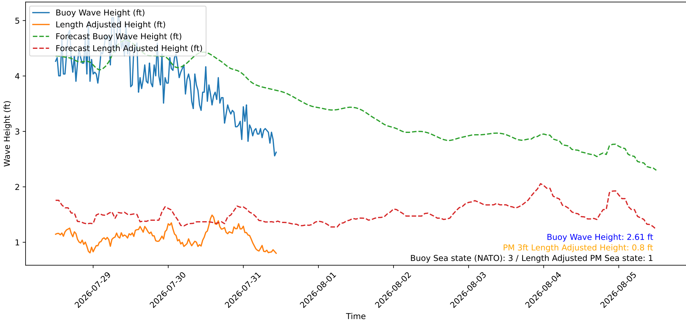
Wave Heights over Time for Red Beach at 2026-07-31 11:40:46
