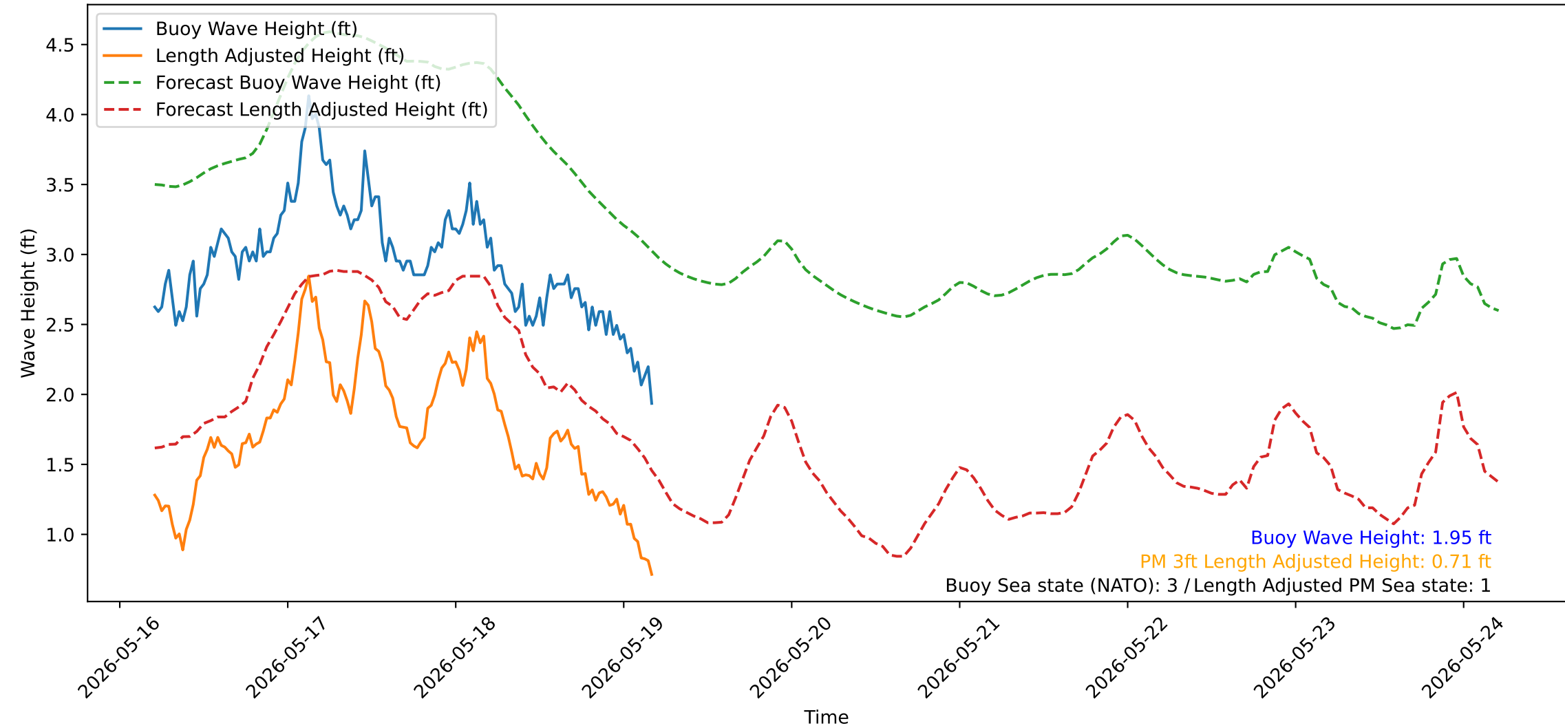
Wave Heights over Time for Red Beach at 2026-05-19 04:40:52
