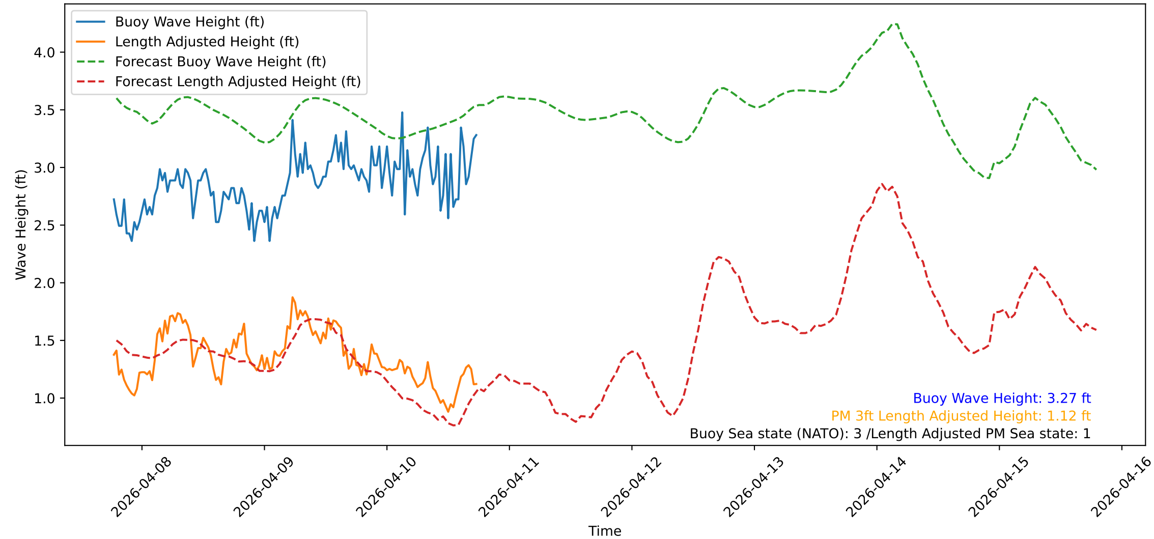
Wave Heights over Time for Green Beach at 2026-04-10 18:31:12
