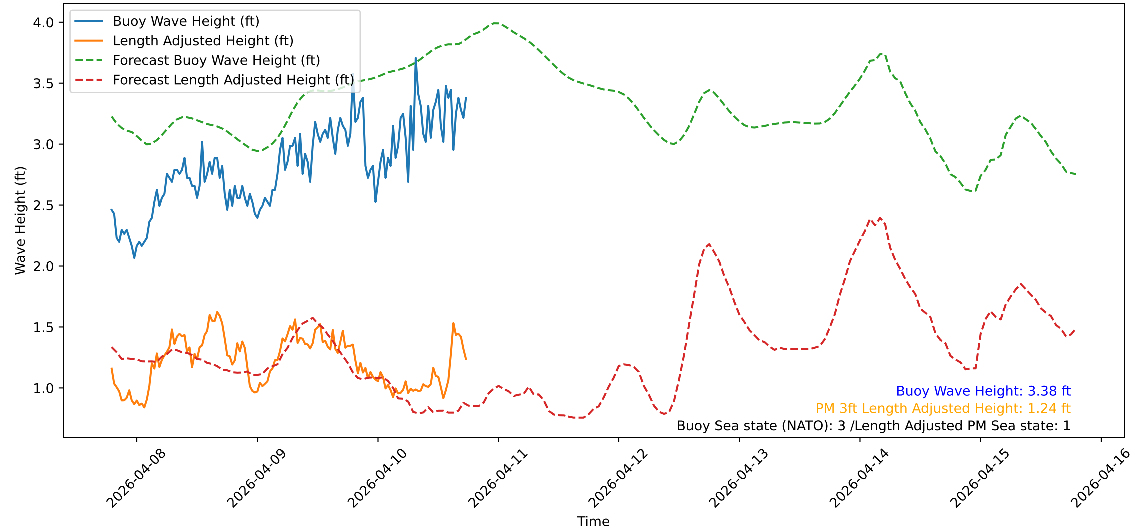
Wave Heights over Time for Red Beach at 2026-04-10 18:30:49
