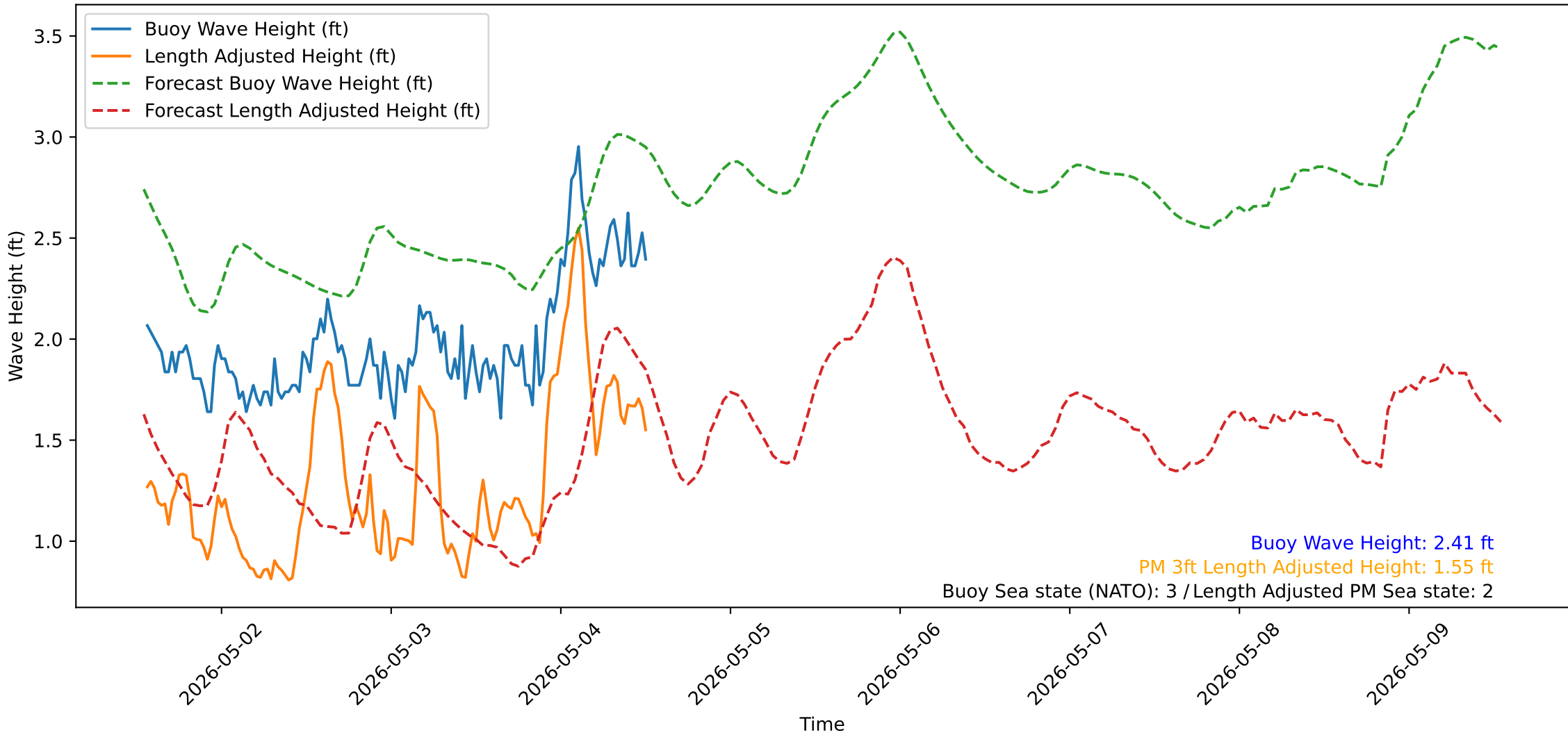
Wave Heights over Time for Red Beach at 2026-05-04 13:00:50
