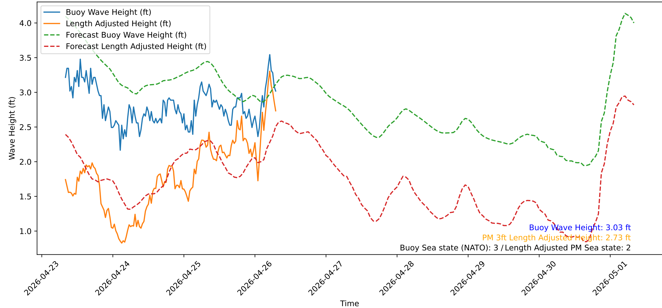
Wave Heights over Time for Red Beach at 2026-04-26 07:40:50
