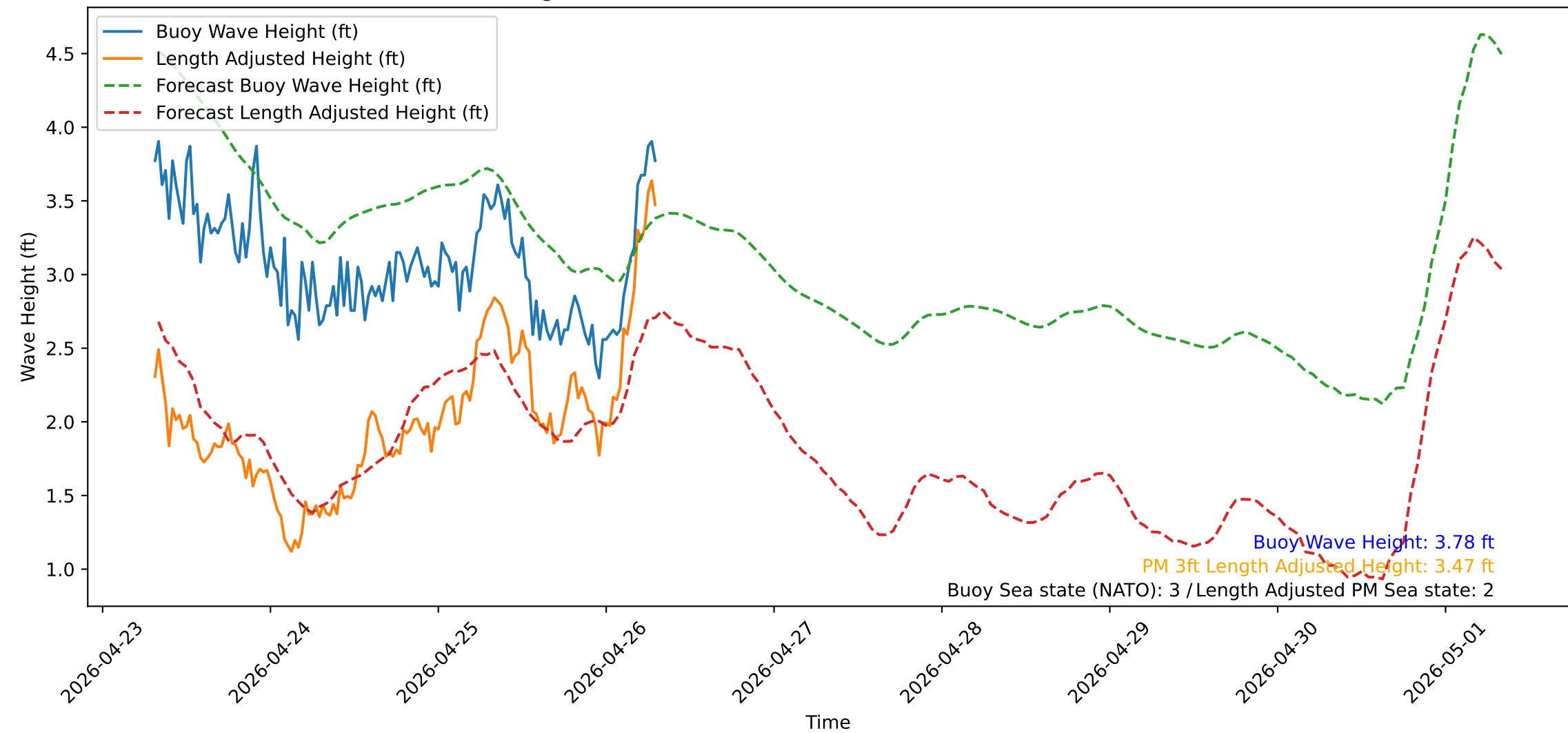
Wave Heights over Time for Oceanside Harbor at 2026-04-26 07:40:31
