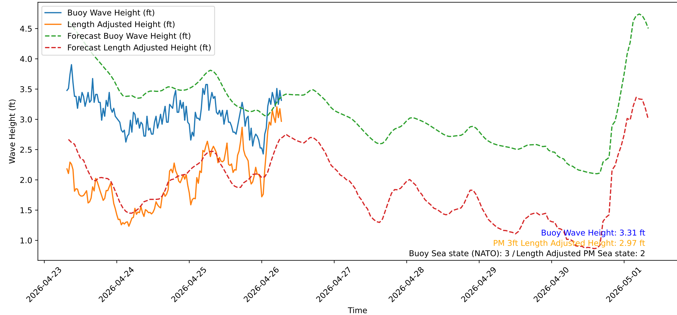
Wave Heights over Time for Green Beach at 2026-04-26 07:41:12
