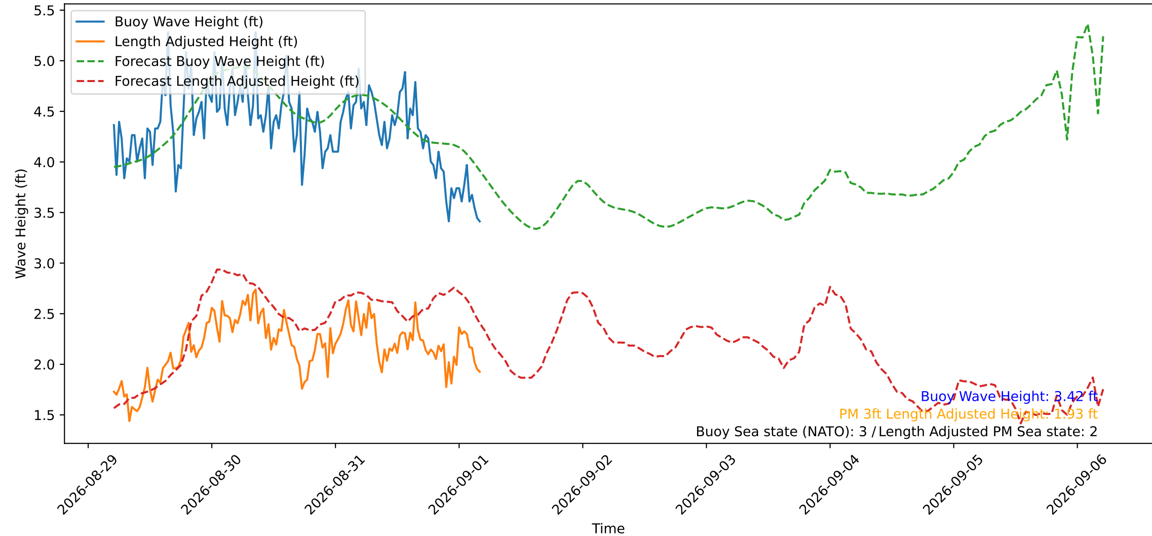
Wave Heights over Time for Oceanside Harbor at 2026-09-01 04:50:30
