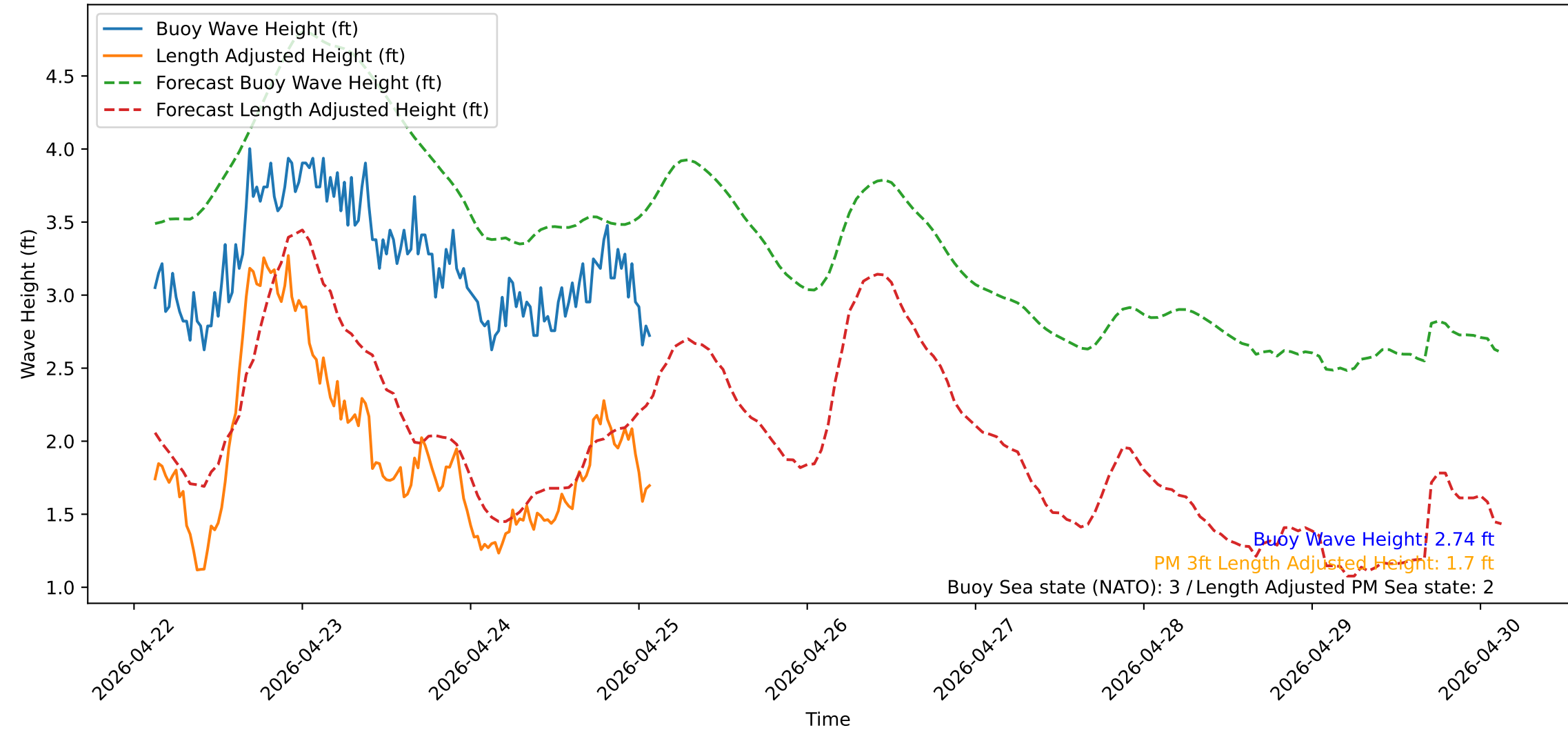
Wave Heights over Time for Green Beach at 2026-04-25 02:51:13
