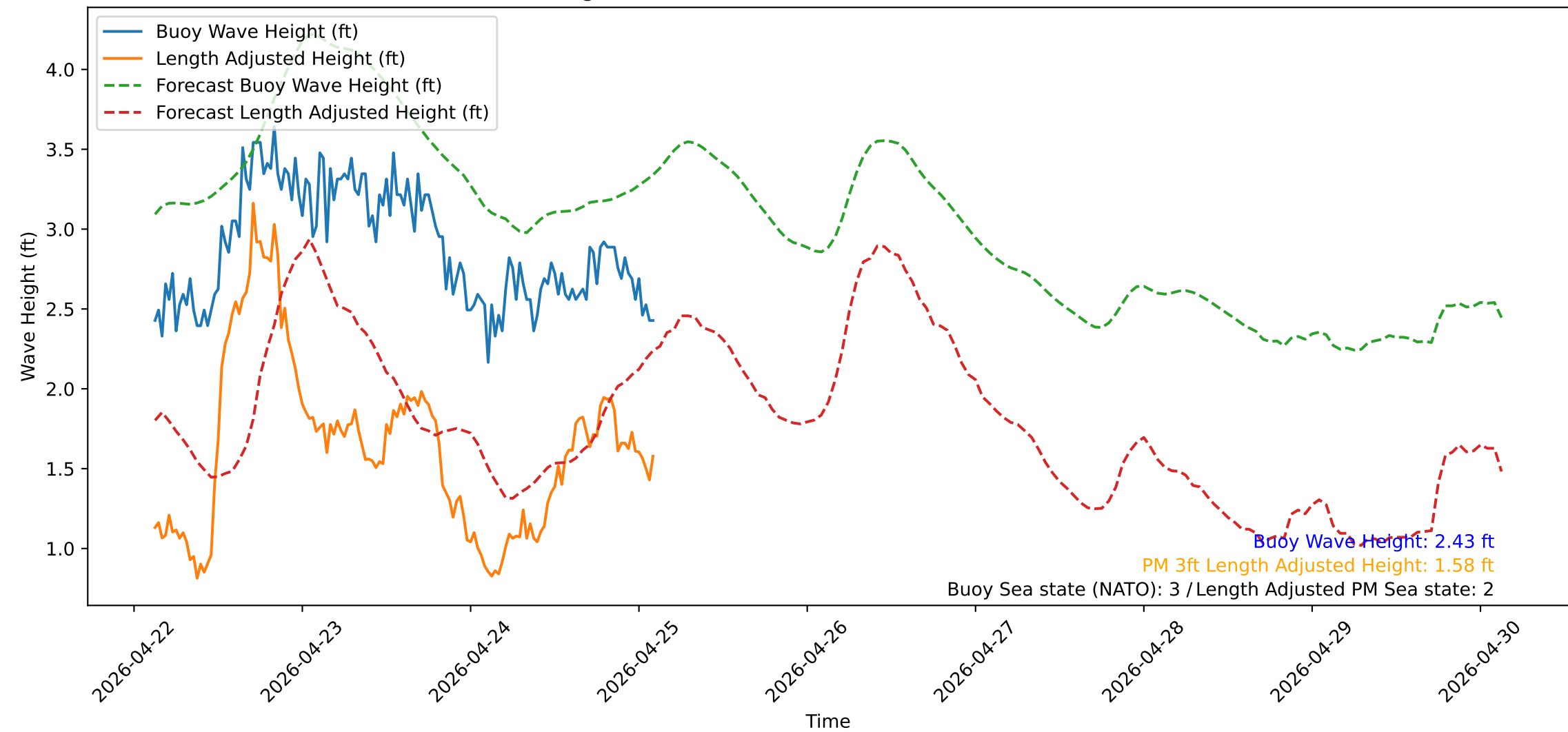
Wave Heights over Time for Red Beach at 2026-04-25 02:50:51
