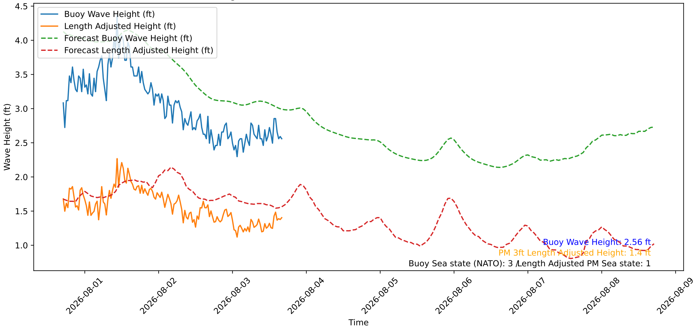
Wave Heights over Time for Oceanside Harbor at 2026-08-03 16:50:26
