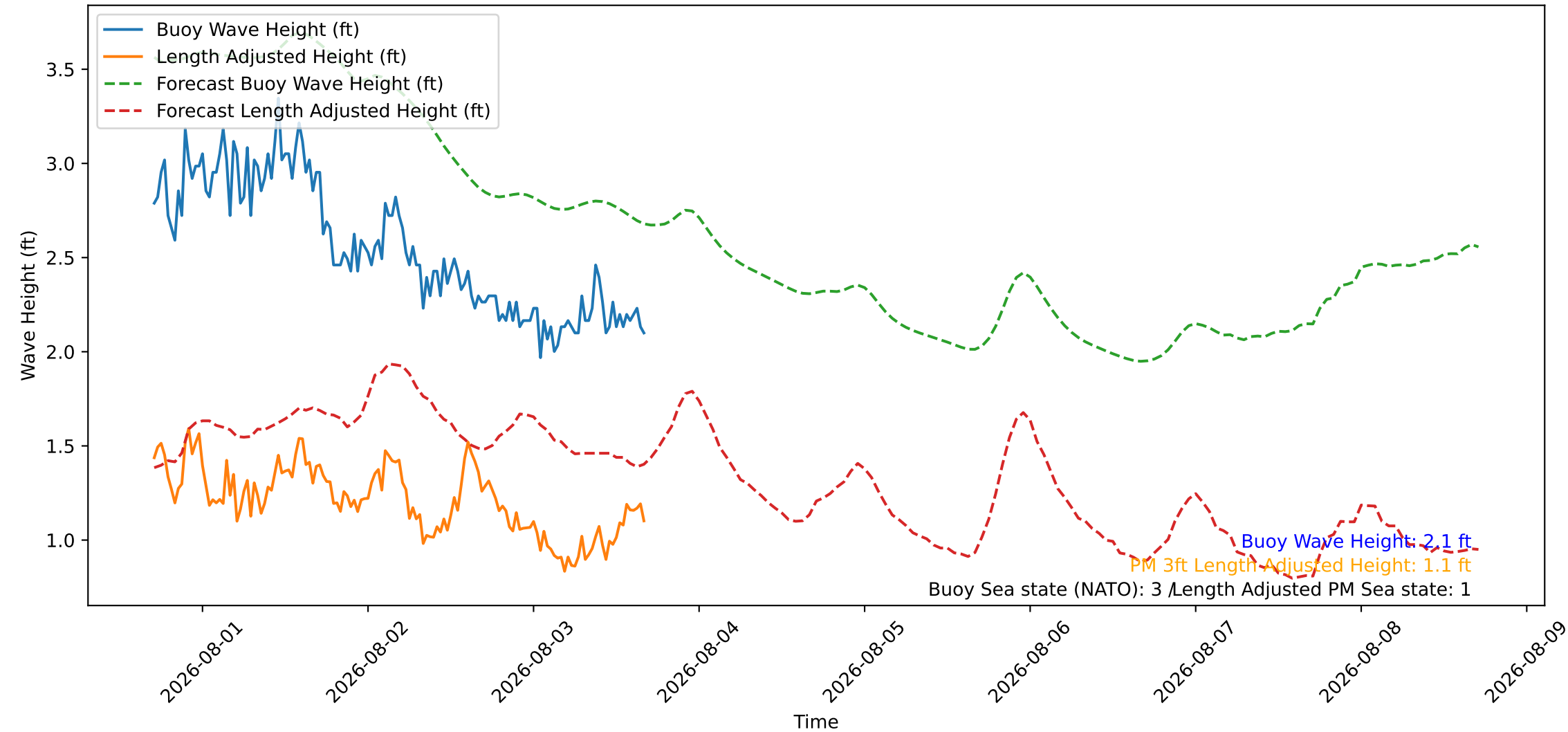
Wave Heights over Time for Red Beach at 2026-08-03 16:50:47
