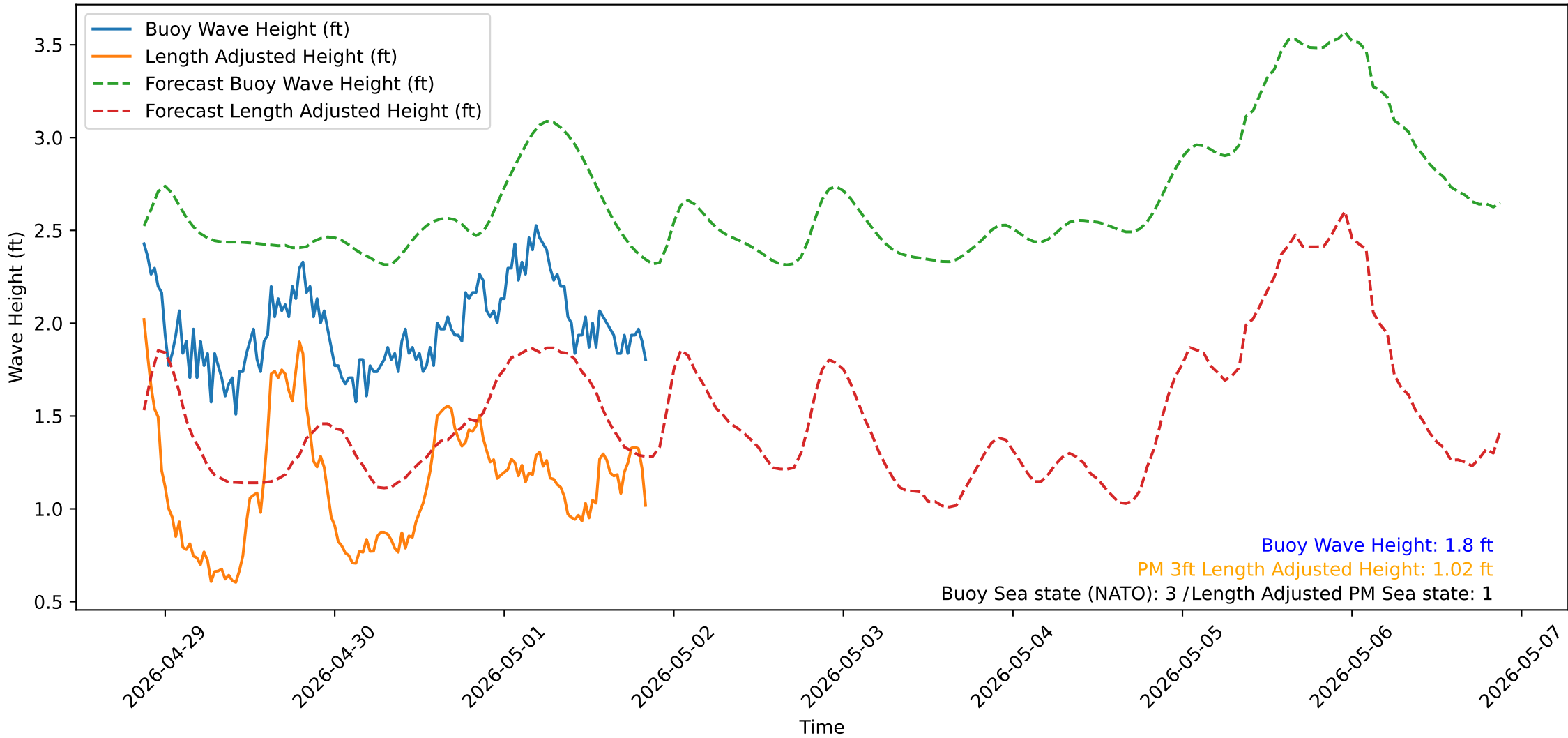
Wave Heights over Time for Red Beach at 2026-05-01 20:50:52
