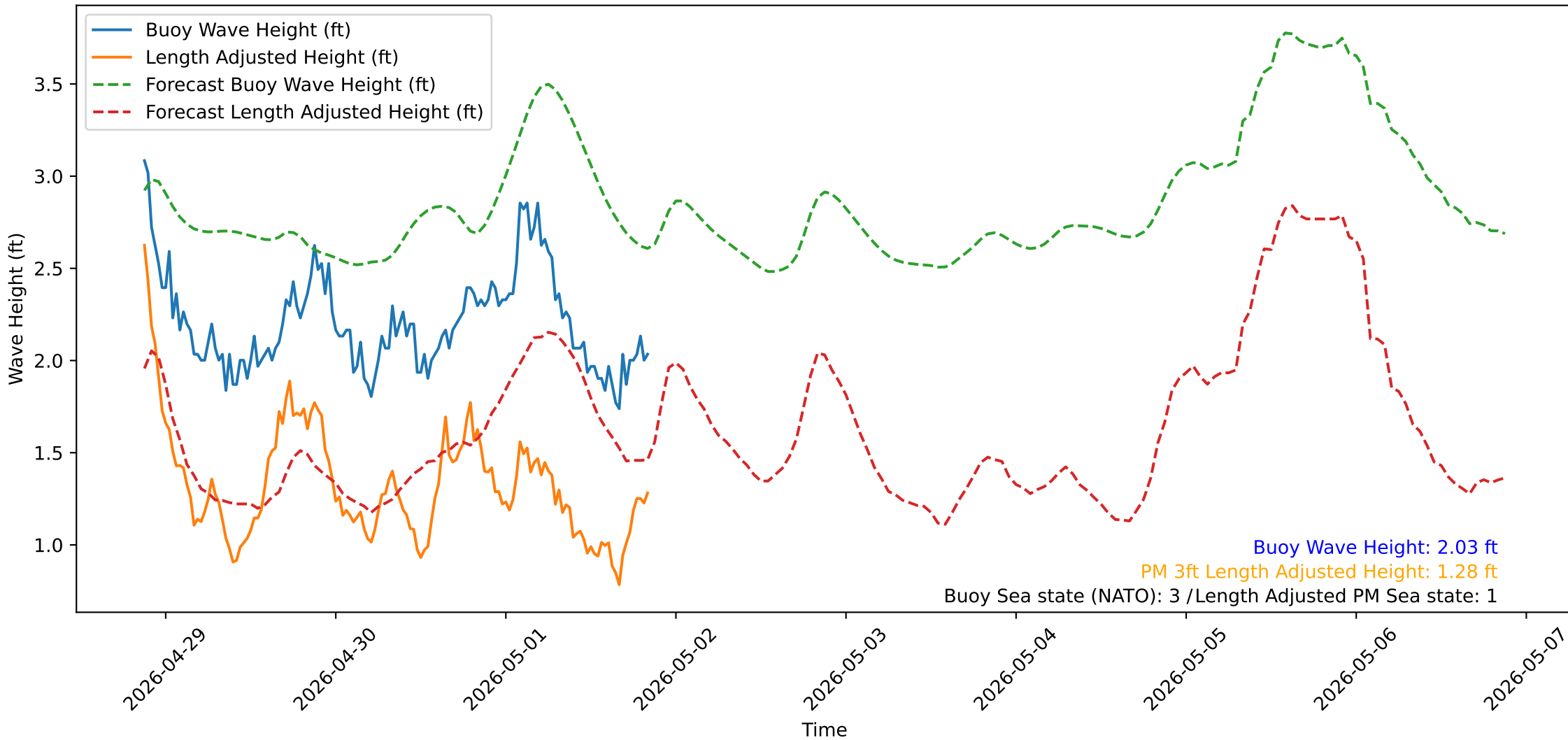
Wave Heights over Time for Green Beach at 2026-05-01 20:51:14
