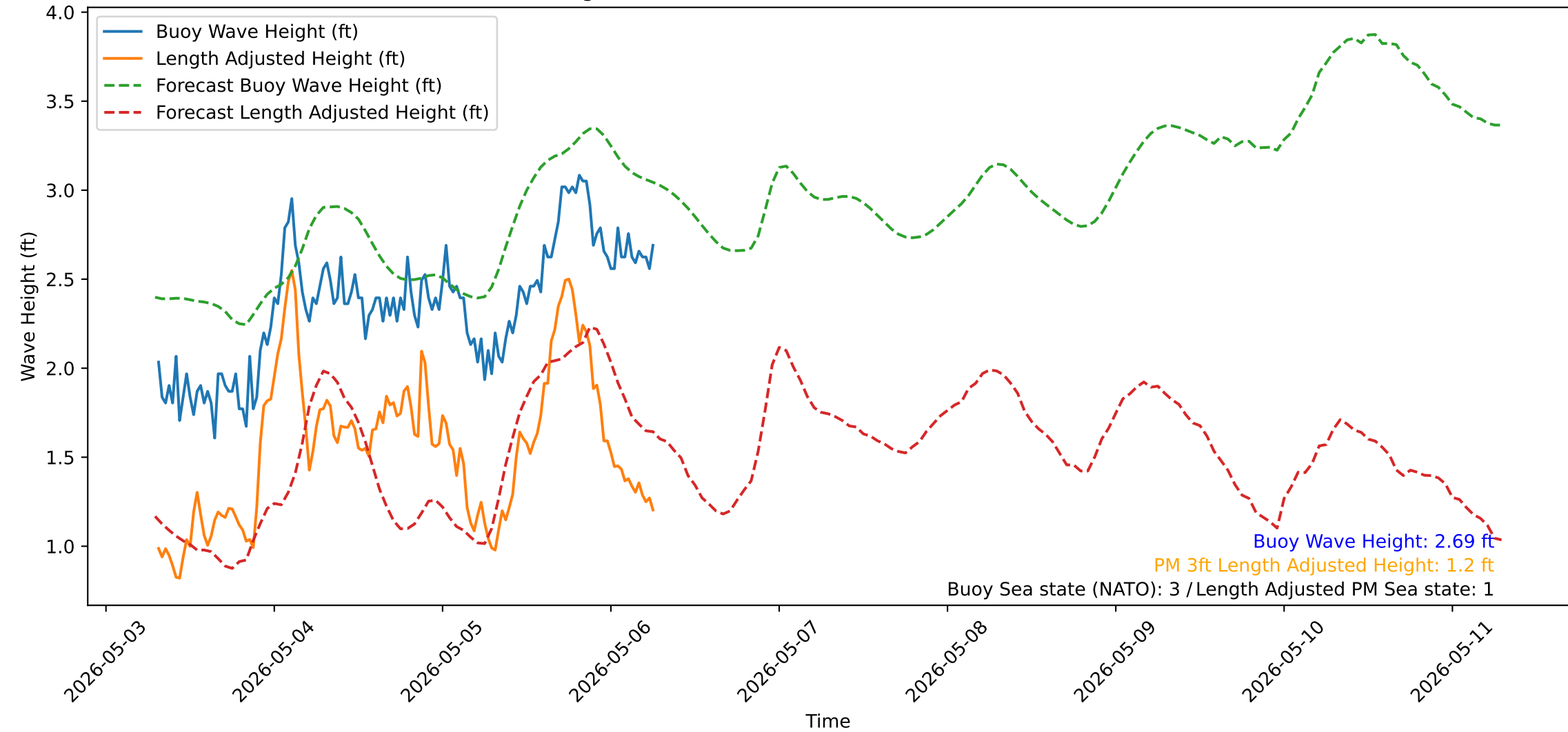
Wave Heights over Time for Red Beach at 2026-05-06 07:00:50
