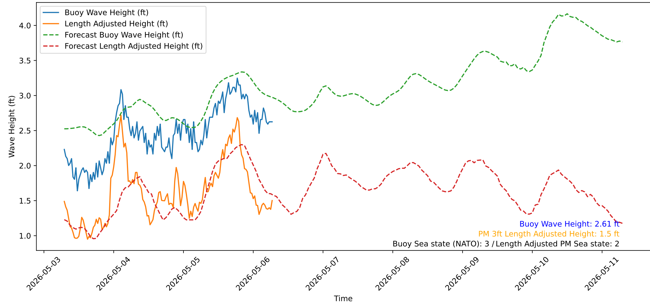
Wave Heights over Time for Oceanside Harbor at 2026-05-06 07:00:31
