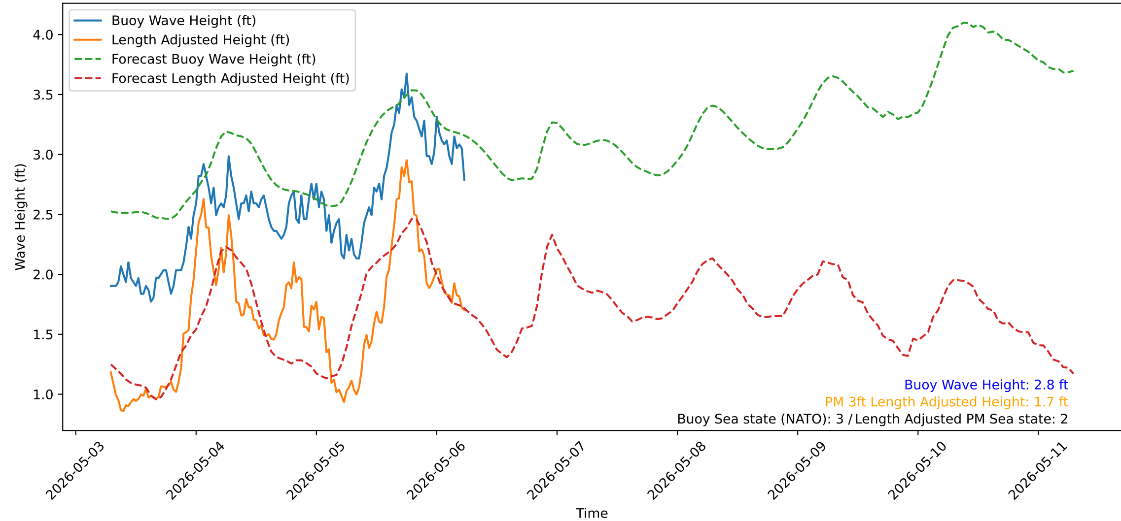
Wave Heights over Time for Green Beach at 2026-05-06 07:01:12
