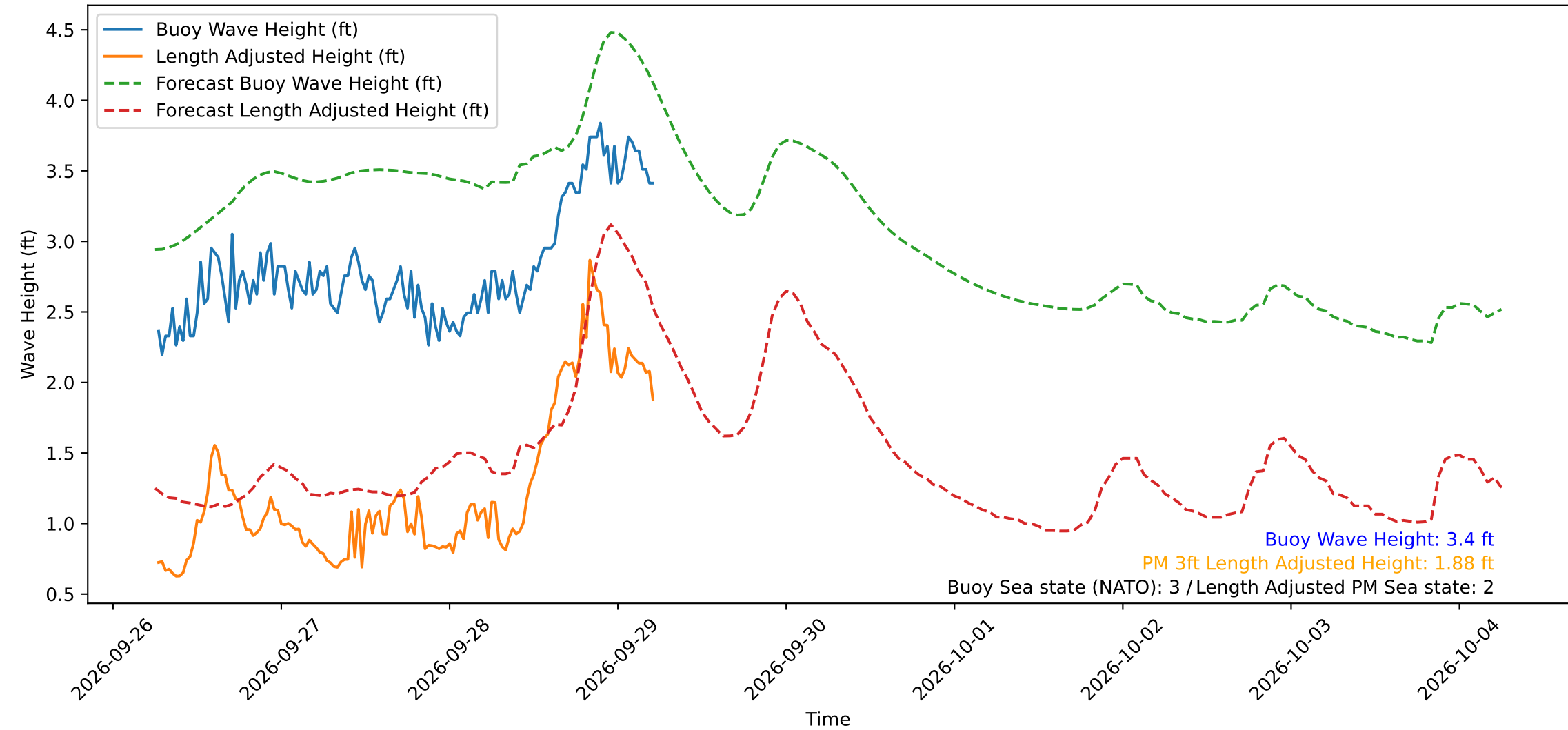
Wave Heights over Time for Red Beach at 2026-09-29 06:00:50
