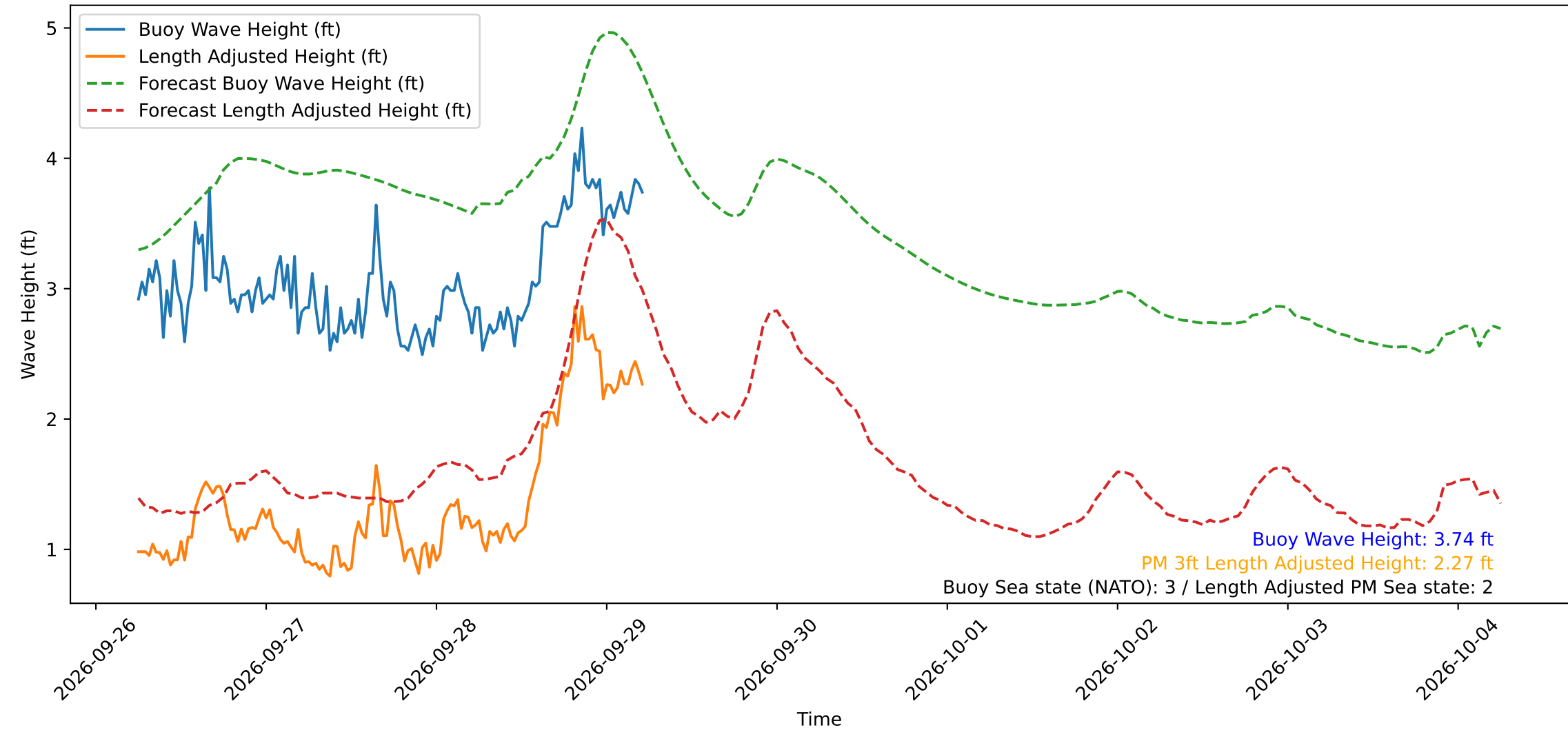
Wave Heights over Time for Oceanside Harbor at 2026-09-29 06:00:30
