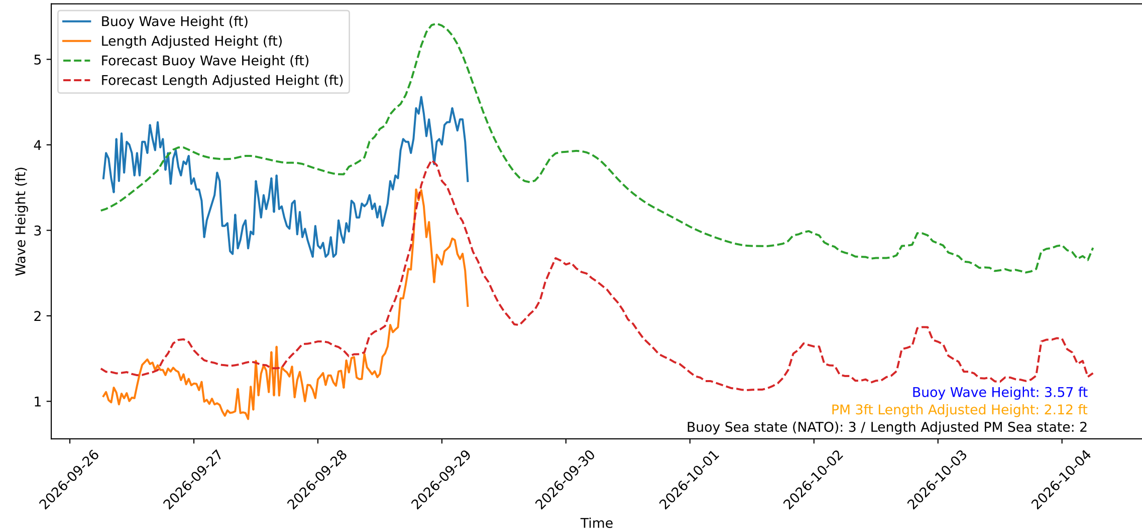
Wave Heights over Time for Green Beach at 2026-09-29 06:01:13
