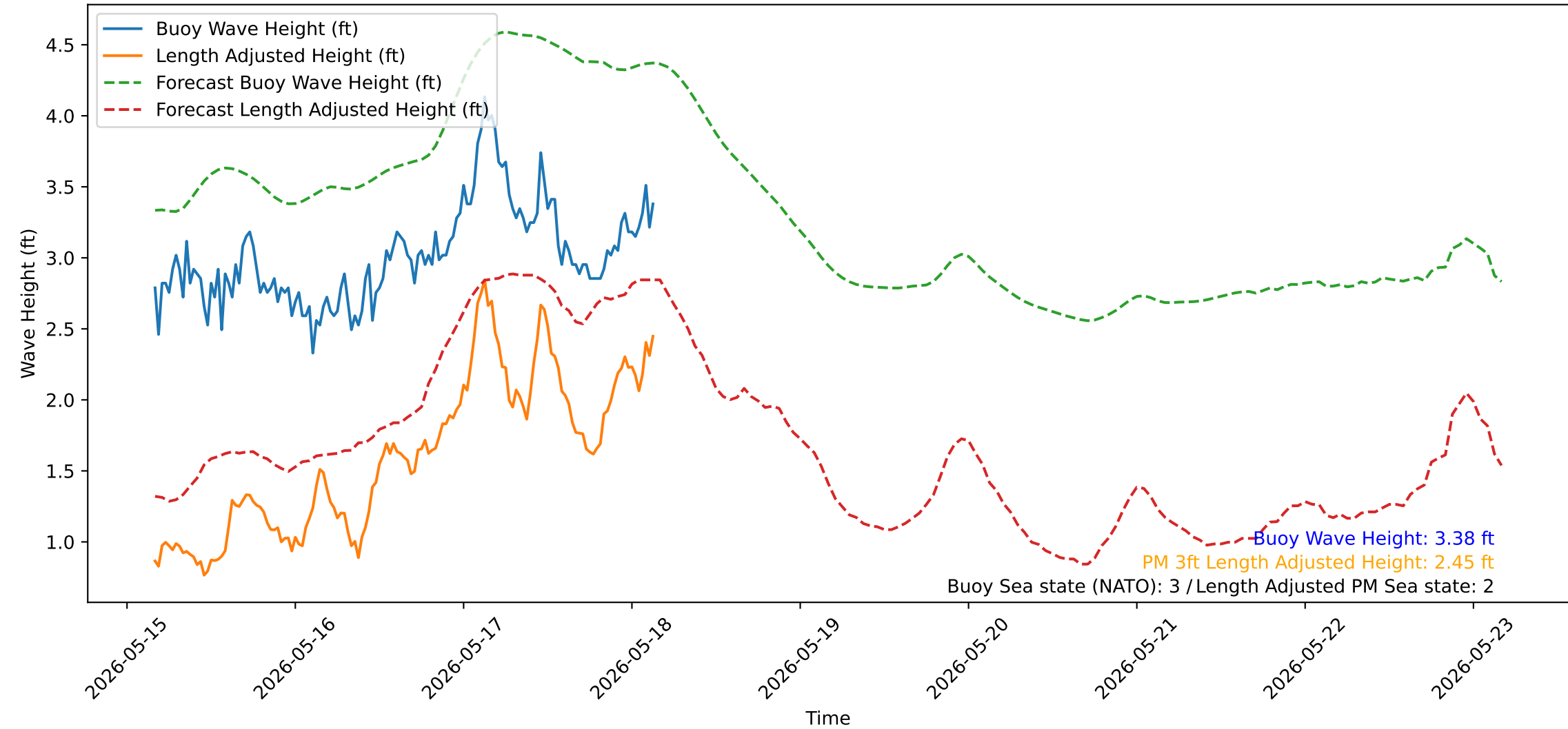
Wave Heights over Time for Red Beach at 2026-05-18 03:50:52
