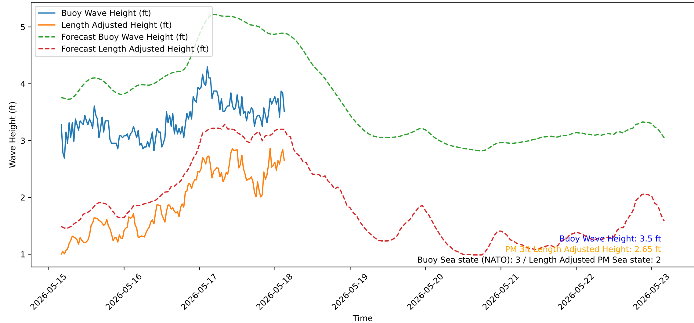
Wave Heights over Time for Oceanside Harbor at 2026-05-18 03:50:32
