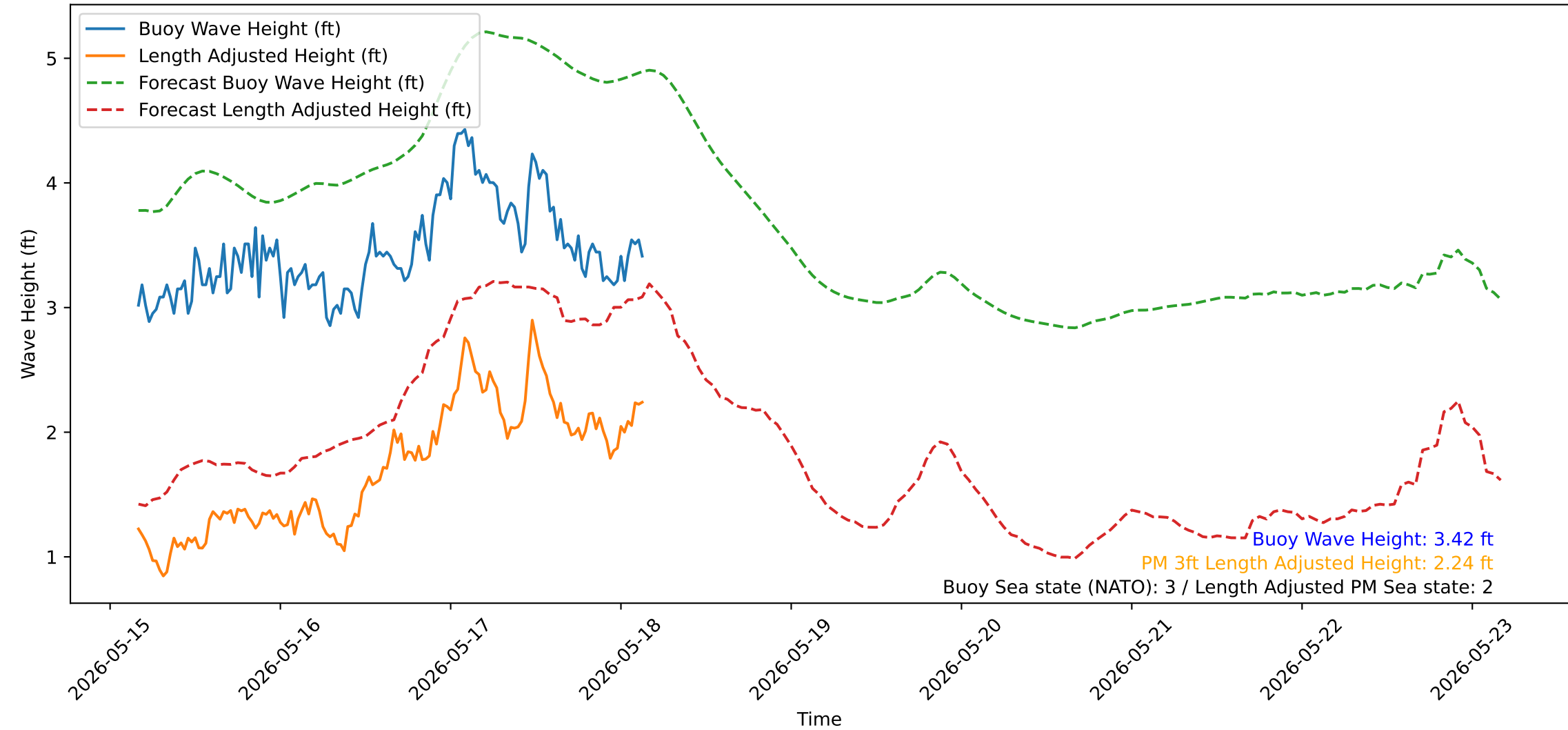
Wave Heights over Time for Green Beach at 2026-05-18 03:51:15
