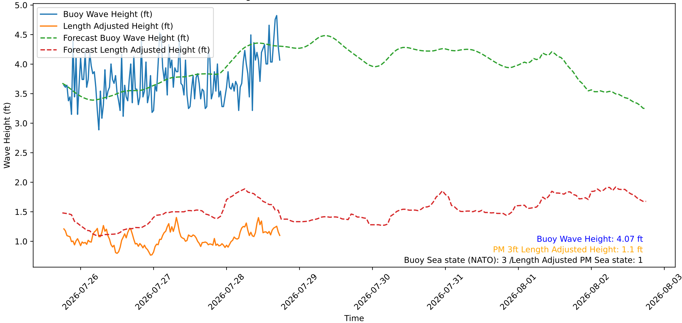
Wave Heights over Time for Red Beach at 2026-07-28 18:20:47
