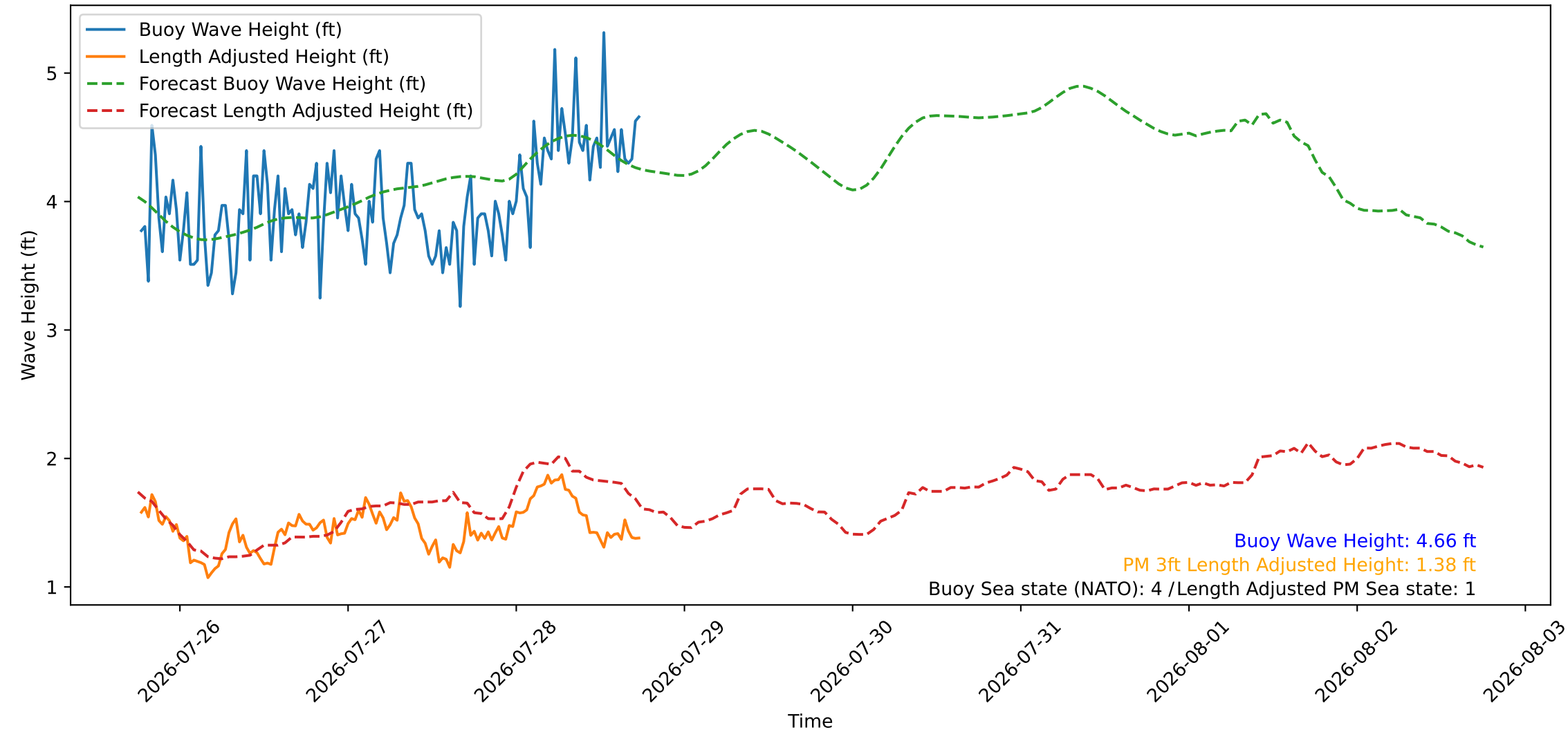
Wave Heights over Time for Oceanside Harbor at 2026-07-28 18:20:26
