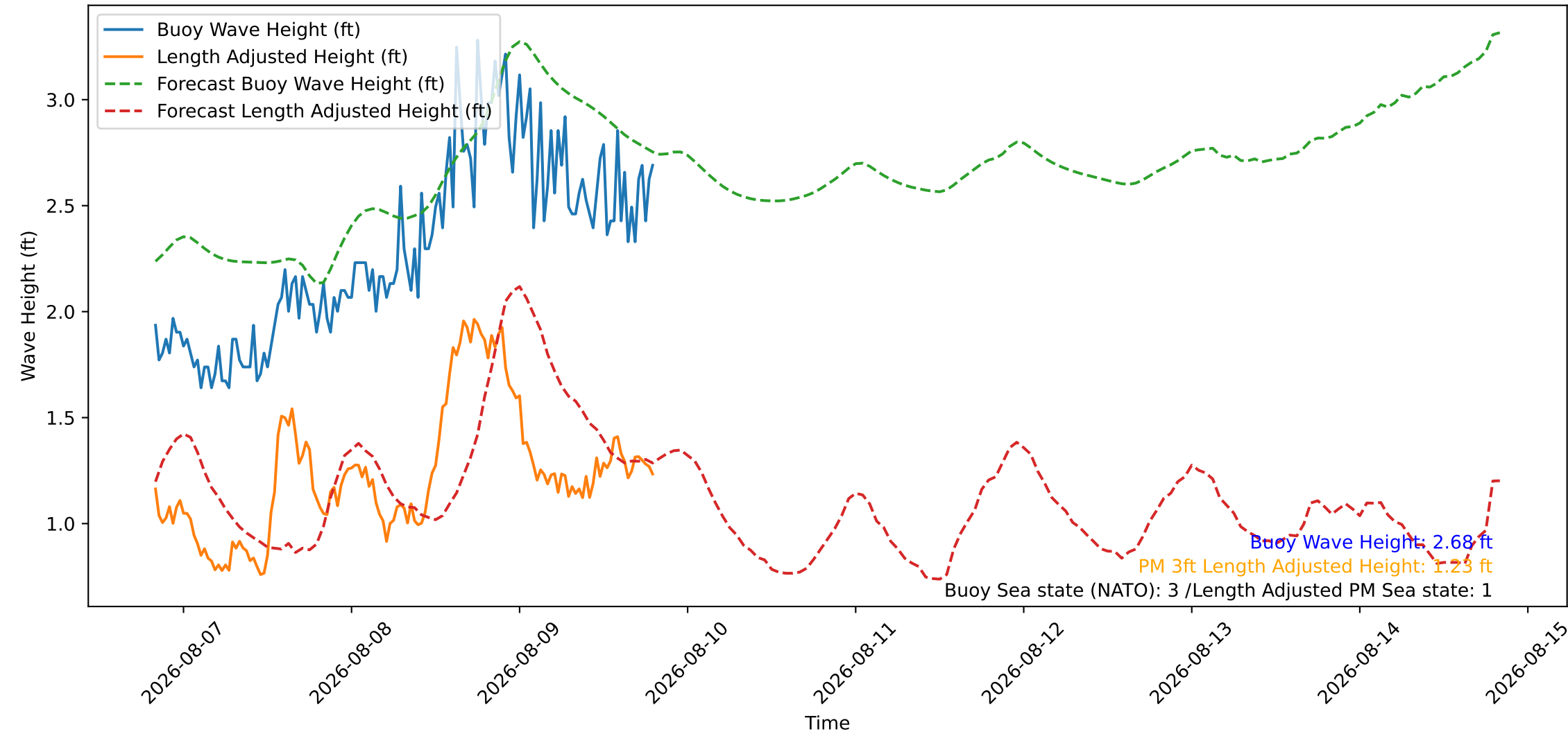
Wave Heights over Time for Oceanside Harbor at 2026-08-09 19:50:27
