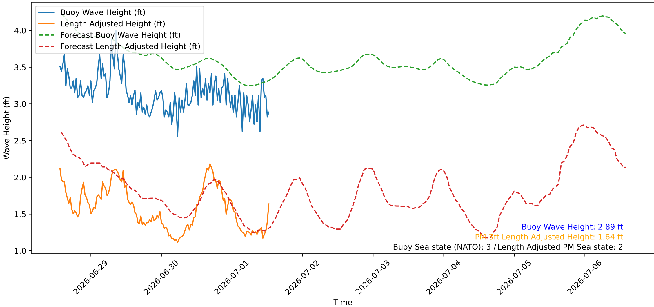
Wave Heights over Time for Oceanside Harbor at 2026-07-01 13:30:26
