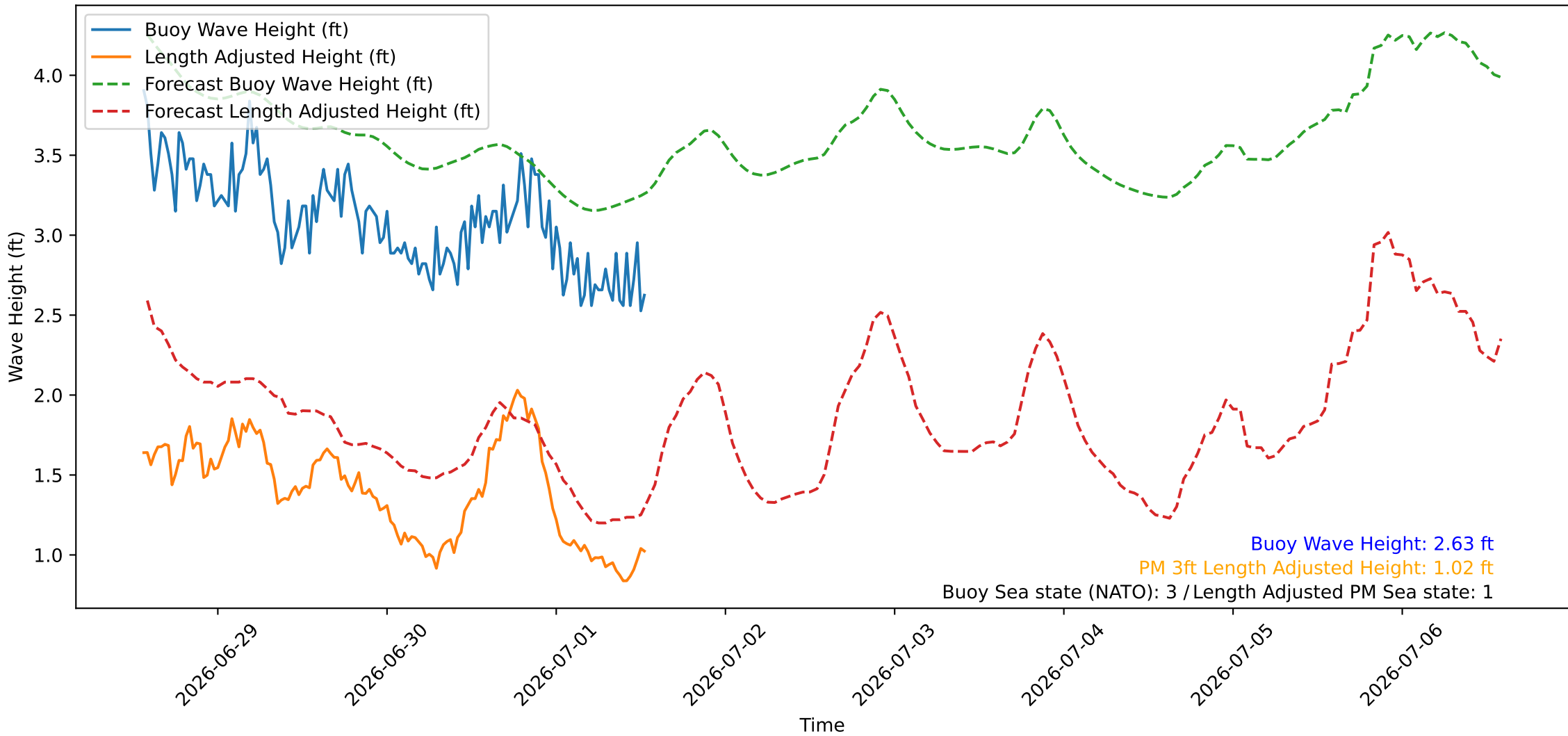
Wave Heights over Time for Green Beach at 2026-07-01 13:31:06
