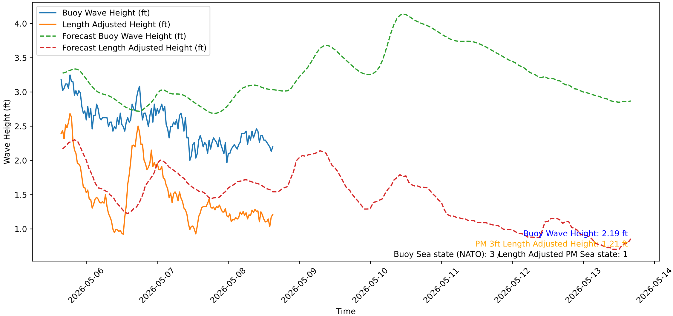
Wave Heights over Time for Oceanside Harbor at 2026-05-08 15:40:31
