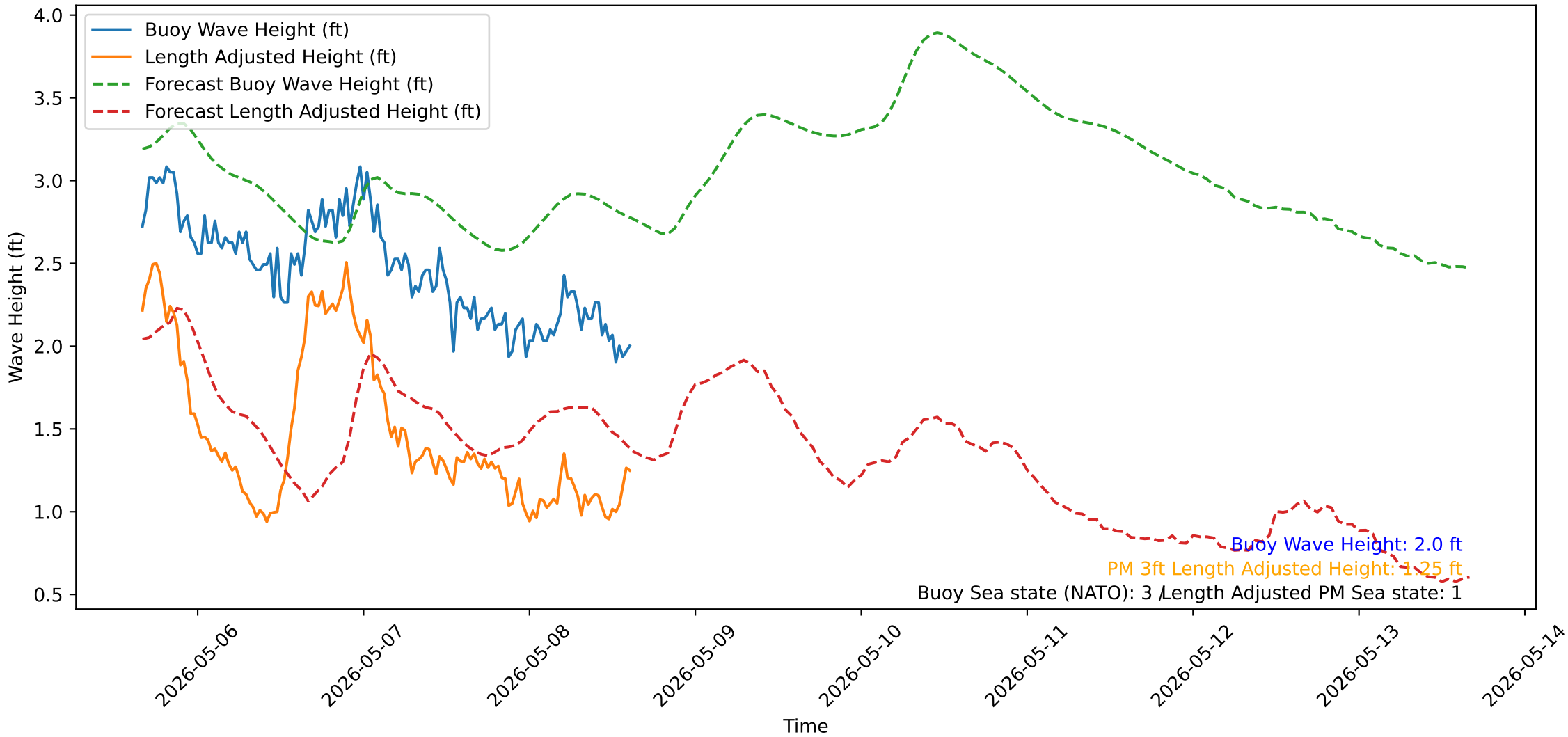
Wave Heights over Time for Red Beach at 2026-05-08 15:40:50
