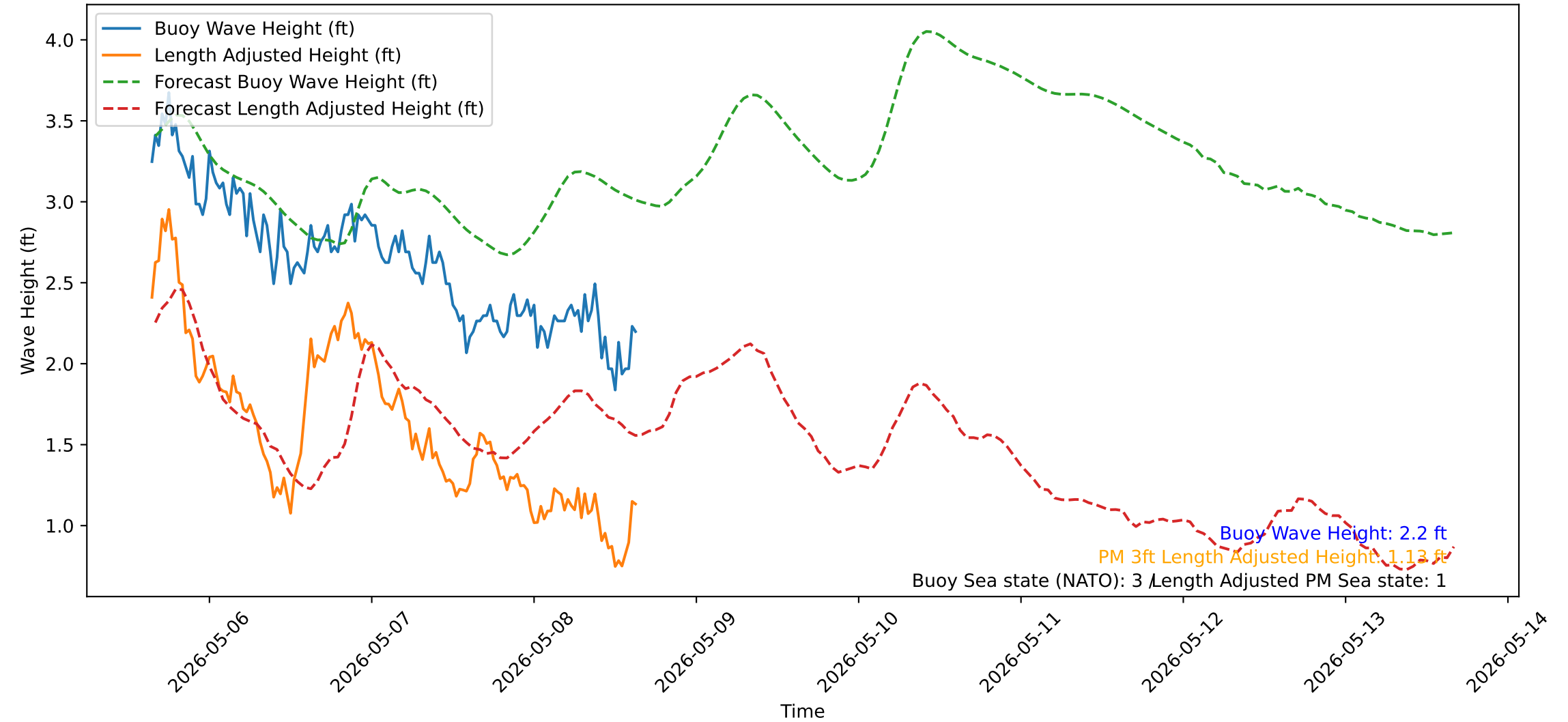
Wave Heights over Time for Green Beach at 2026-05-08 15:41:13
