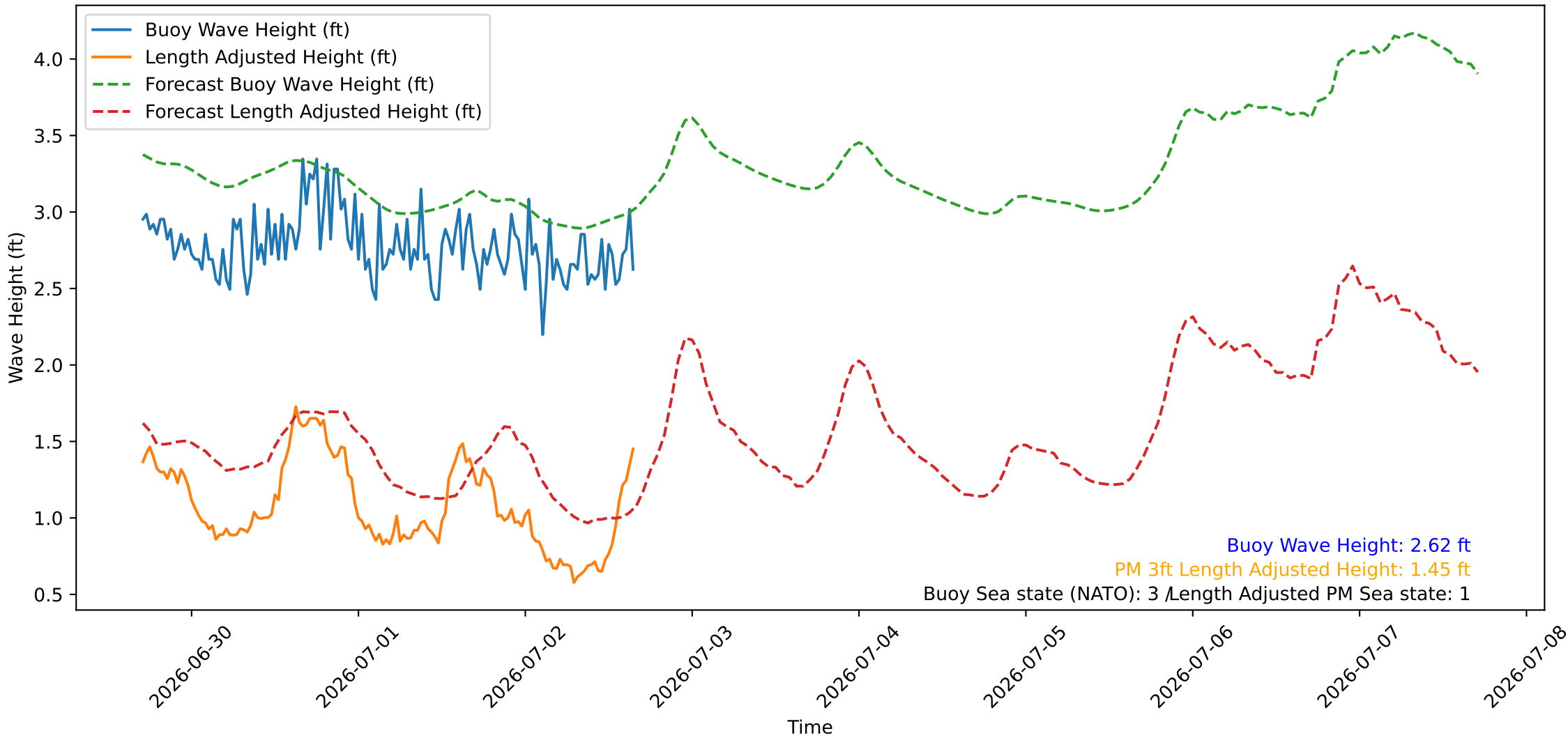
Wave Heights over Time for Red Beach at 2026-07-02 16:40:45
