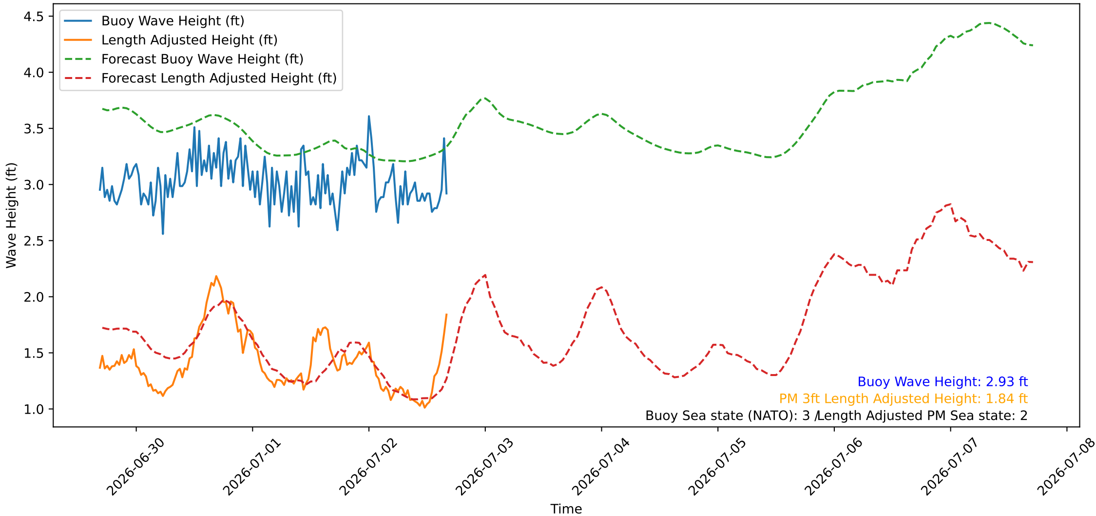
Wave Heights over Time for Oceanside Harbor at 2026-07-02 16:40:26
