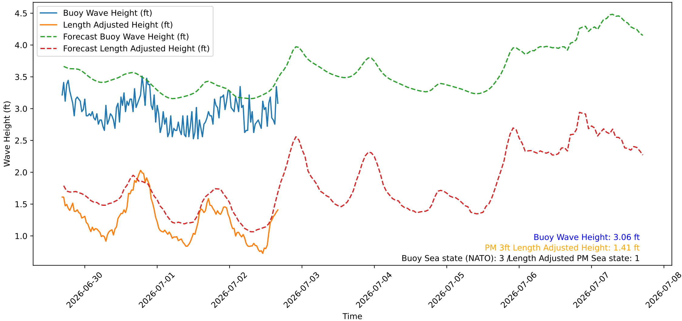
Wave Heights over Time for Green Beach at 2026-07-02 16:41:08
