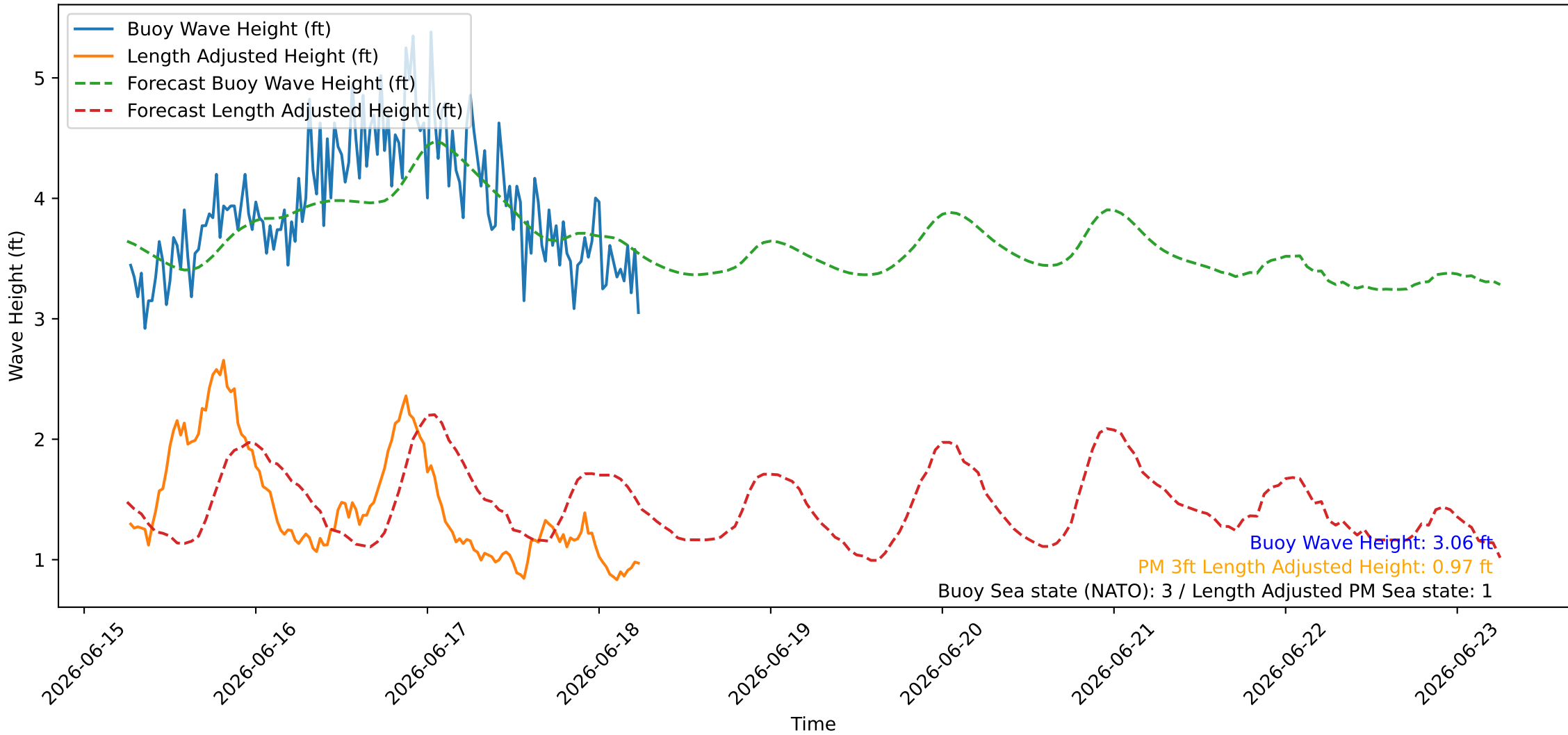
Wave Heights over Time for Red Beach at 2026-06-18 06:20:47
