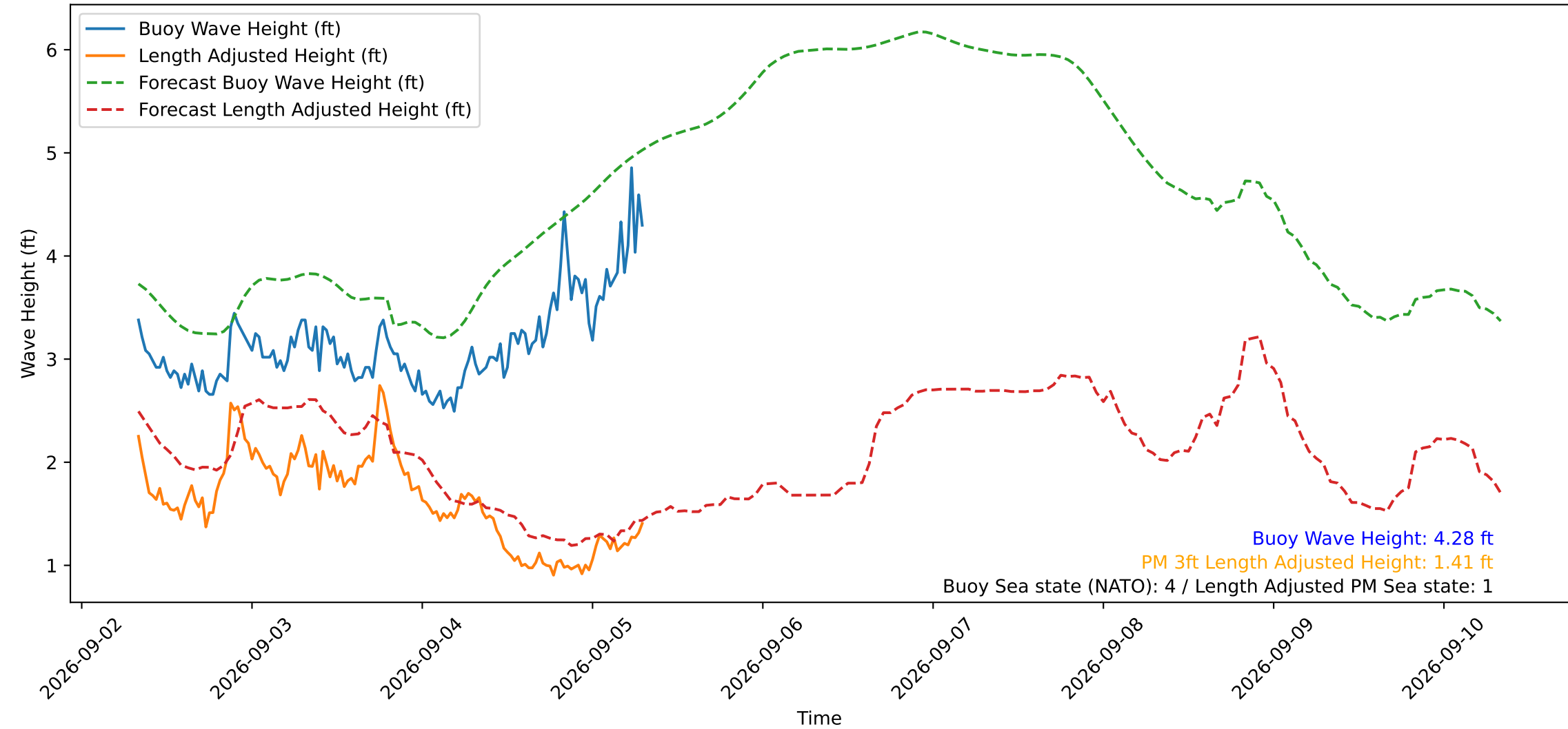
Wave Heights over Time for Green Beach at 2026-09-05 07:51:14
