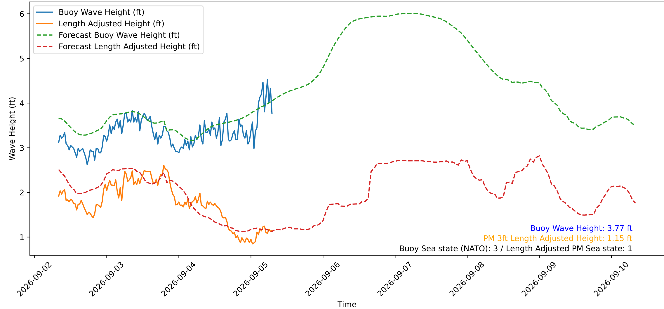
Wave Heights over Time for Oceanside Harbor at 2026-09-05 07:50:29
