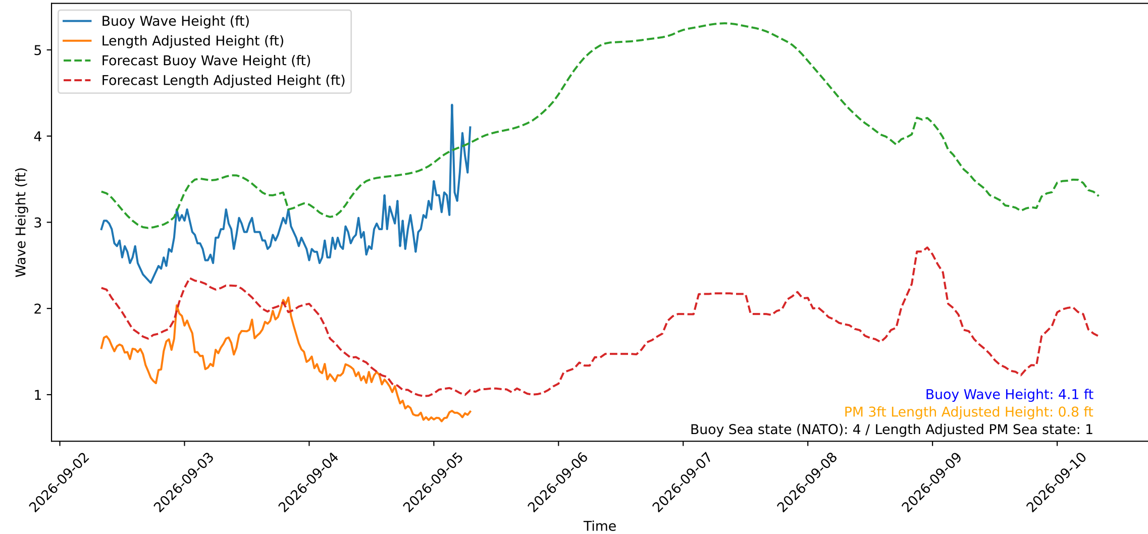
Wave Heights over Time for Red Beach at 2026-09-05 07:50:50
