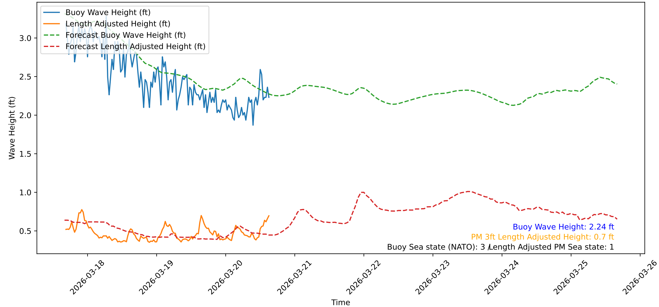
Wave Heights over Time for Red Beach at 2026-03-20 16:00:47
