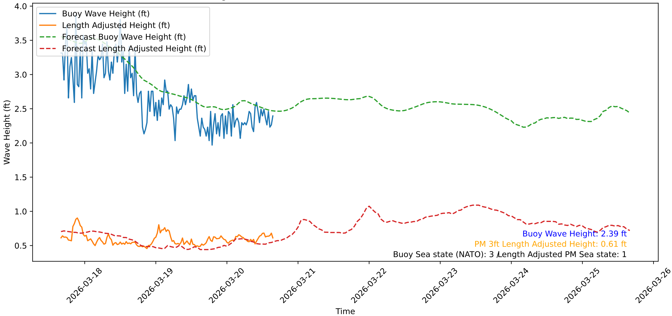
Wave Heights over Time for Oceanside Harbor at 2026-03-20 16:00:31
