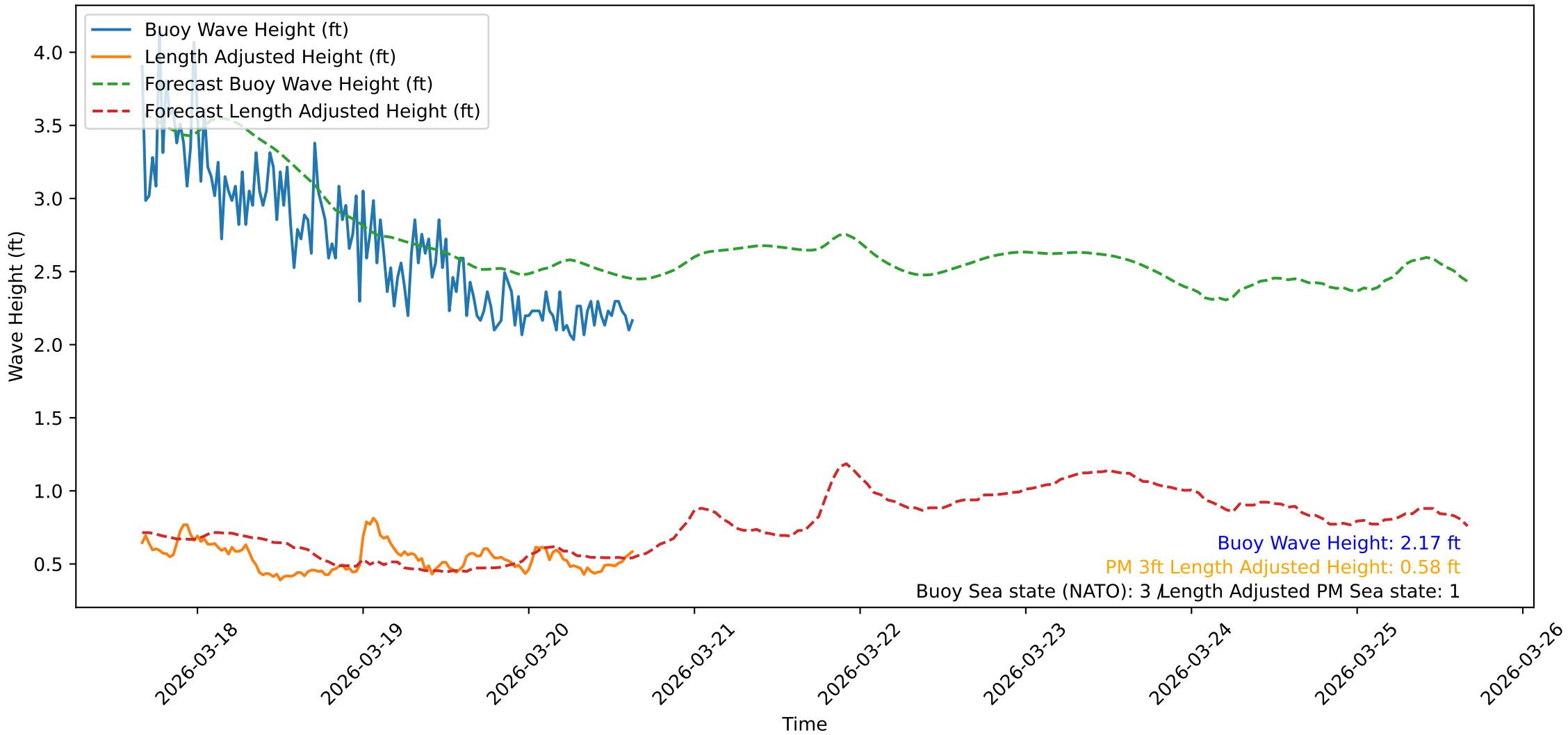
Wave Heights over Time for Green Beach at 2026-03-20 16:01:09
