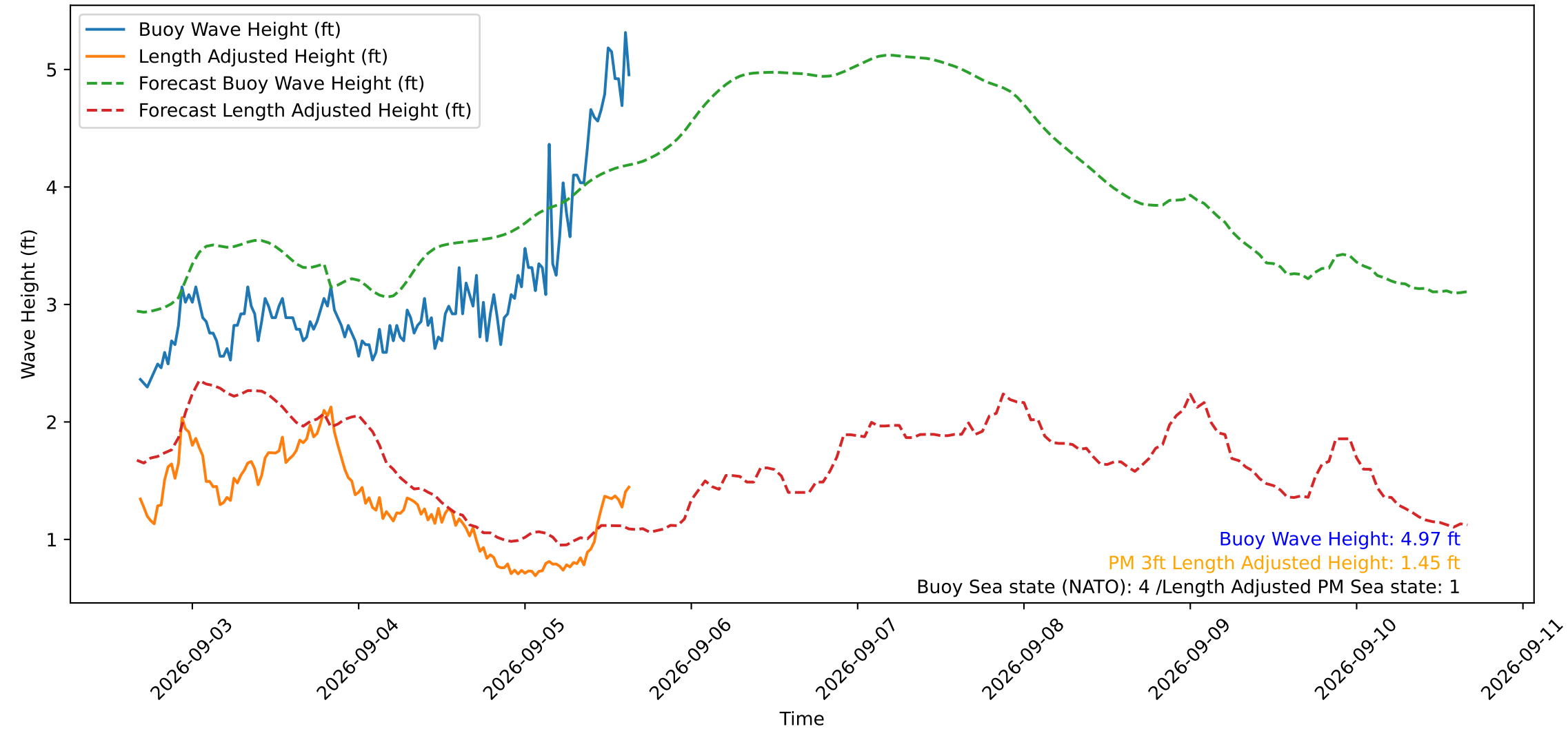
Wave Heights over Time for Red Beach at 2026-09-05 16:10:50
