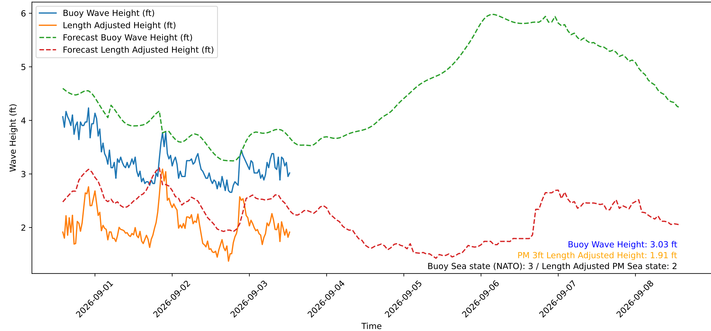
Wave Heights over Time for Green Beach at 2026-09-03 13:31:12
