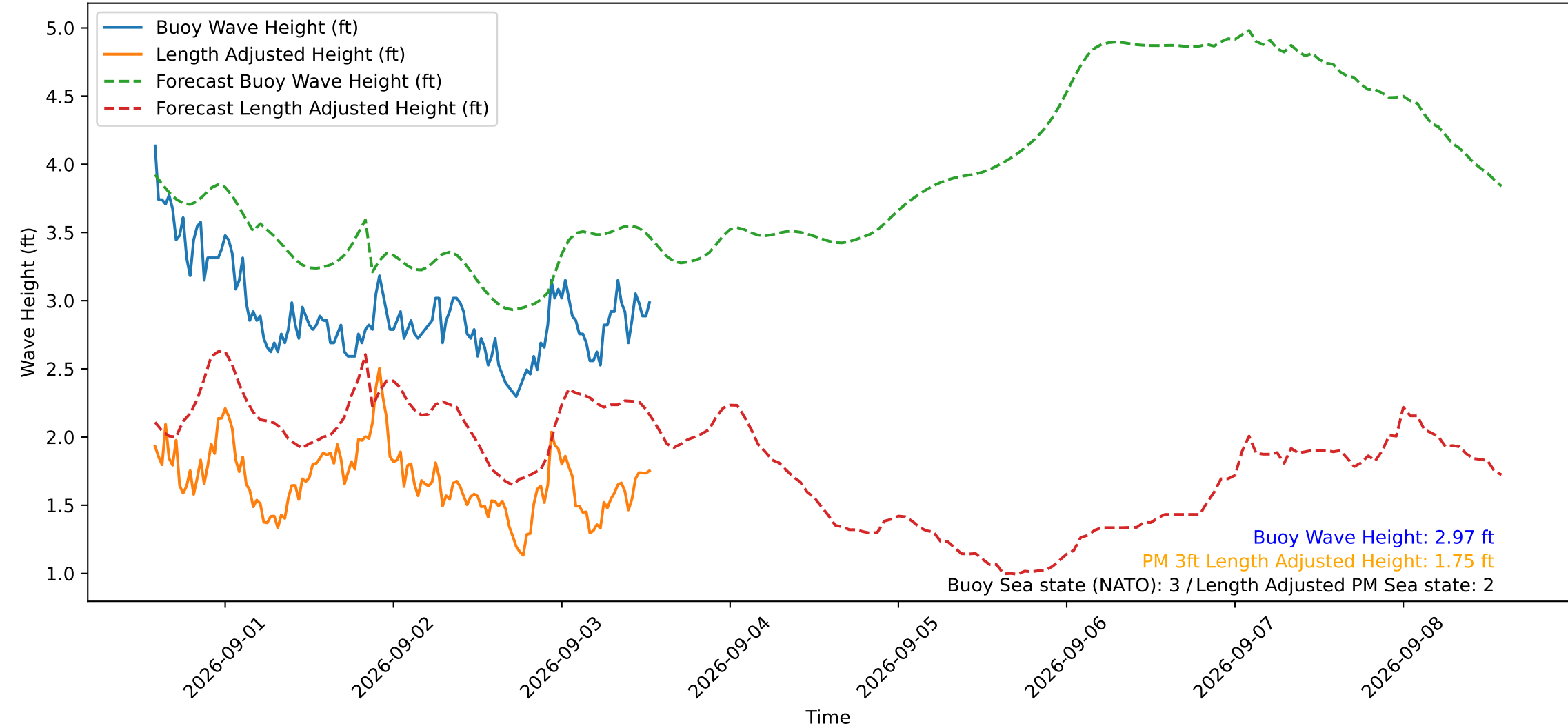
Wave Heights over Time for Red Beach at 2026-09-03 13:30:49
