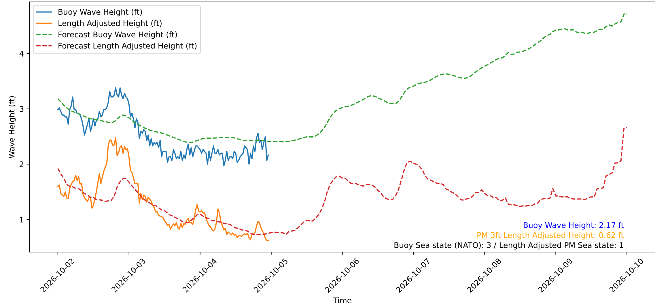
Wave Heights over Time for Green Beach at 2026-10-04 23:41:11
