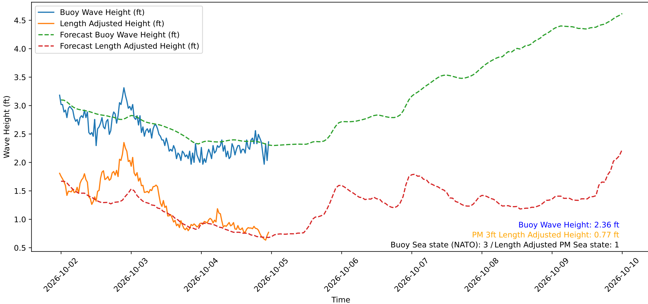
Wave Heights over Time for Oceanside Harbor at 2026-10-04 23:40:29
