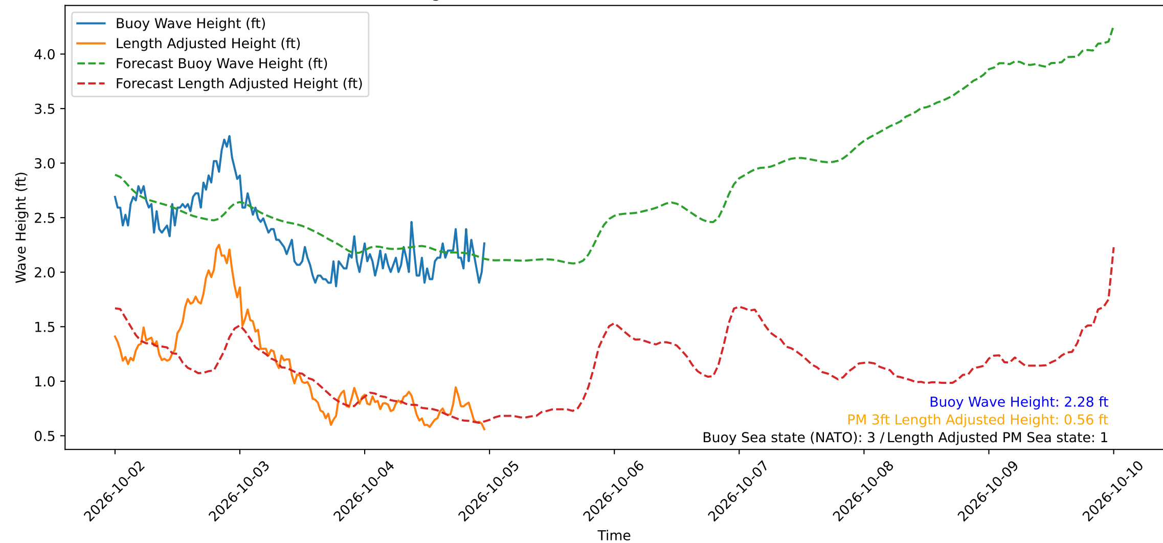
Wave Heights over Time for Red Beach at 2026-10-04 23:40:49
