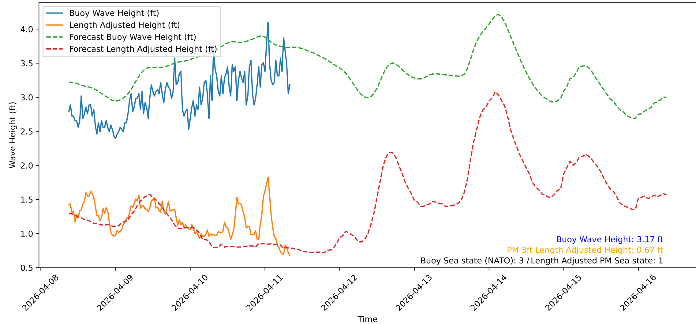
Wave Heights over Time for Red Beach at 2026-04-11 08:50:51
