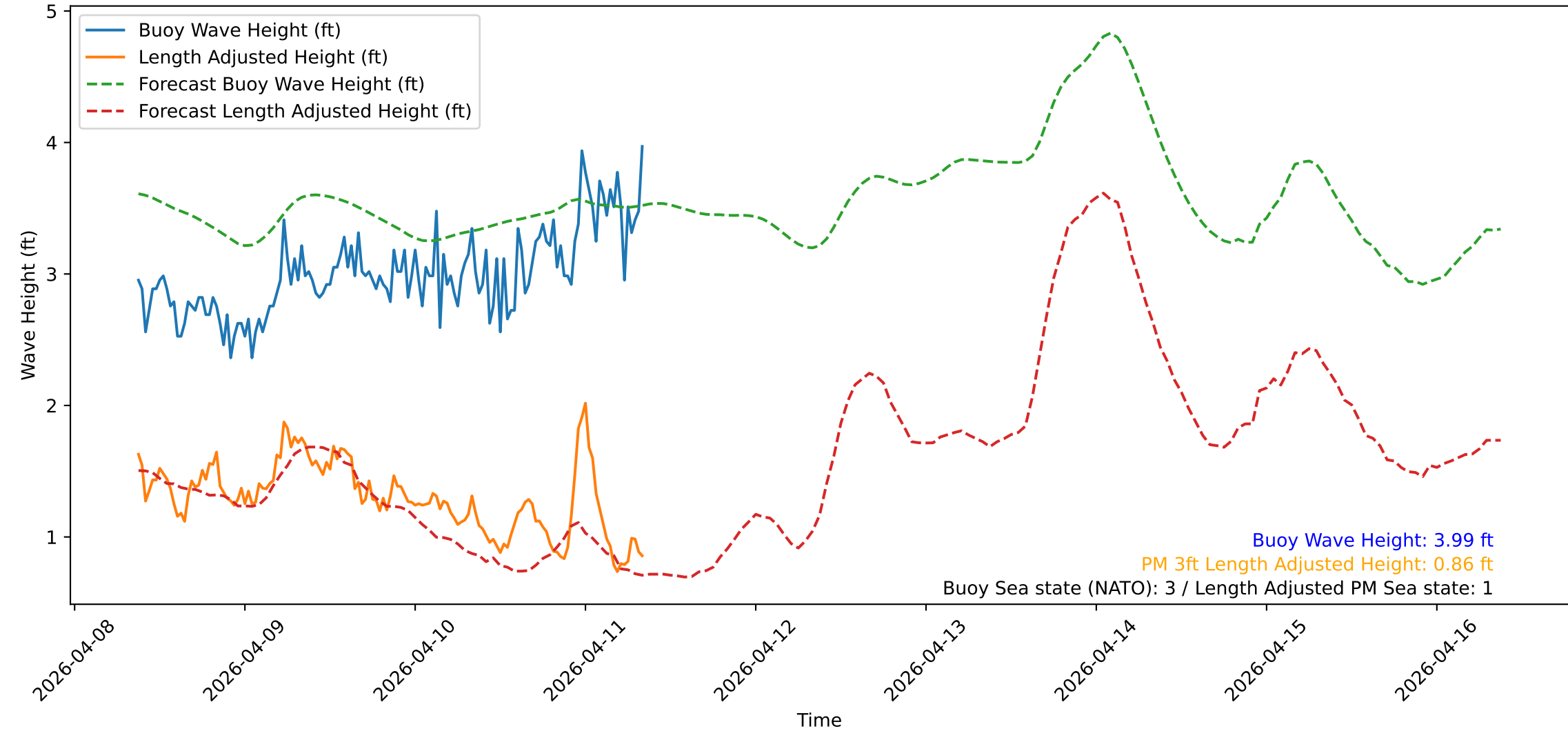
Wave Heights over Time for Green Beach at 2026-04-11 08:51:14
