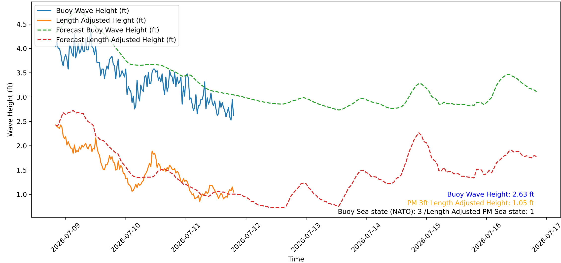
Wave Heights over Time for Green Beach at 2026-07-11 20:01:09
