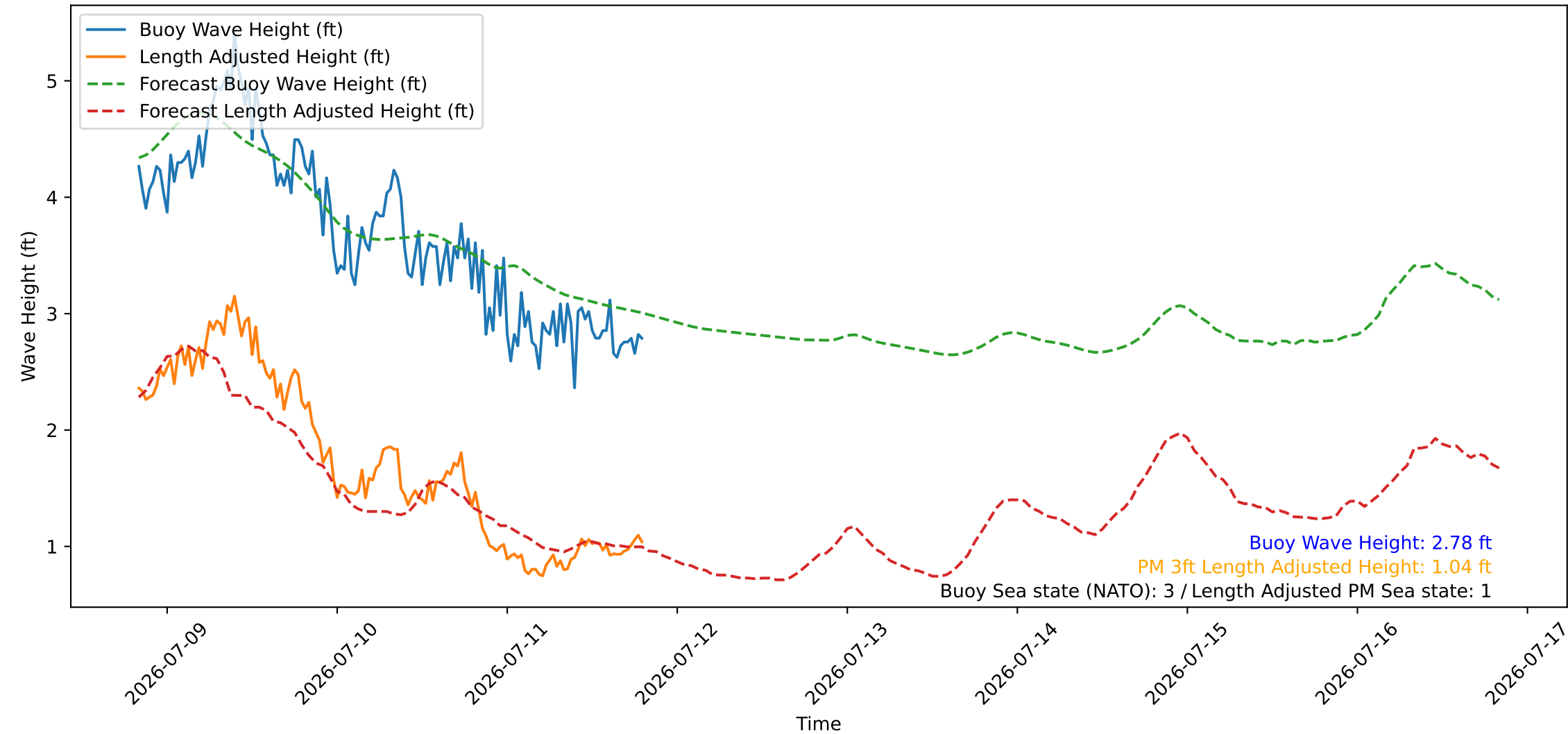
Wave Heights over Time for Oceanside Harbor at 2026-07-11 20:00:26
