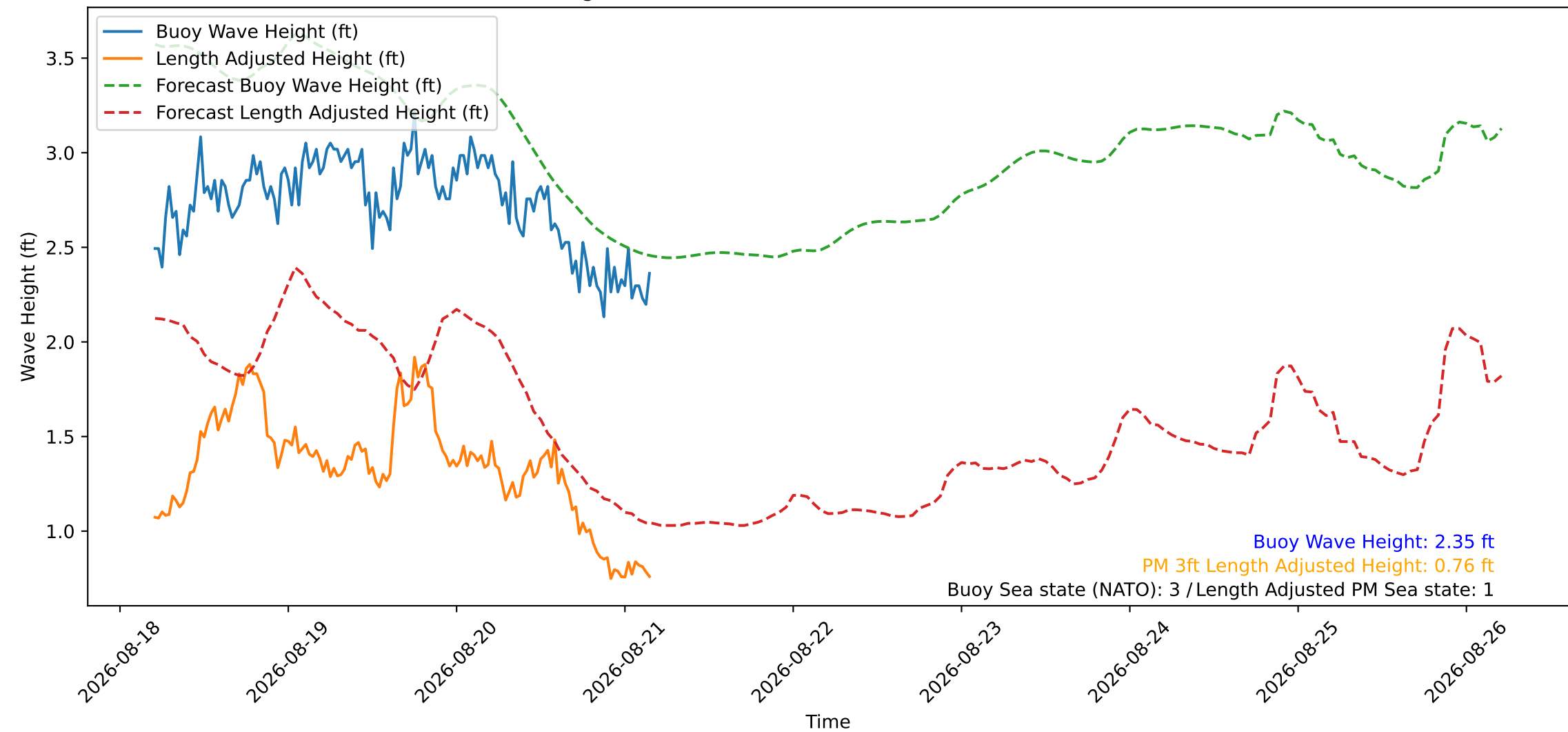
Wave Heights over Time for Red Beach at 2026-08-21 04:30:46
