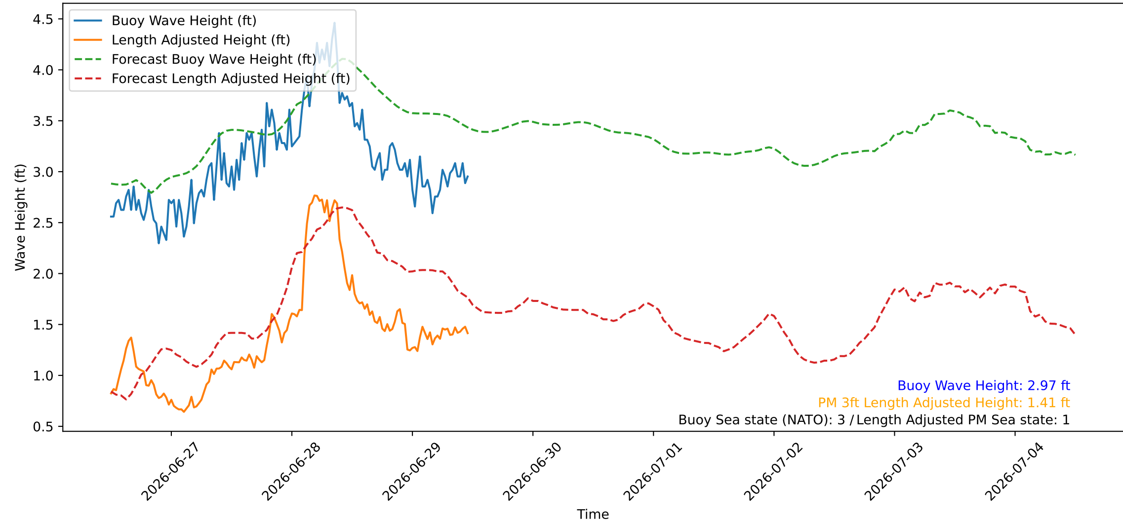
Wave Heights over Time for Red Beach at 2026-06-29 11:50:46
