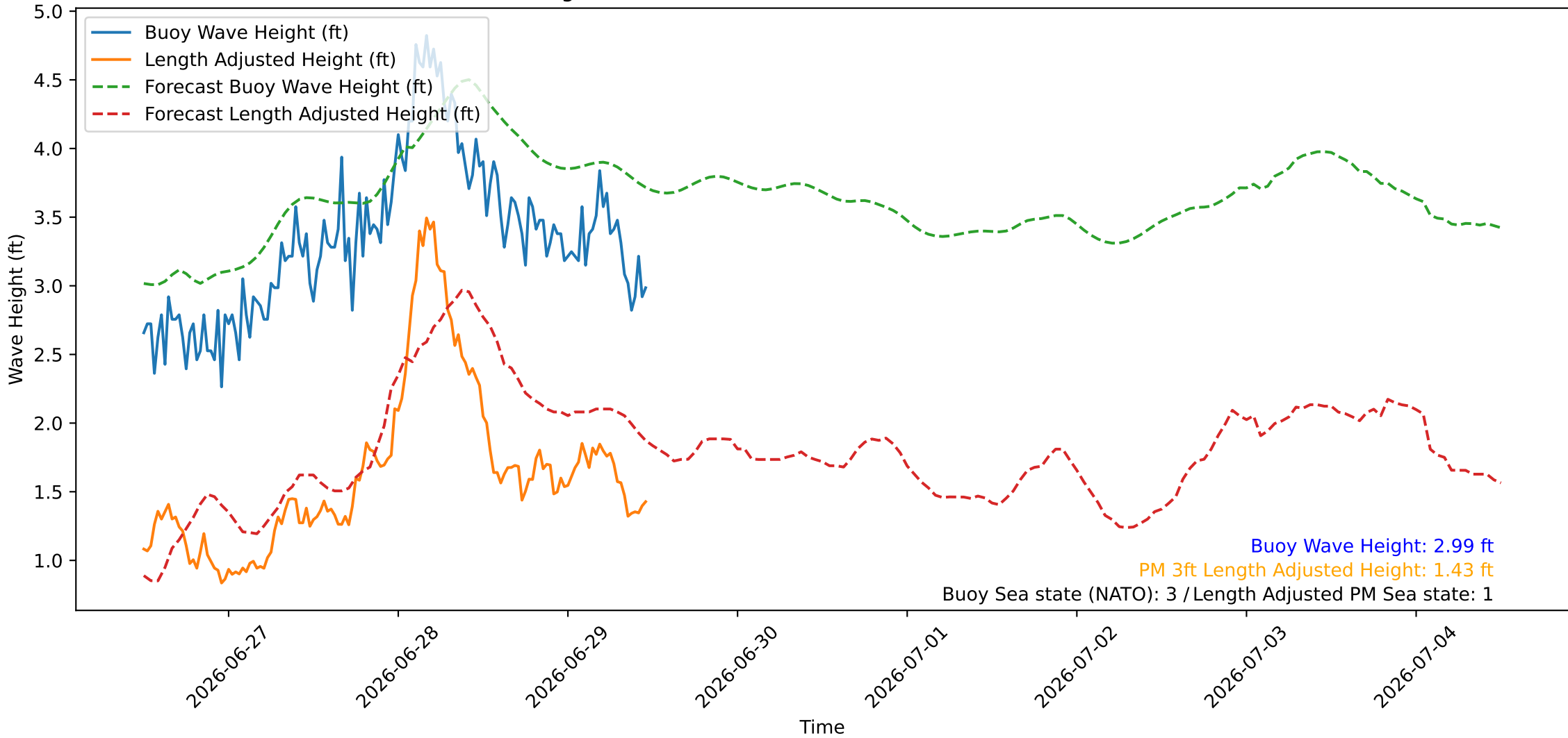
Wave Heights over Time for Green Beach at 2026-06-29 11:51:08
