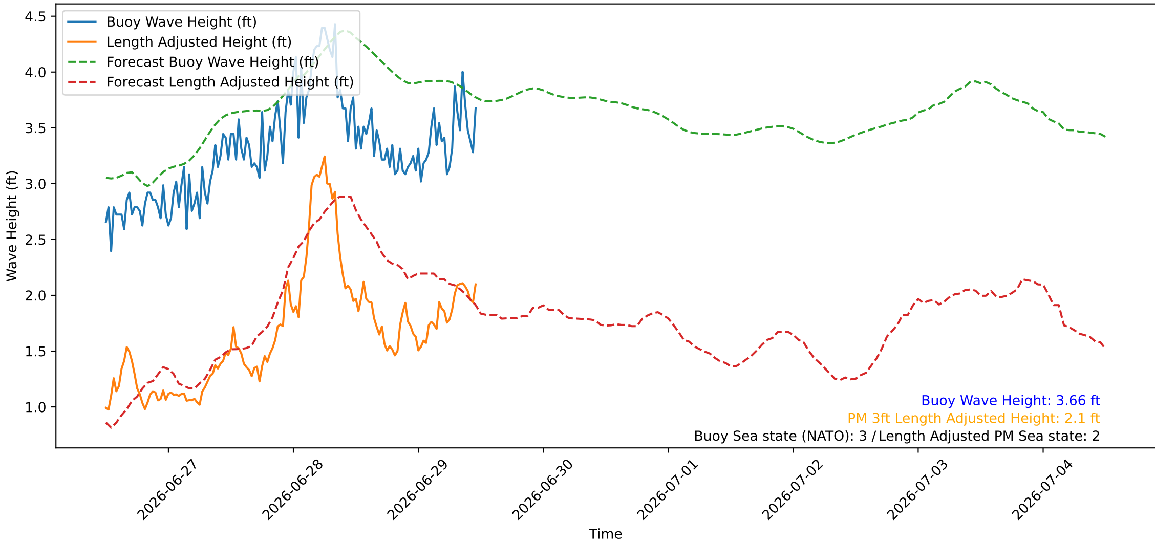
Wave Heights over Time for Oceanside Harbor at 2026-06-29 11:50:25
