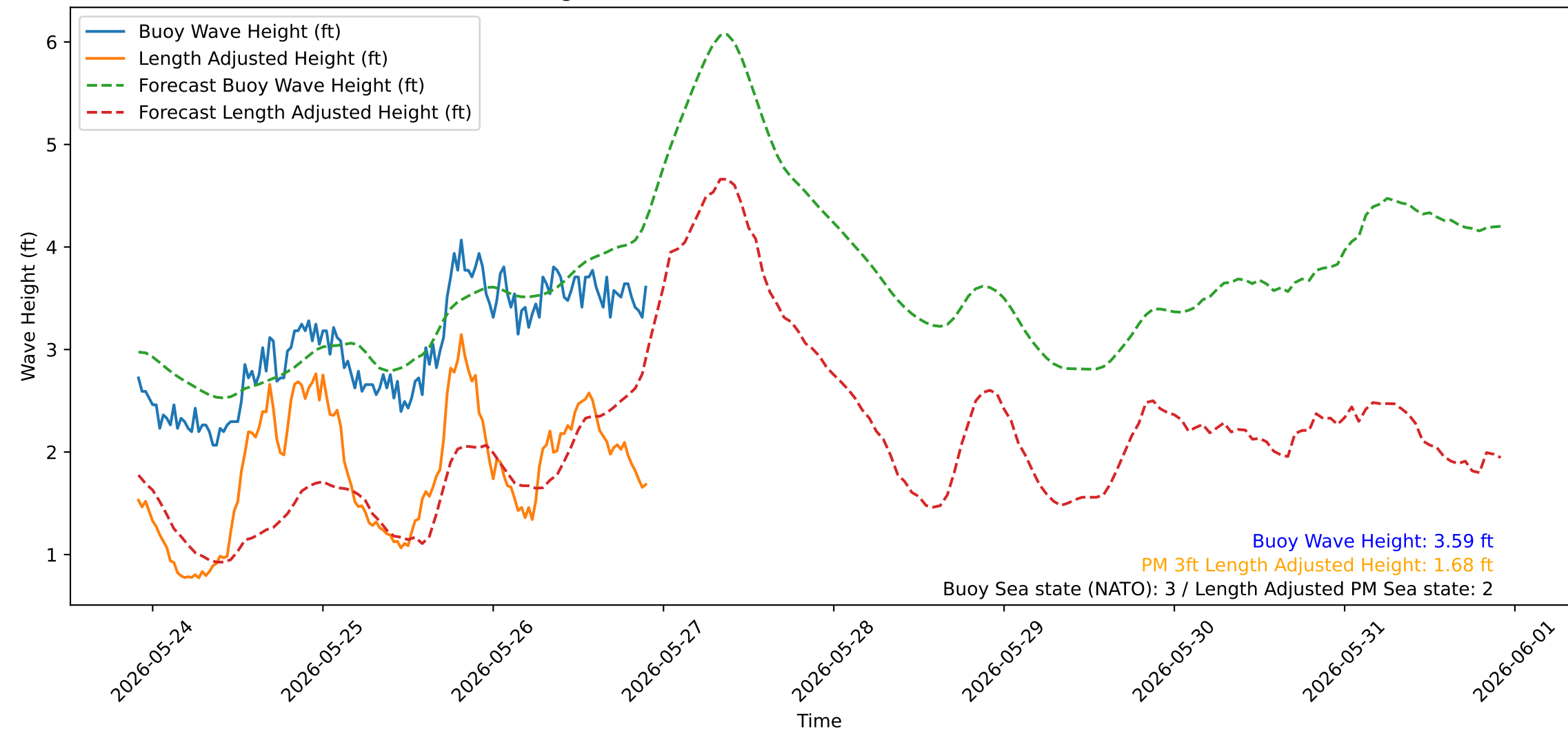
Wave Heights over Time for Green Beach at 2026-05-26 22:11:08
