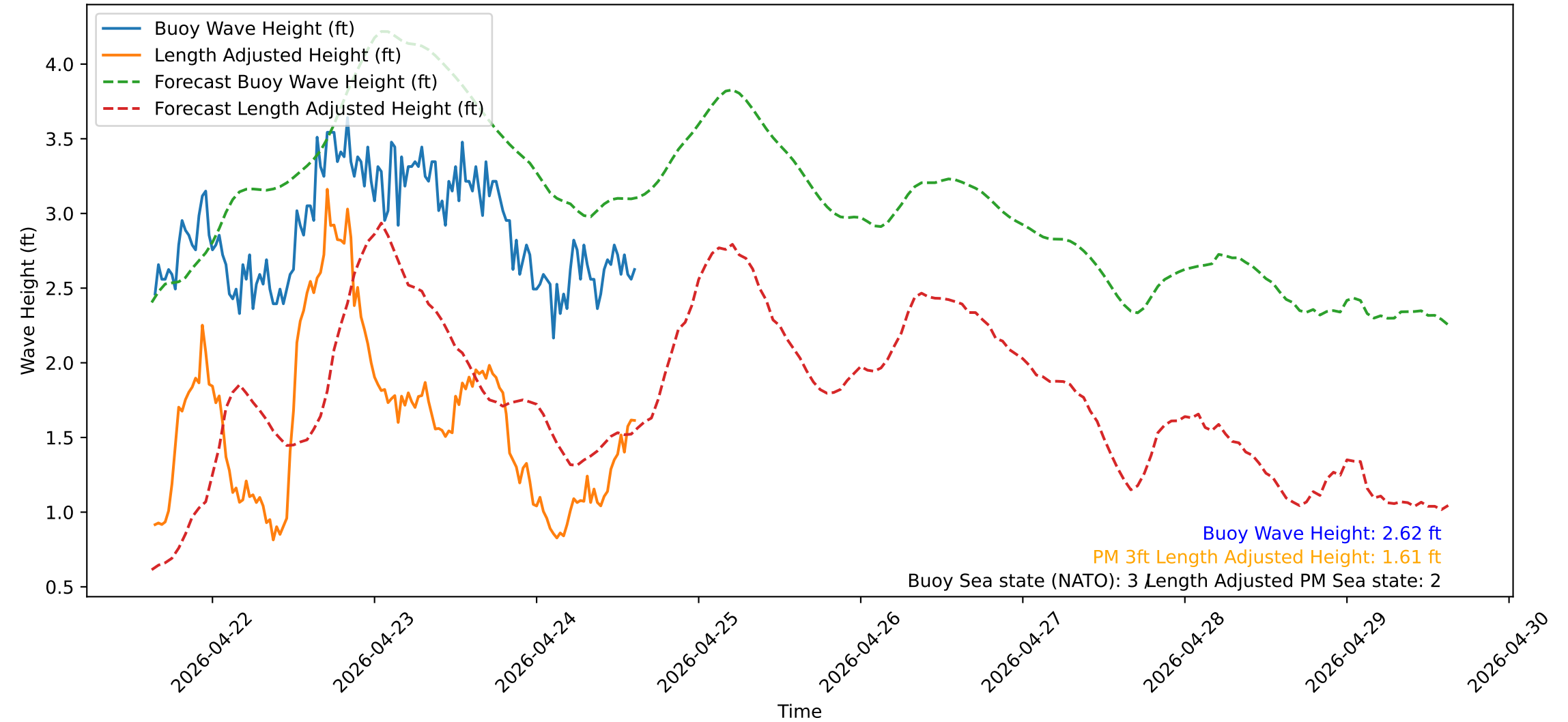
Wave Heights over Time for Red Beach at 2026-04-24 15:20:52
