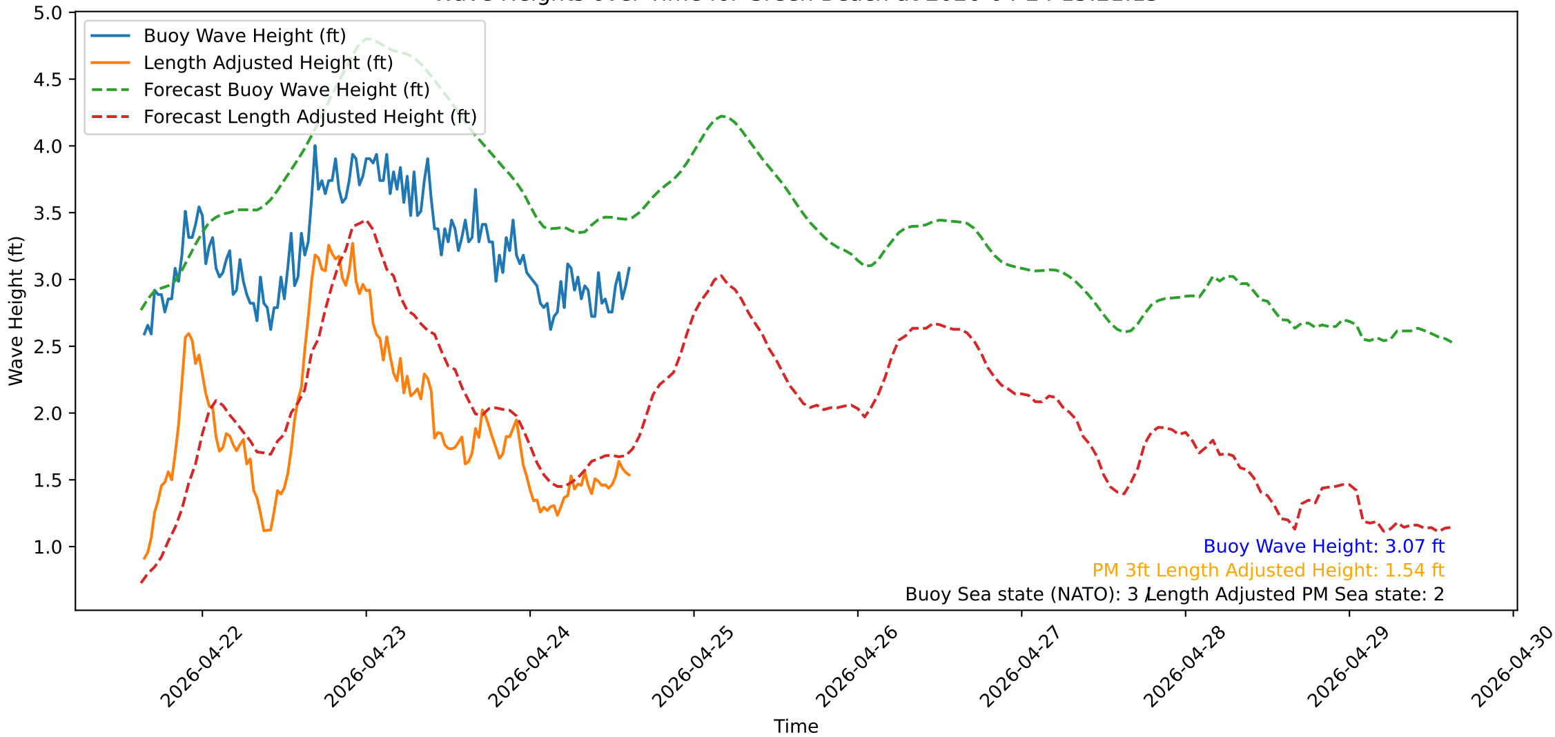
Wave Heights over Time for Green Beach at 2026-04-24 15:21:15
