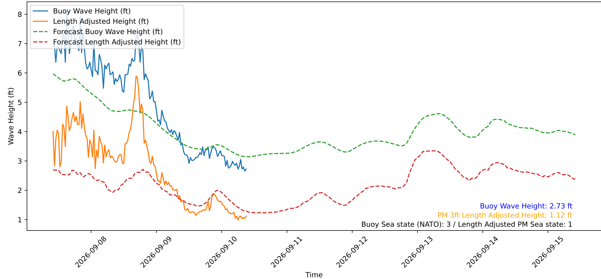
Wave Heights over Time for Green Beach at 2026-09-10 09:51:13
