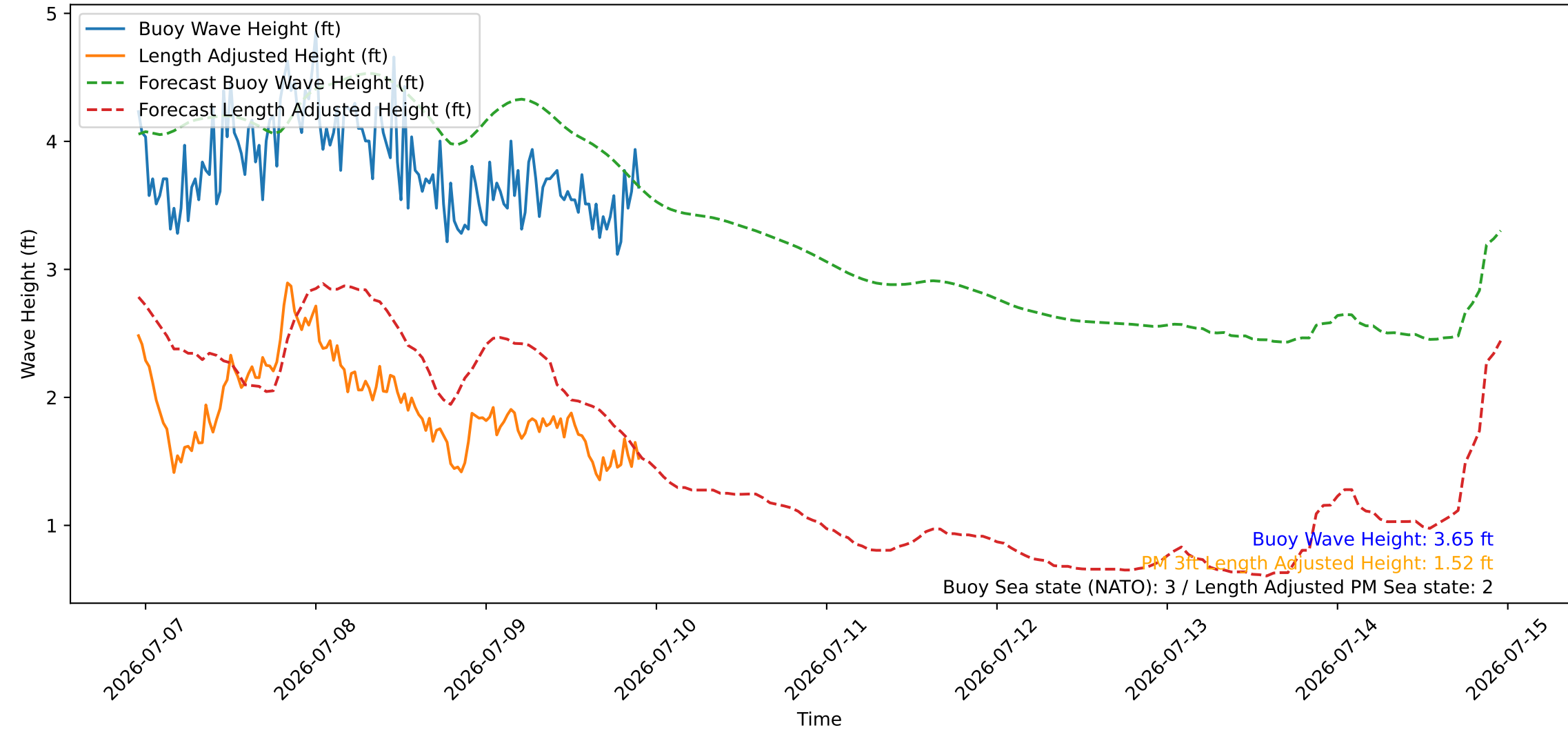
Wave Heights over Time for Red Beach at 2026-07-09 22:30:45
