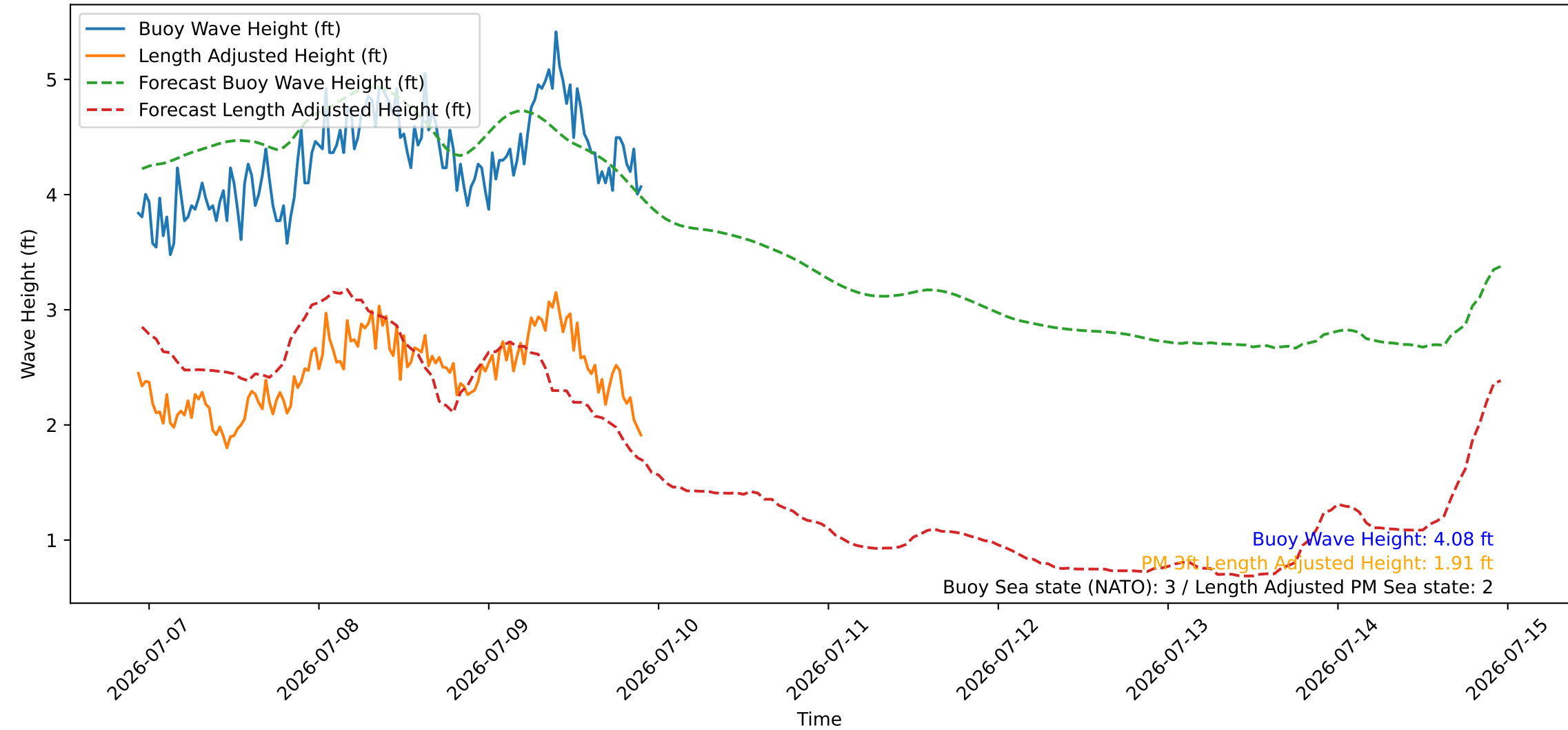
Wave Heights over Time for Oceanside Harbor at 2026-07-09 22:30:26
