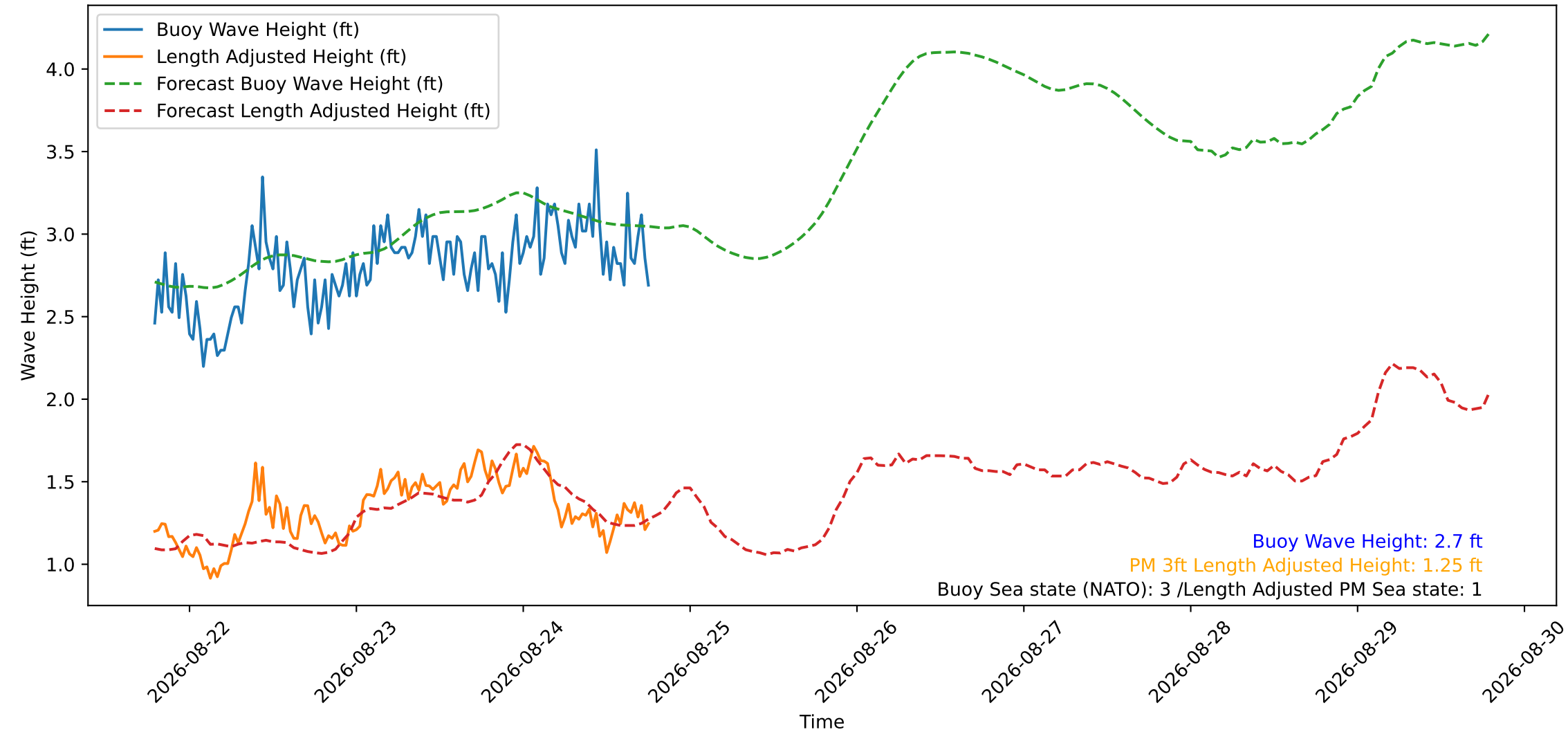
Wave Heights over Time for Oceanside Harbor at 2026-08-24 19:00:29
