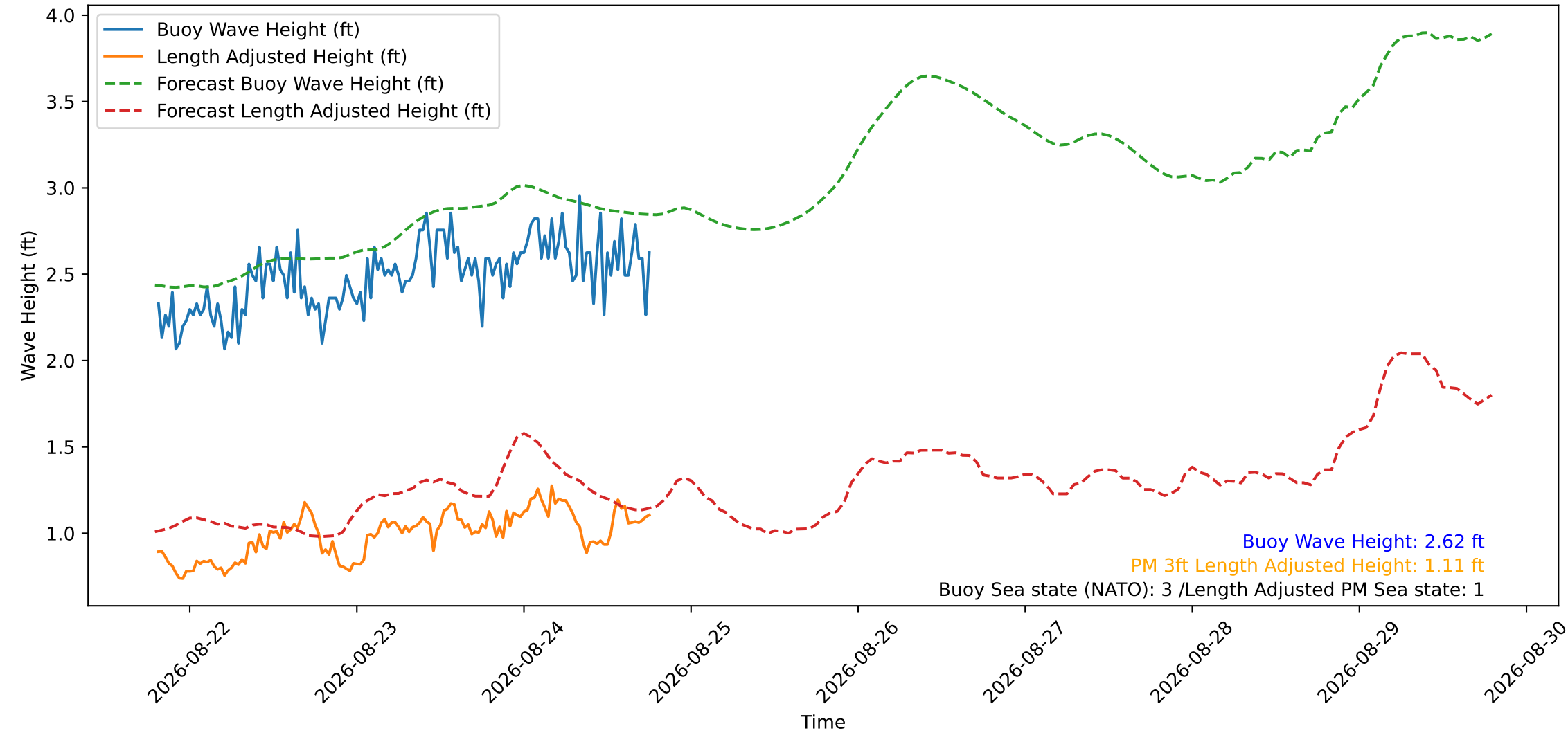
Wave Heights over Time for Red Beach at 2026-08-24 19:00:49
