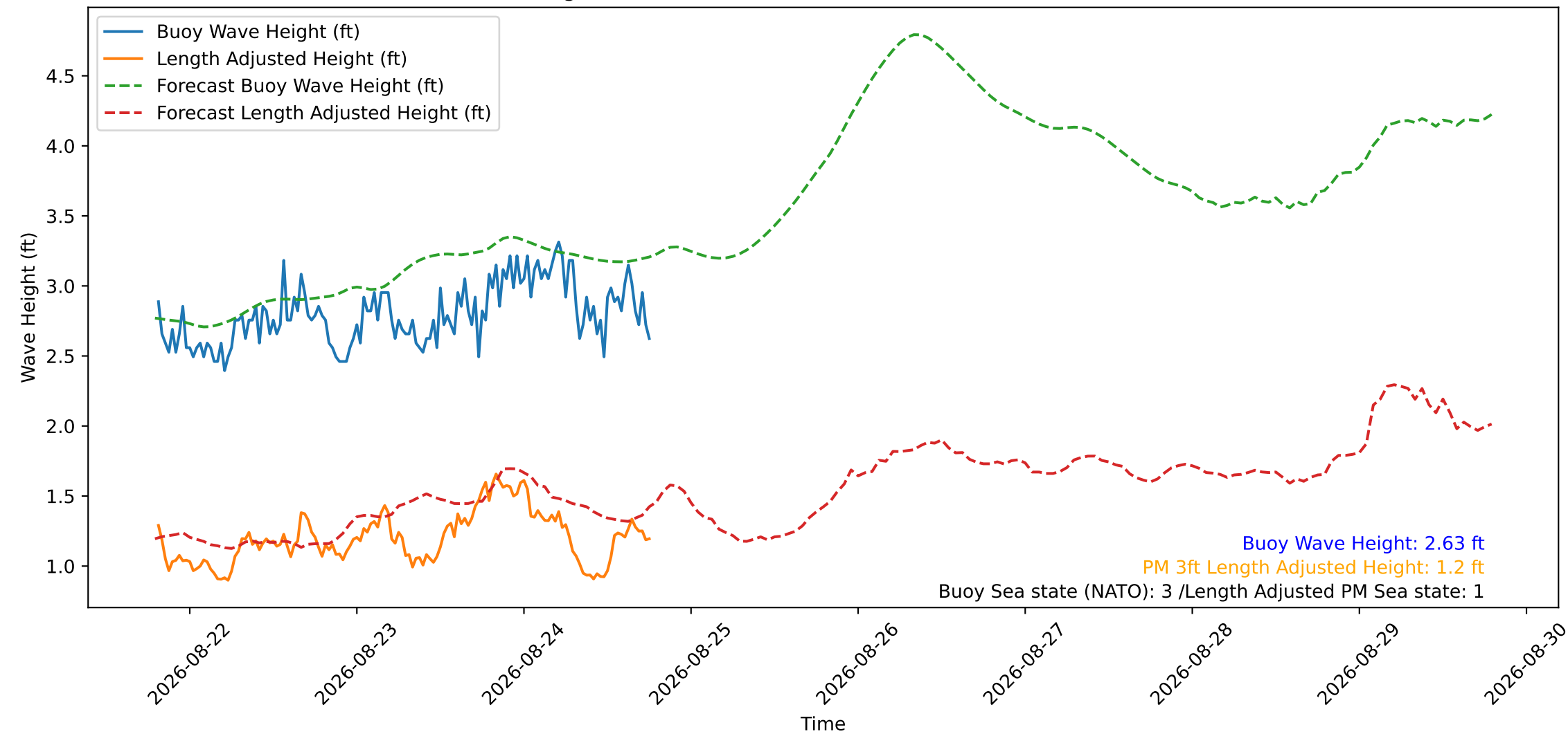
Wave Heights over Time for Green Beach at 2026-08-24 19:01:11
