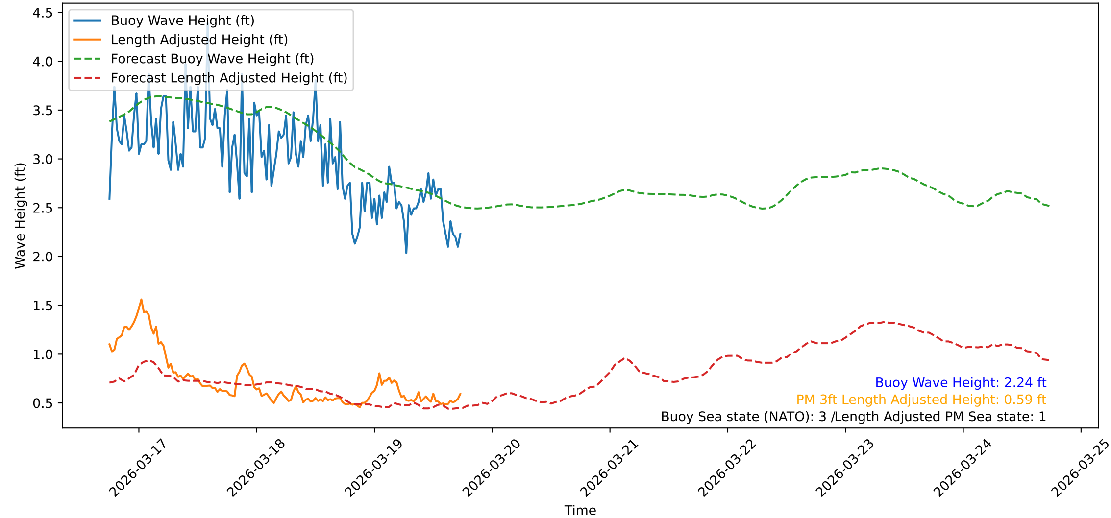
Wave Heights over Time for Oceanside Harbor at 2026-03-19 18:00:31
