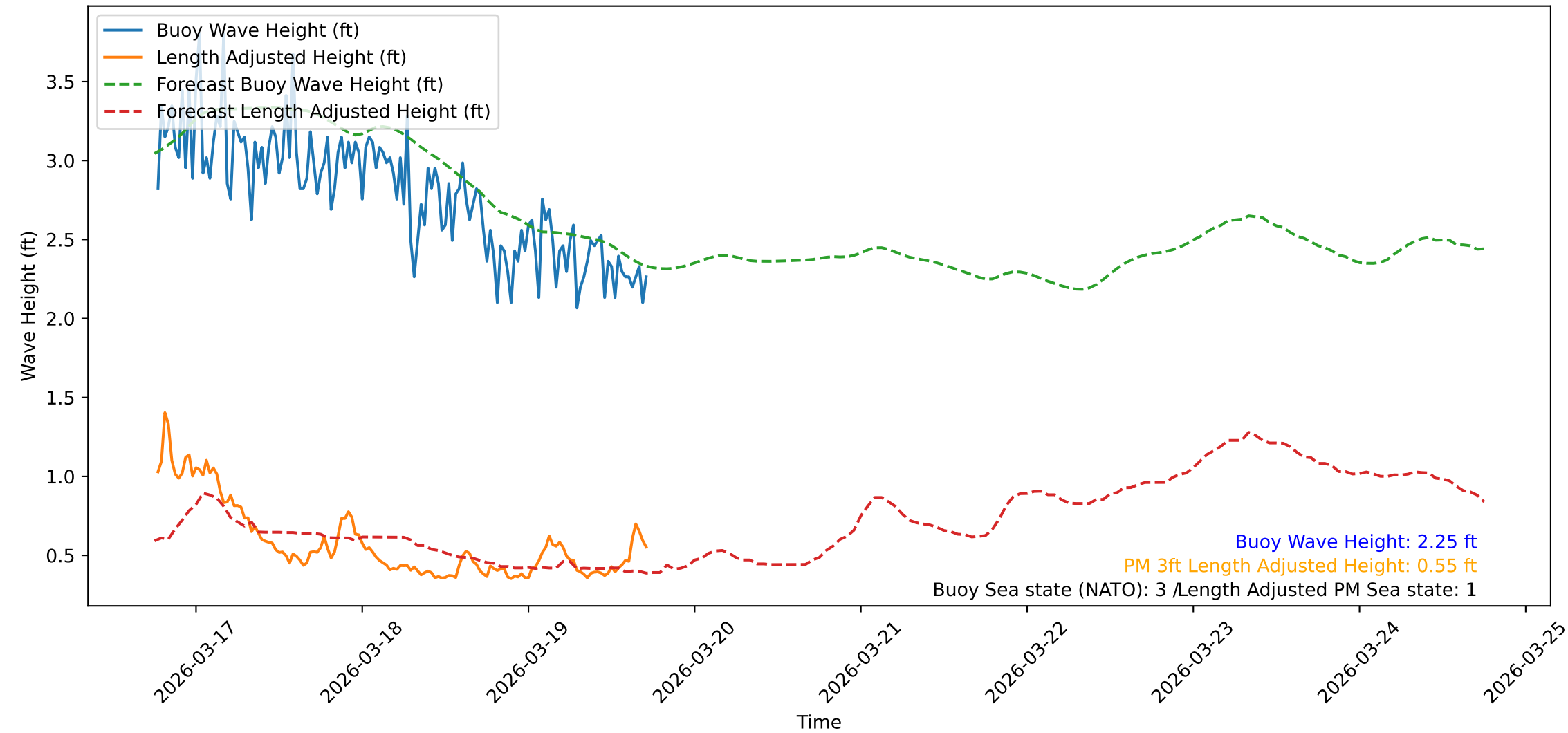
Wave Heights over Time for Red Beach at 2026-03-19 18:00:48
