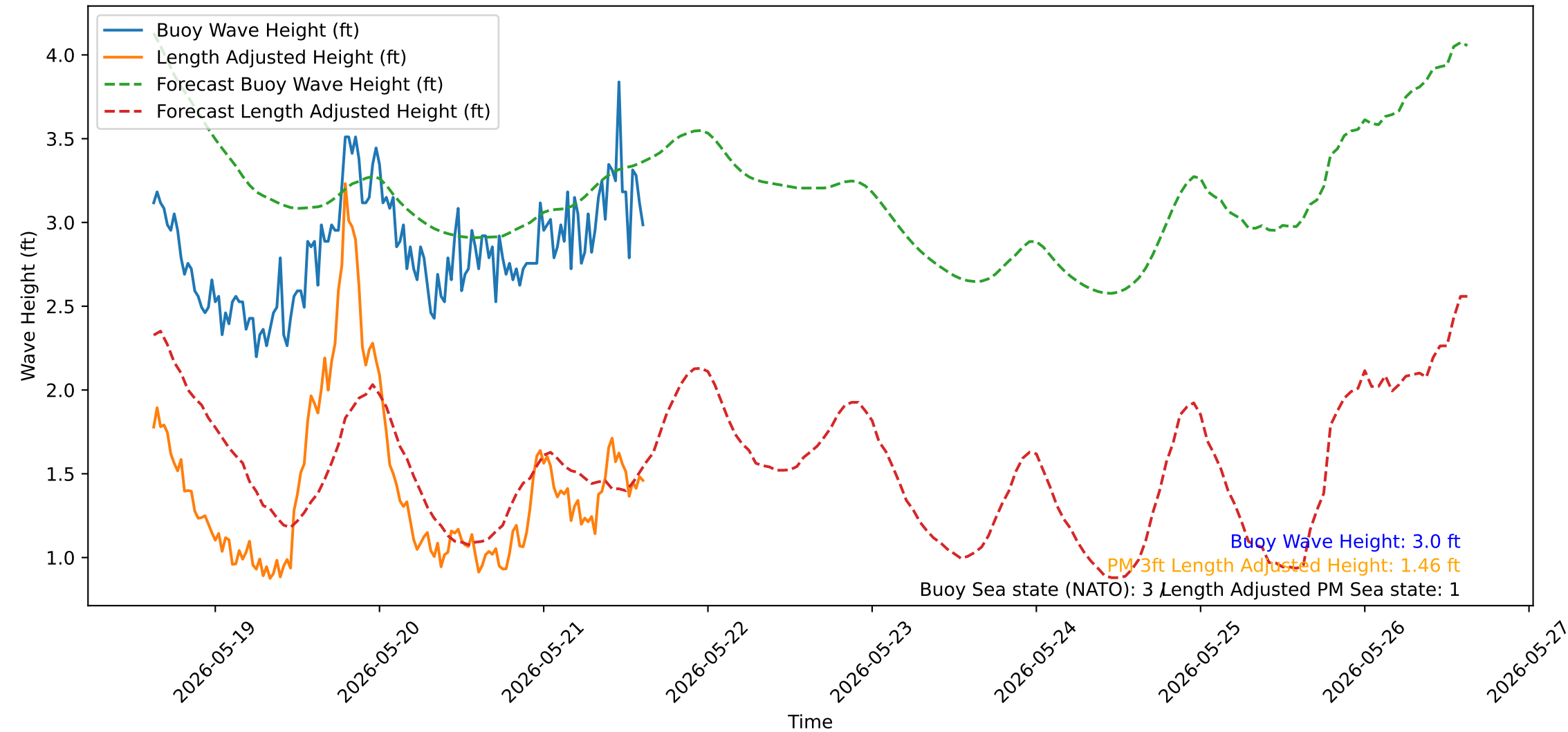
Wave Heights over Time for Oceanside Harbor at 2026-05-21 15:00:31
