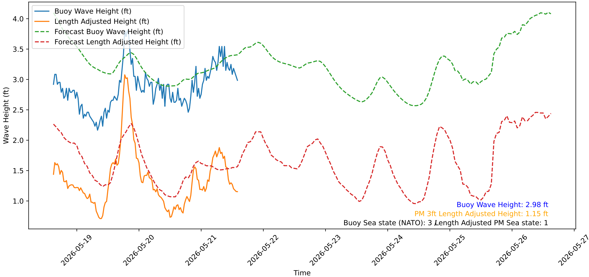
Wave Heights over Time for Green Beach at 2026-05-21 15:01:13
