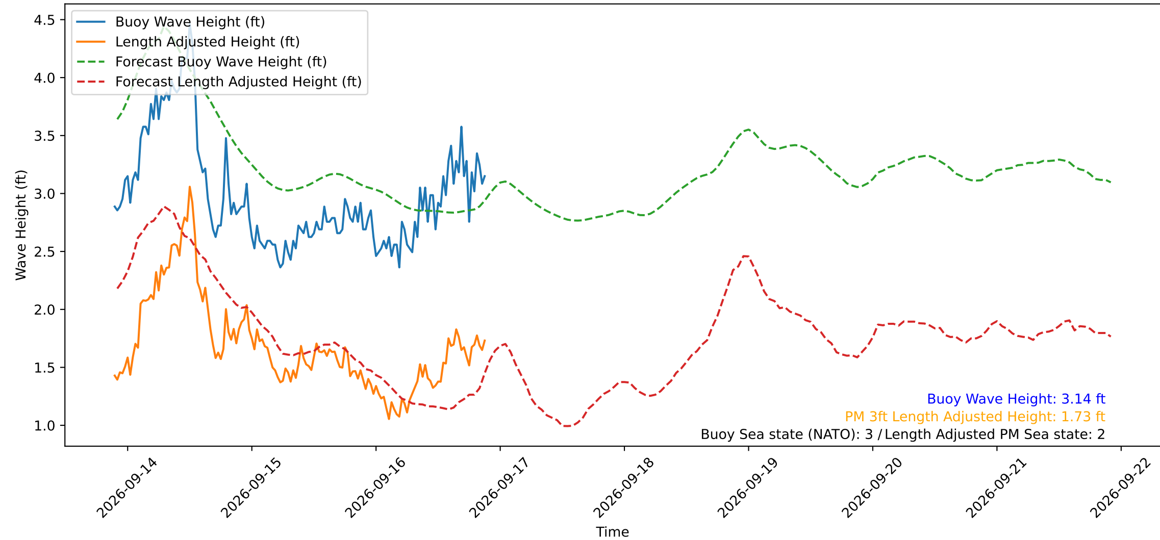
Wave Heights over Time for Oceanside Harbor at 2026-09-16 21:40:30
