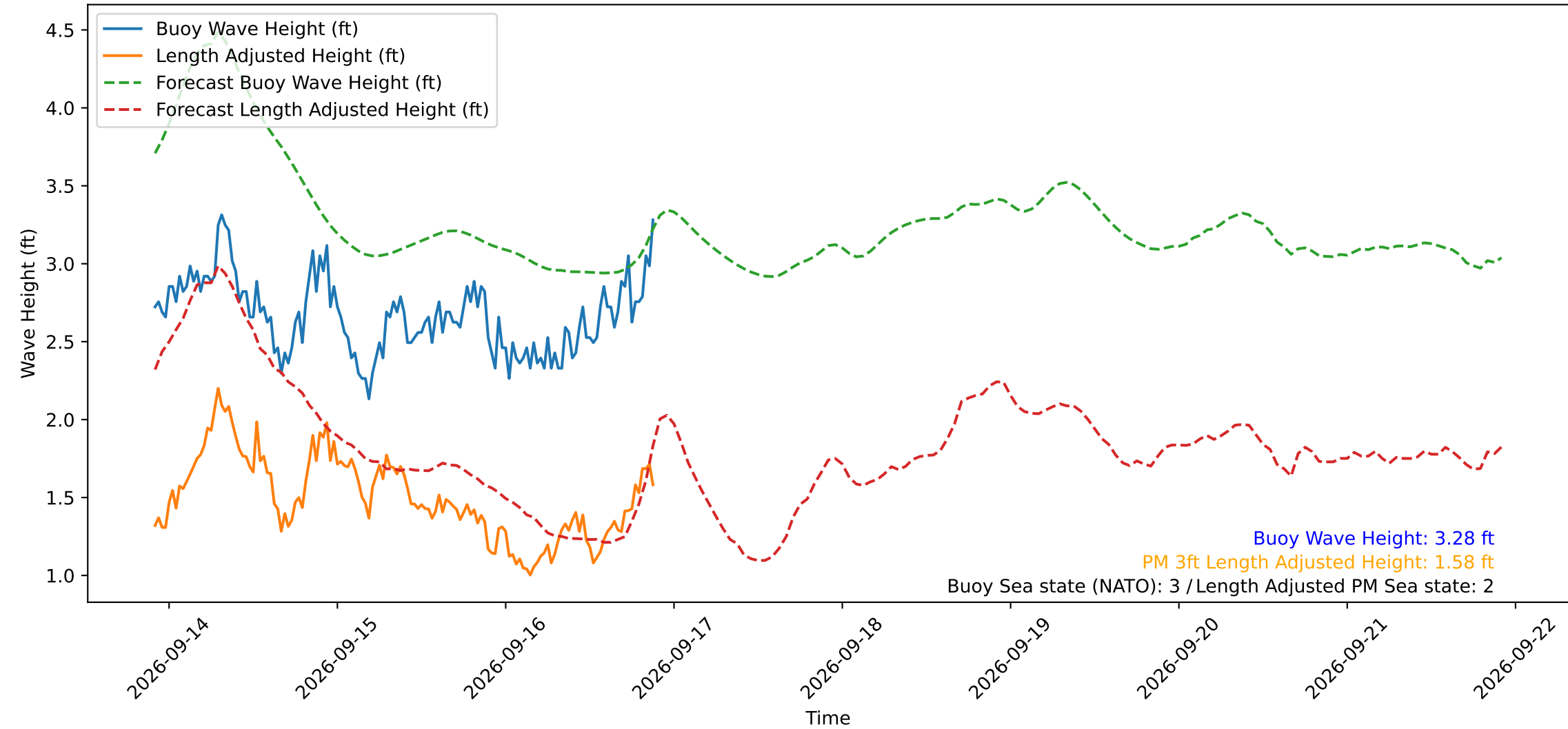
Wave Heights over Time for Green Beach at 2026-09-16 21:41:12
