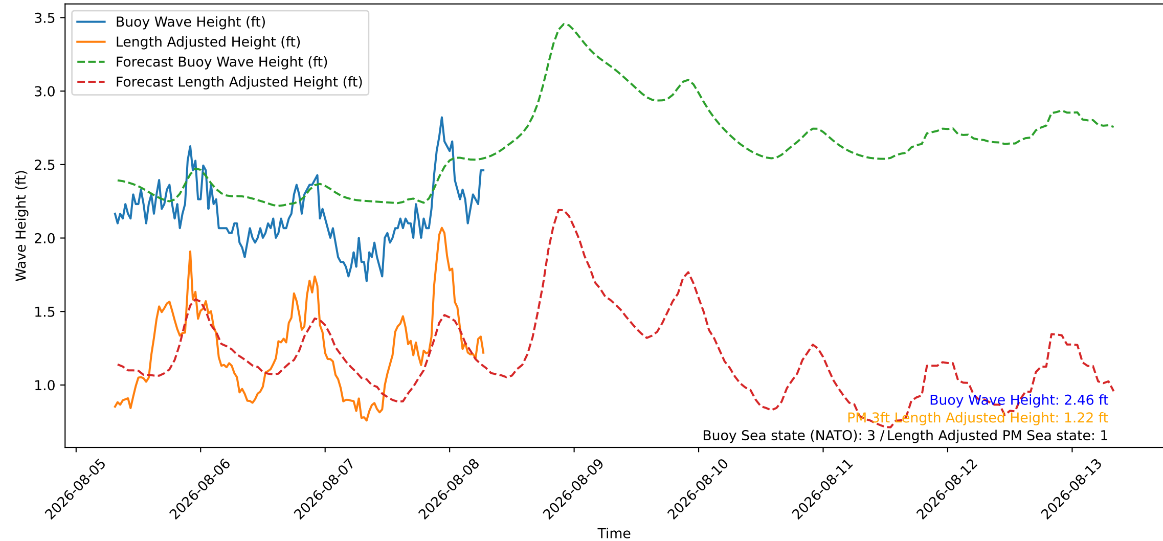
Wave Heights over Time for Green Beach at 2026-08-08 07:31:08
