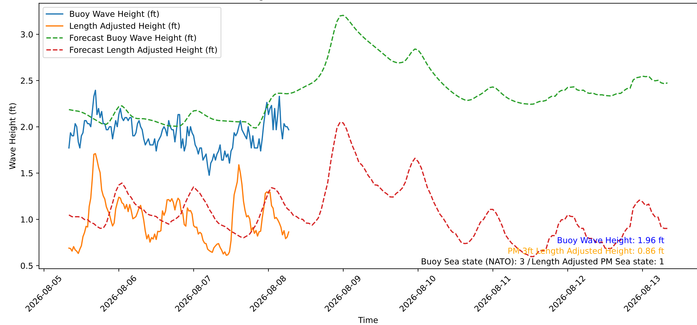
Wave Heights over Time for Red Beach at 2026-08-08 07:30:45
