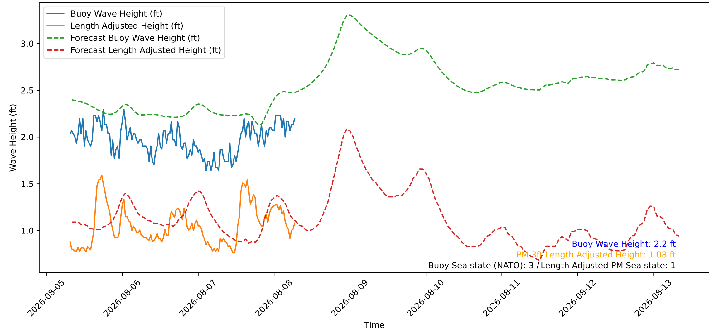
Wave Heights over Time for Oceanside Harbor at 2026-08-08 07:30:26
