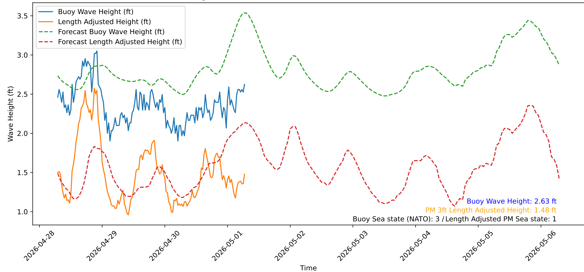
Wave Heights over Time for Oceanside Harbor at 2026-05-01 07:10:31
