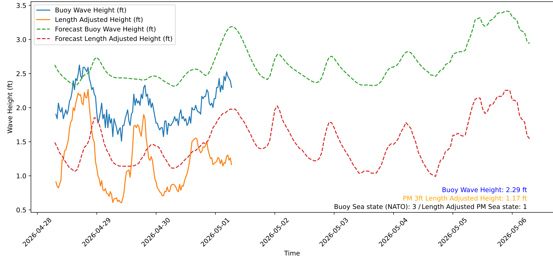
Wave Heights over Time for Red Beach at 2026-05-01 07:10:51
