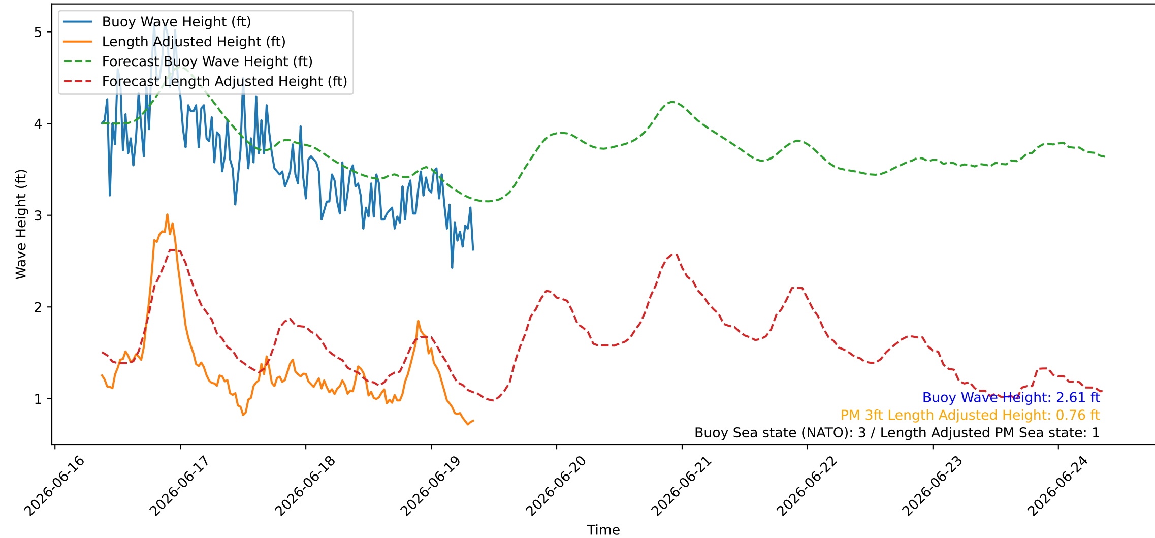
Wave Heights over Time for Green Beach at 2026-06-19 09:01:07
