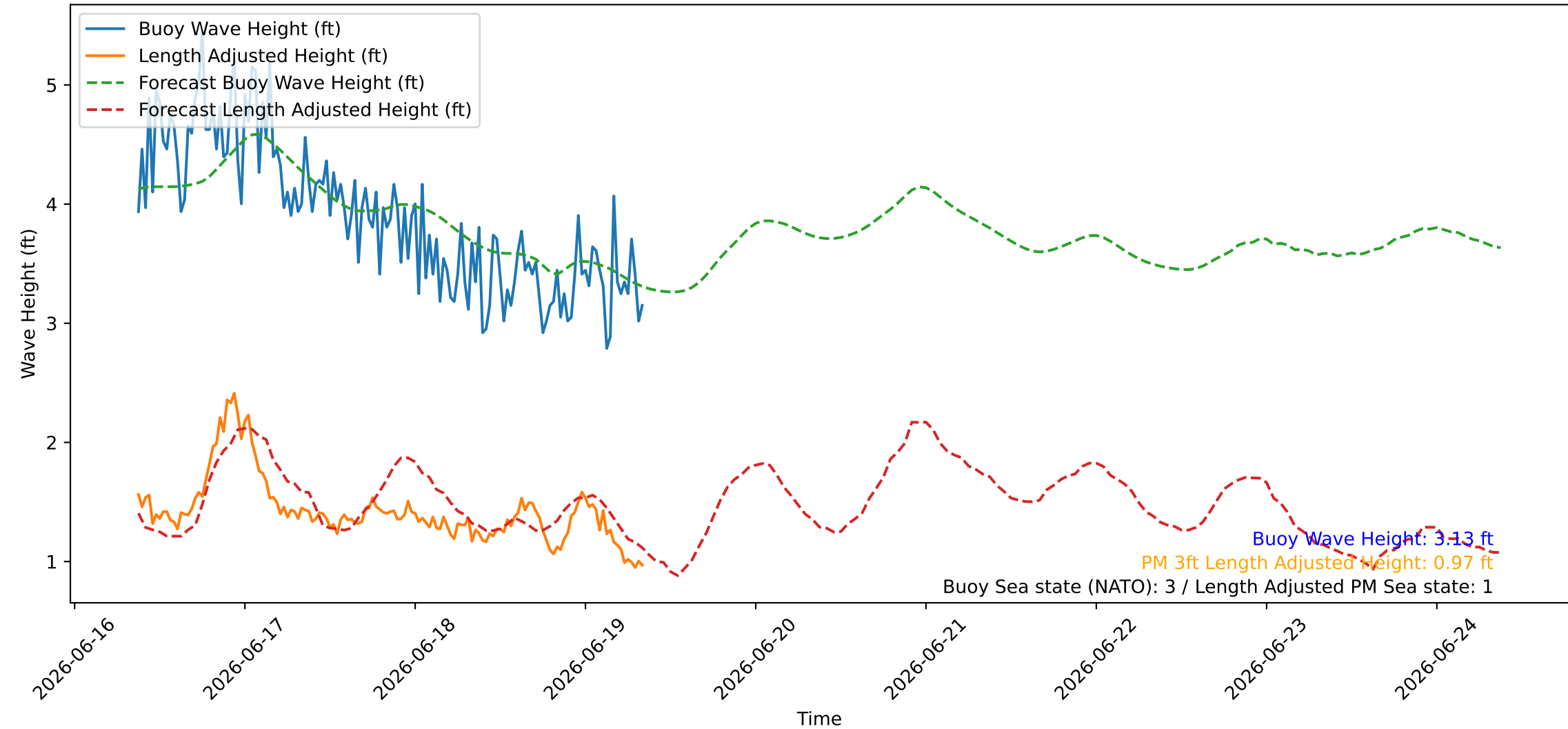
Wave Heights over Time for Oceanside Harbor at 2026-06-19 09:00:26
