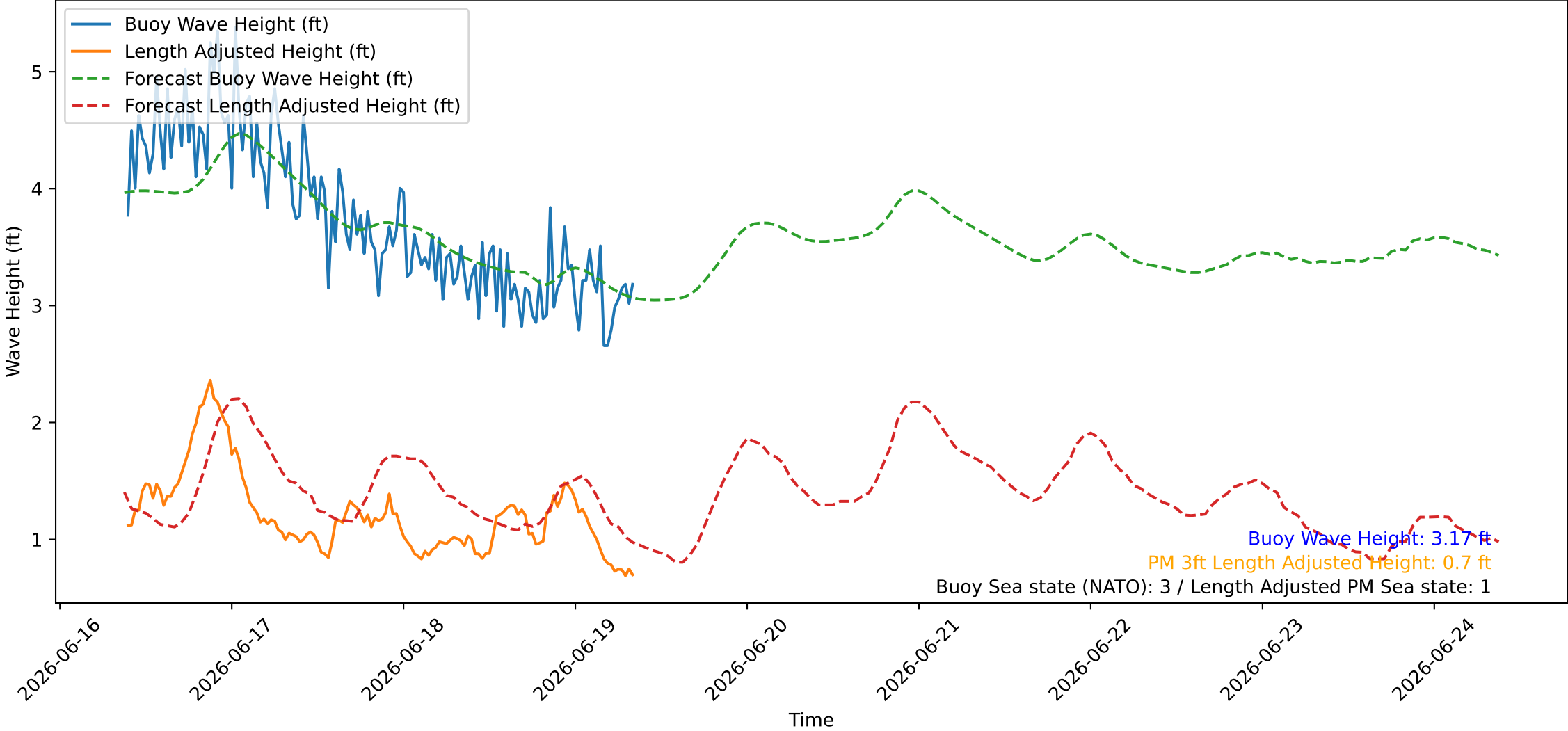
Wave Heights over Time for Red Beach at 2026-06-19 09:00:45
