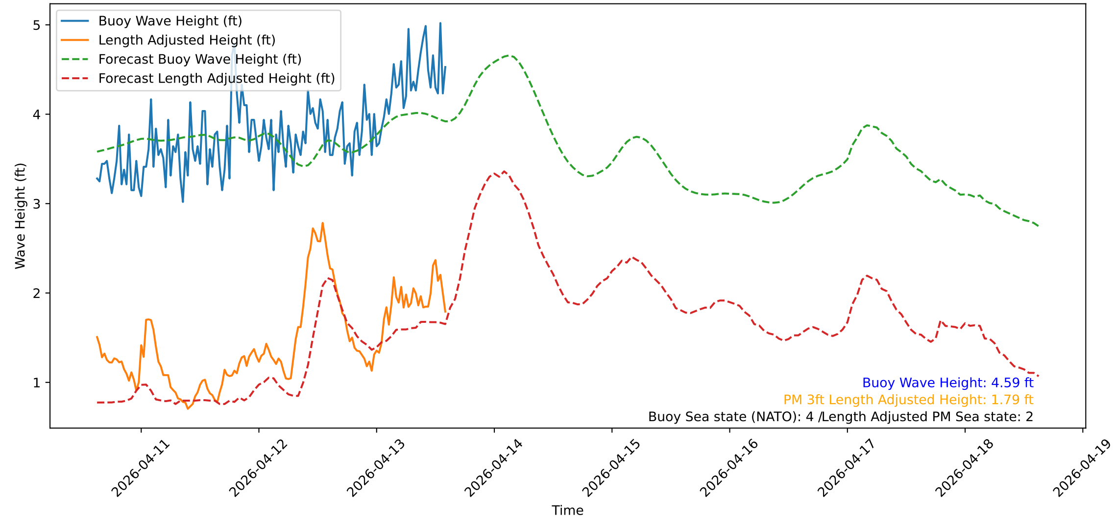
Wave Heights over Time for Oceanside Harbor at 2026-04-13 14:50:32
