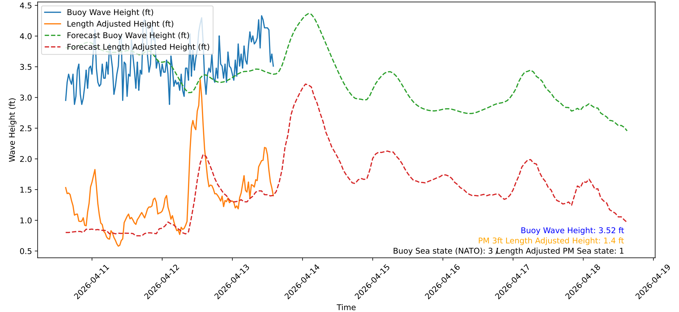
Wave Heights over Time for Red Beach at 2026-04-13 14:50:52
