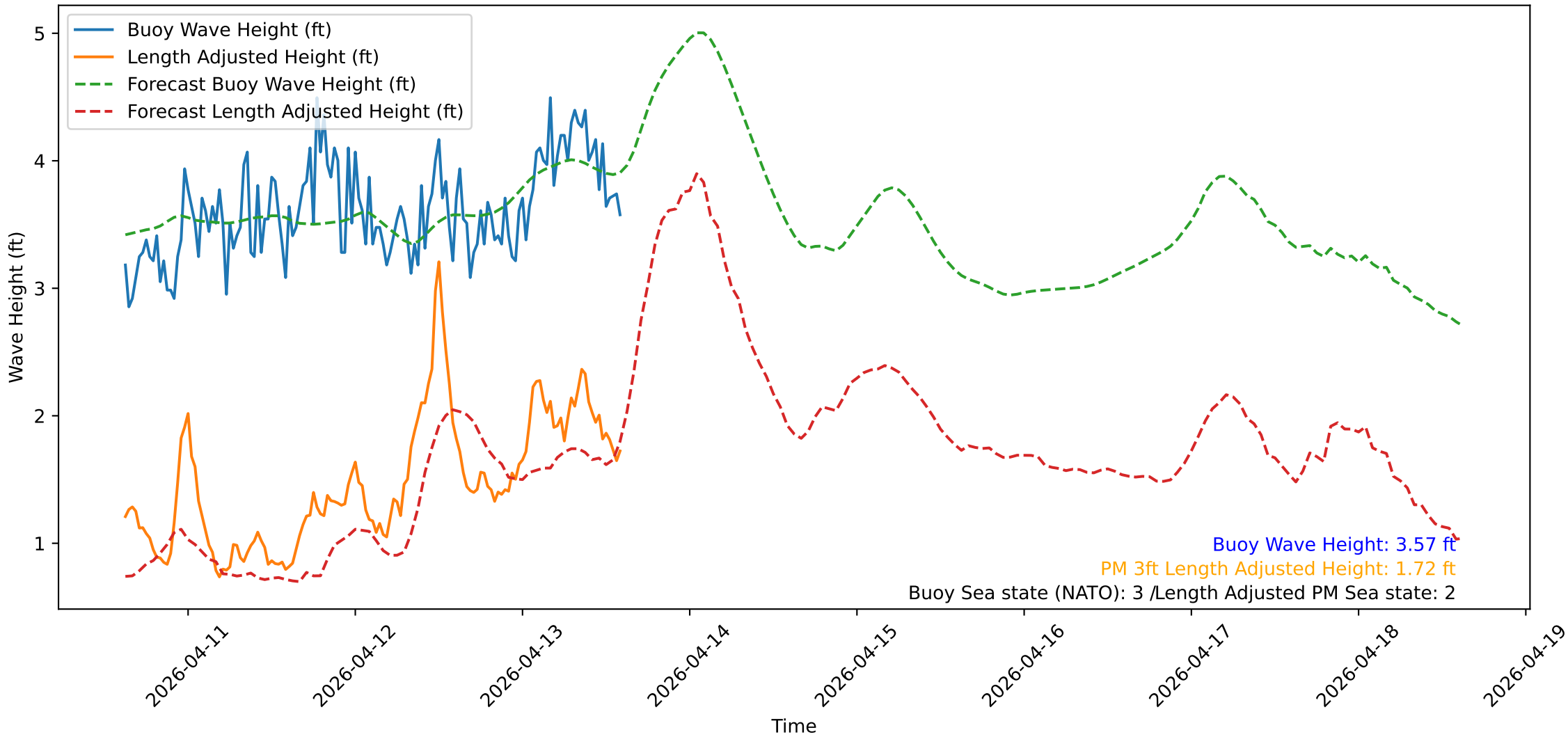
Wave Heights over Time for Green Beach at 2026-04-13 14:51:15
