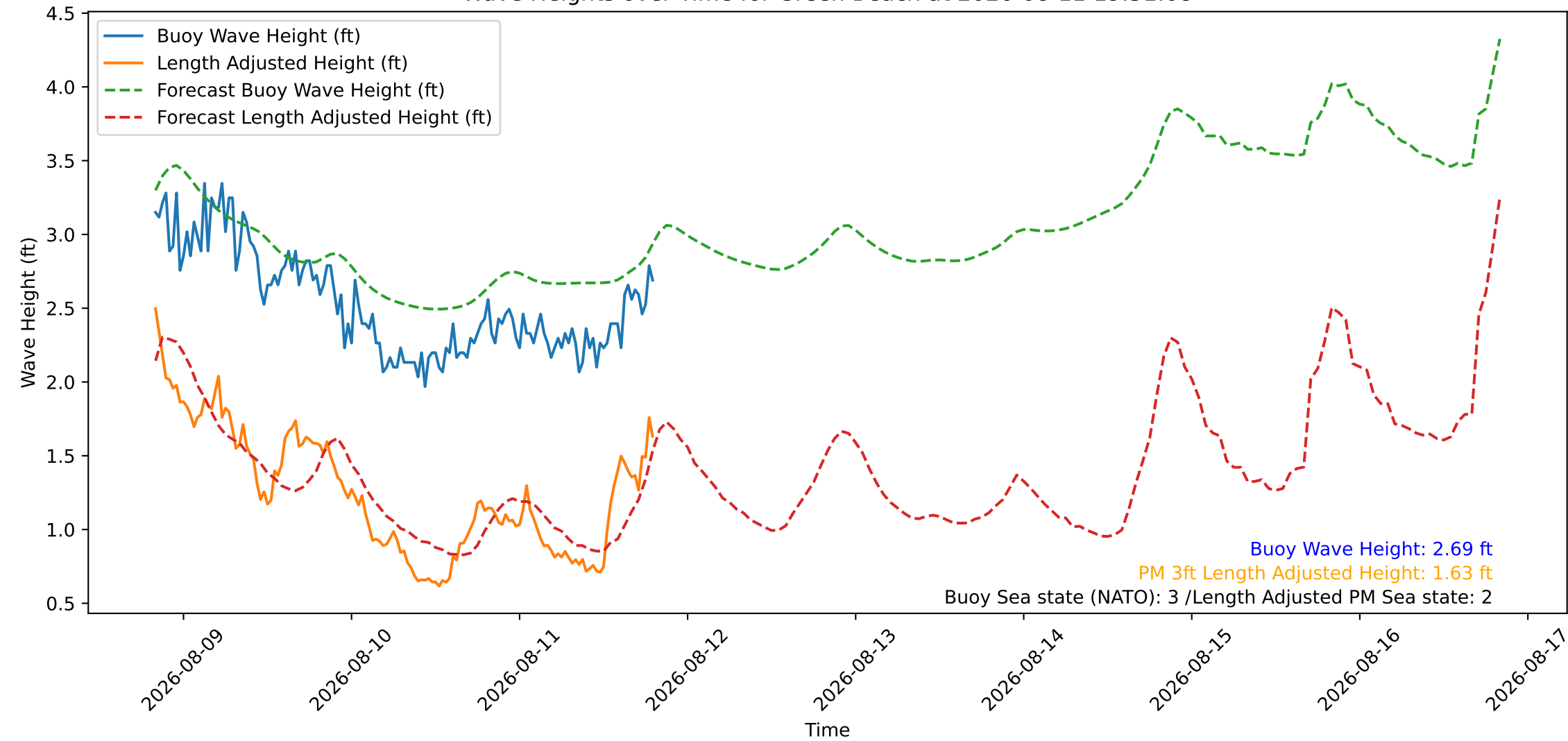
Wave Heights over Time for Green Beach at 2026-08-11 19:51:08
