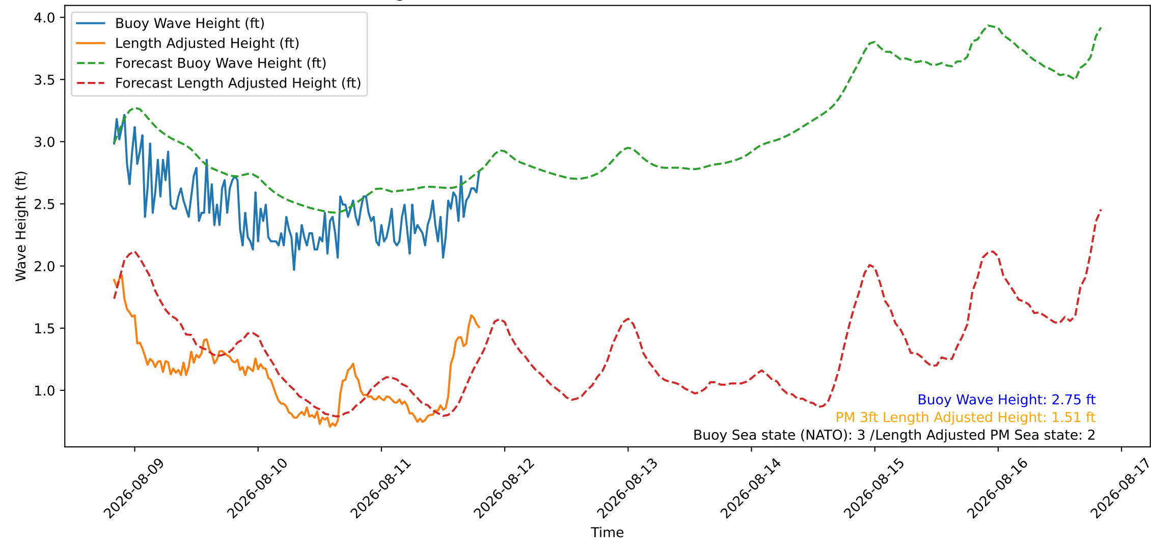
Wave Heights over Time for Oceanside Harbor at 2026-08-11 19:50:26
