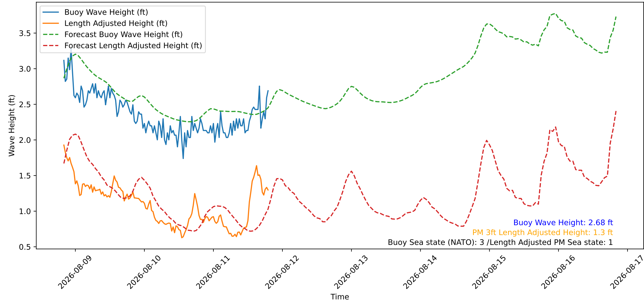
Wave Heights over Time for Red Beach at 2026-08-11 19:50:46
