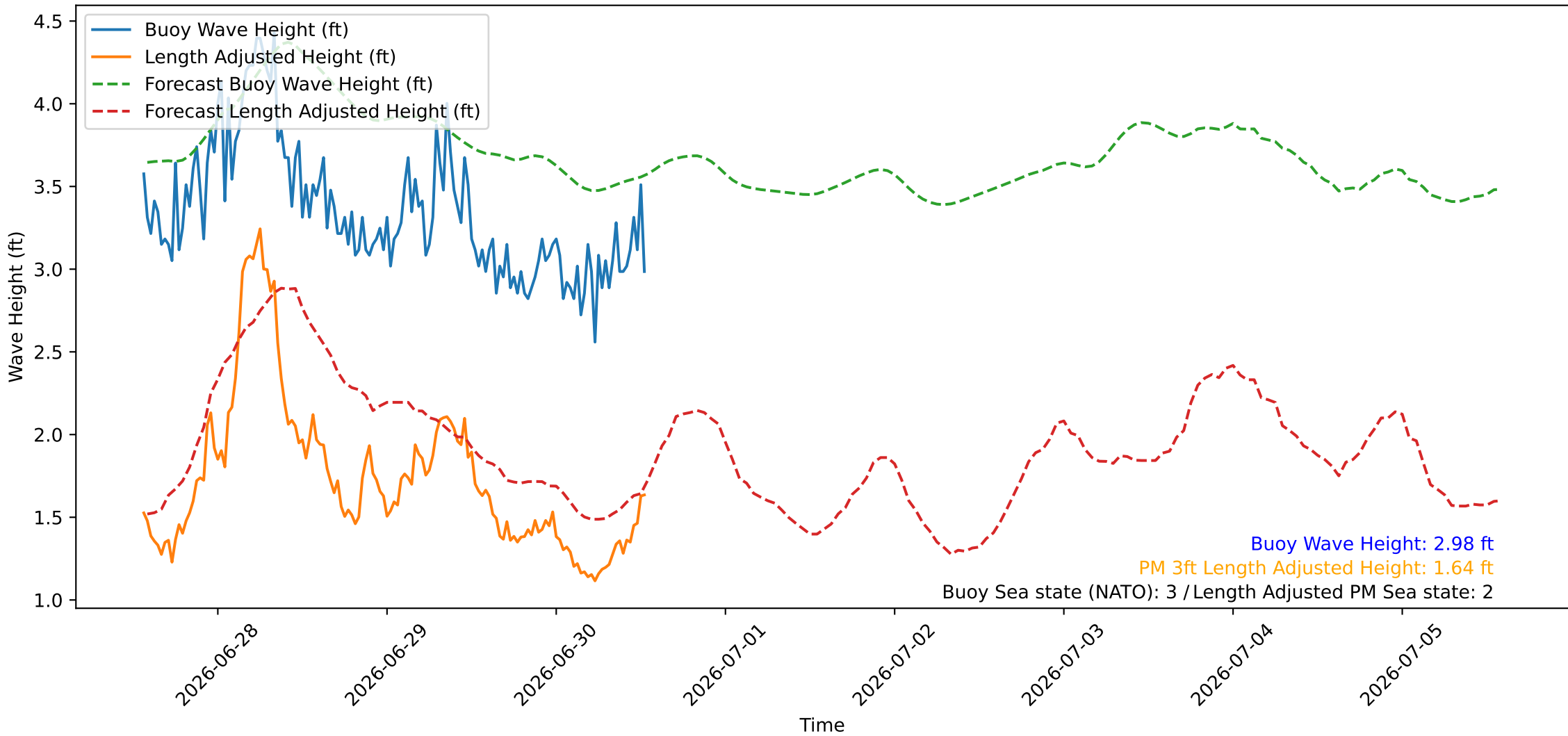
Wave Heights over Time for Oceanside Harbor at 2026-06-30 13:30:26
