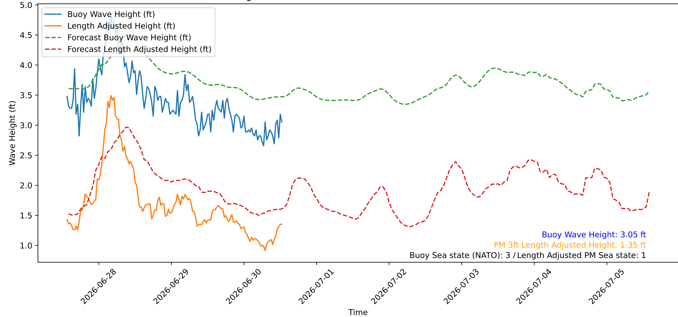
Wave Heights over Time for Green Beach at 2026-06-30 13:31:07
