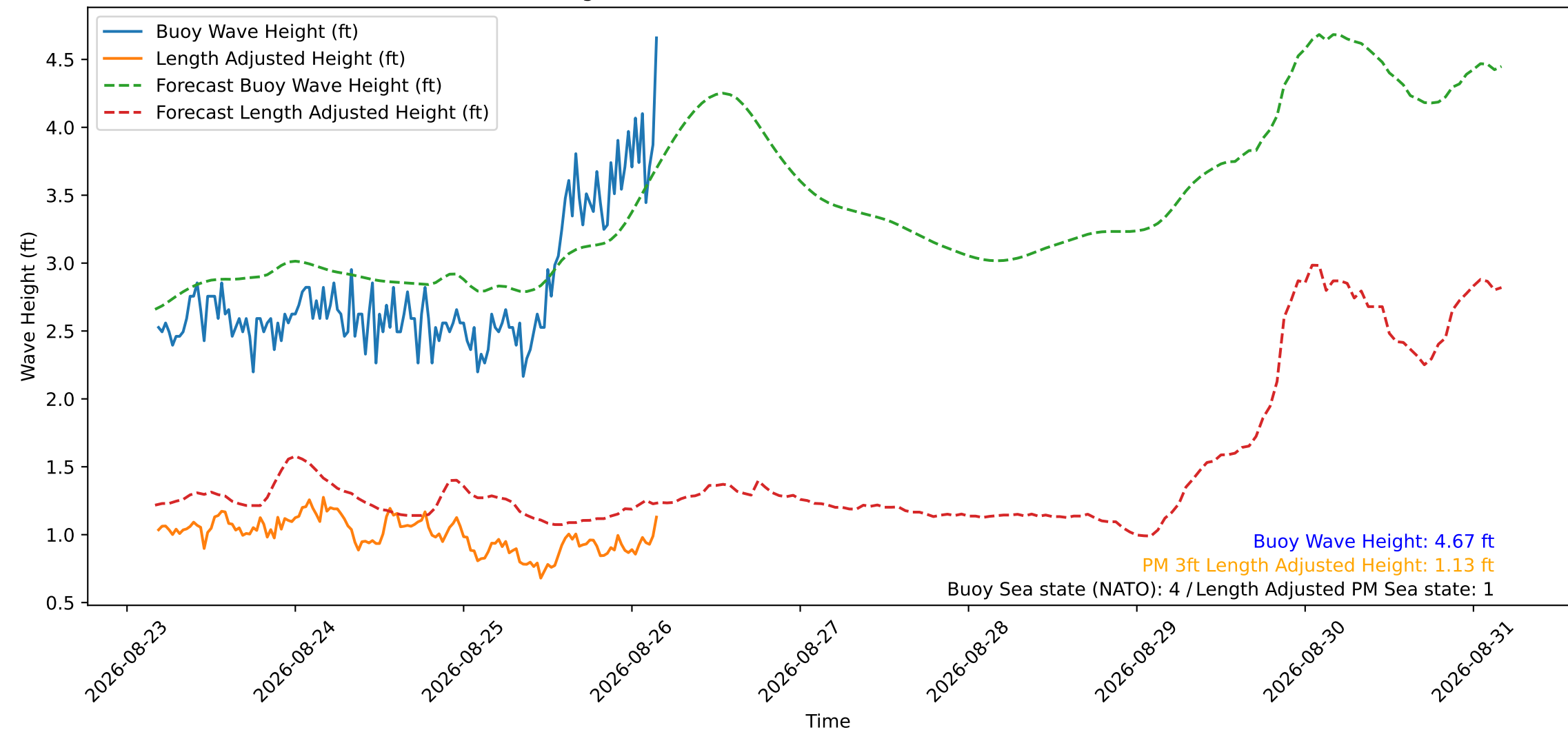
Wave Heights over Time for Red Beach at 2026-08-26 04:10:49
