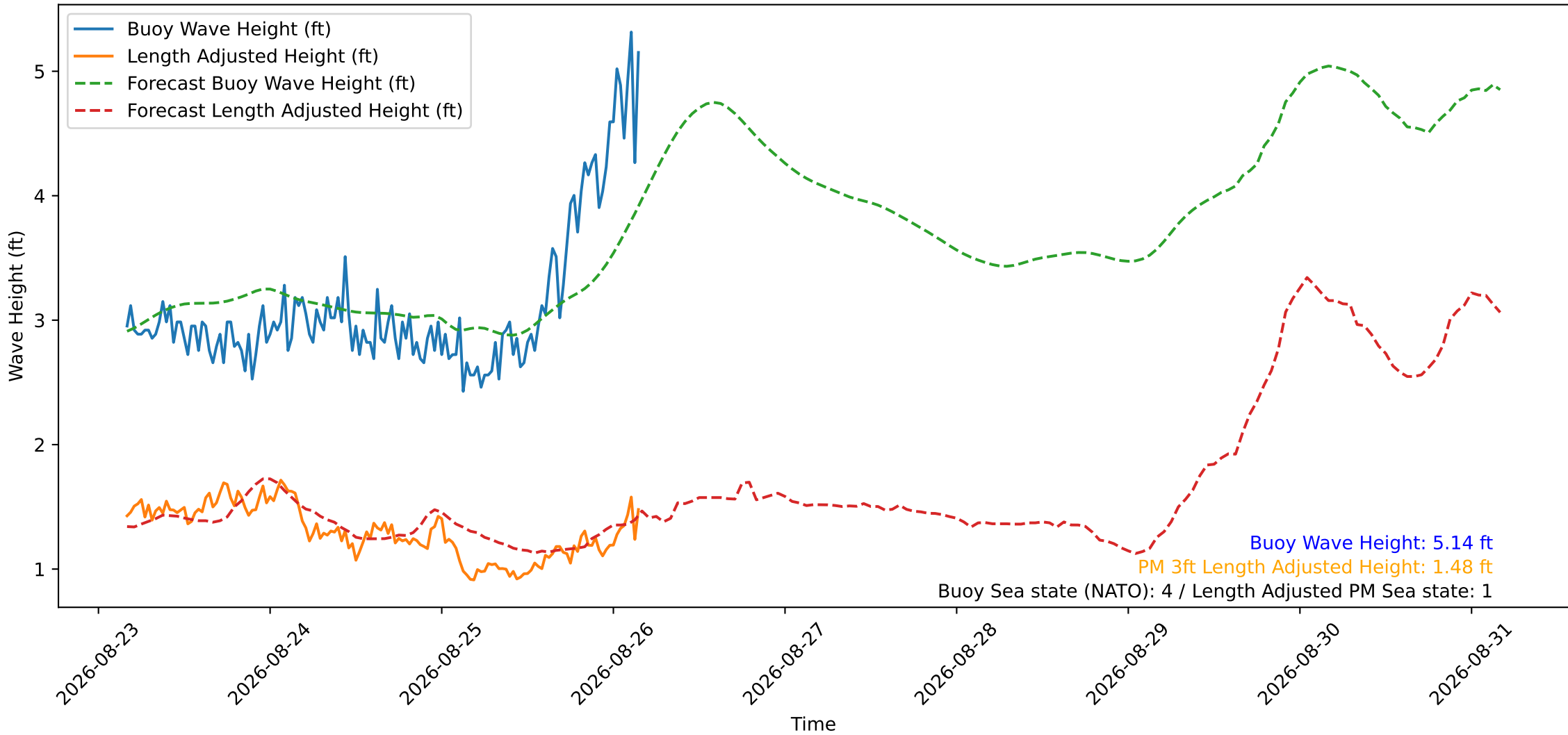
Wave Heights over Time for Oceanside Harbor at 2026-08-26 04:10:29
