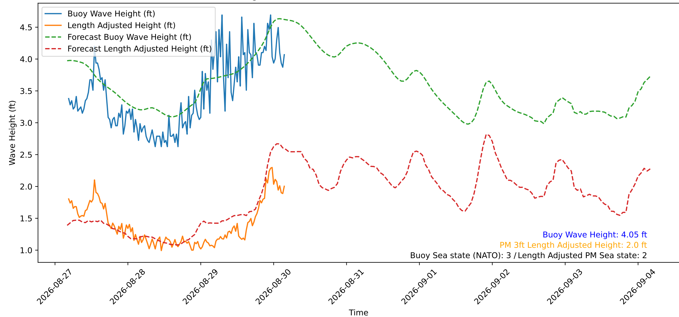
Wave Heights over Time for Red Beach at 2026-08-30 04:20:51
