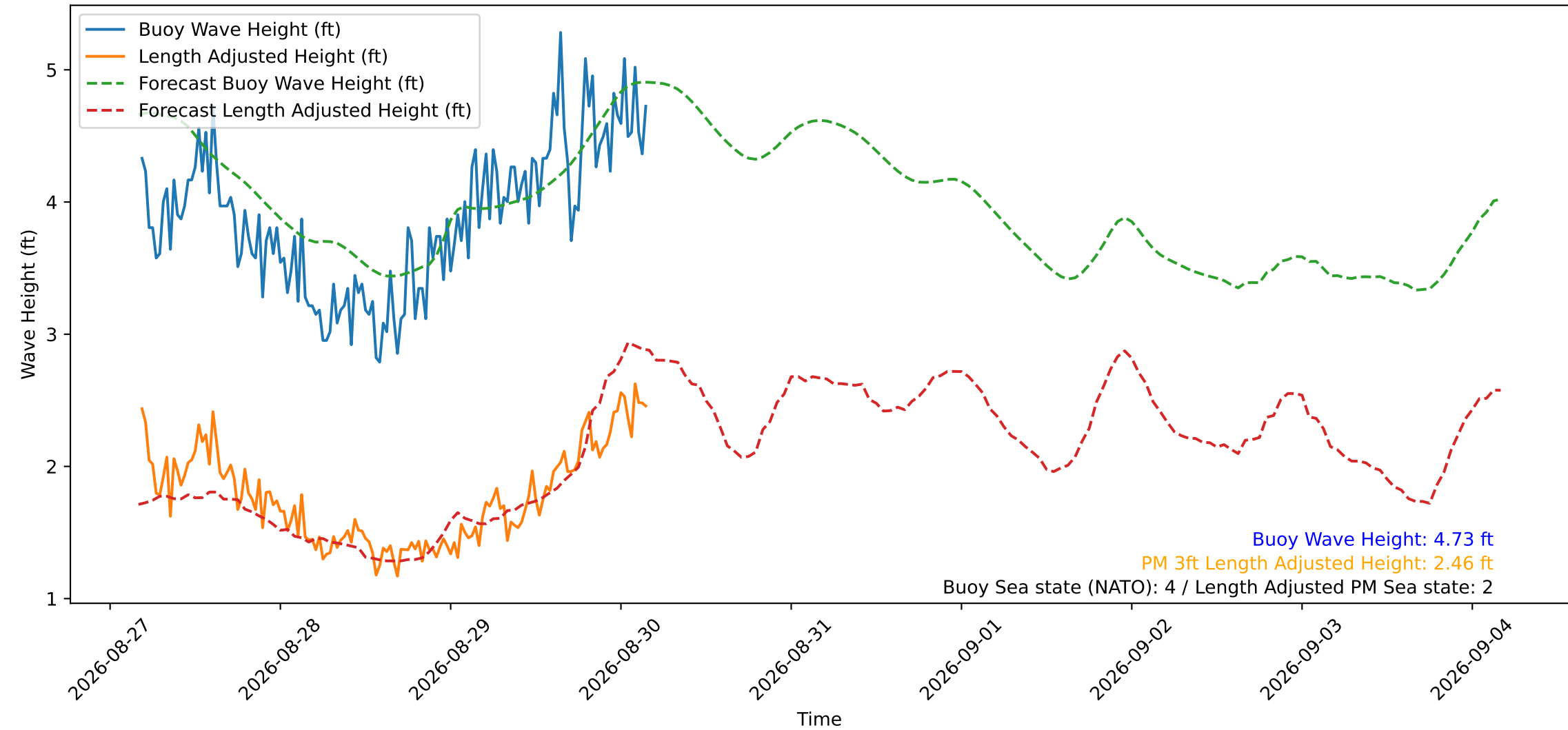
Wave Heights over Time for Oceanside Harbor at 2026-08-30 04:20:30
