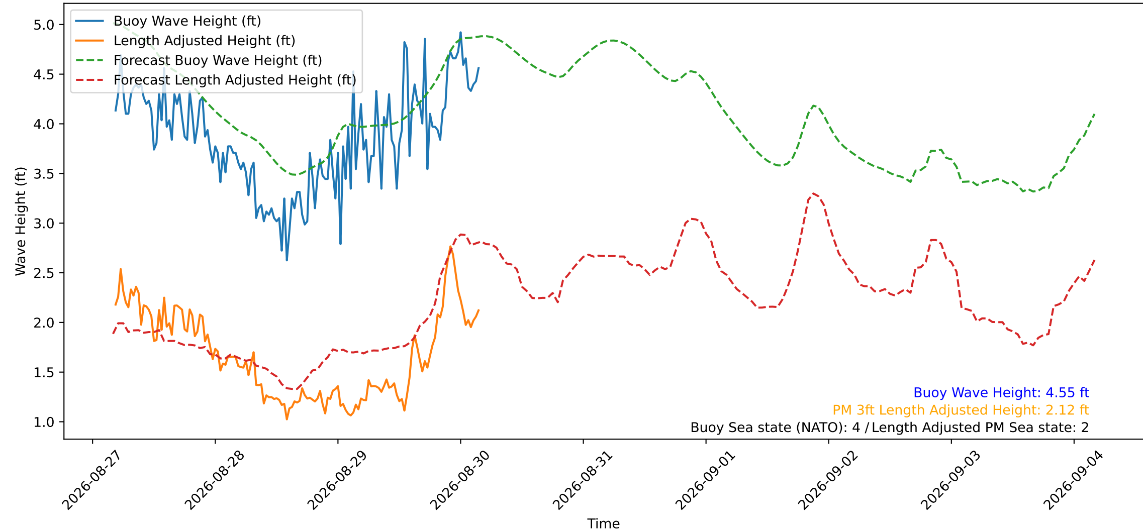
Wave Heights over Time for Green Beach at 2026-08-30 04:21:15
