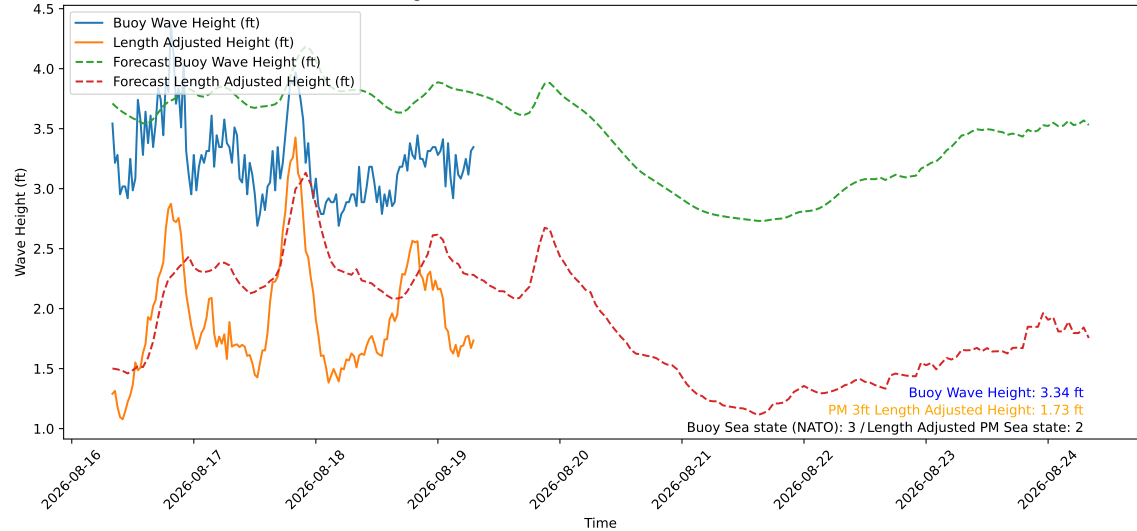
Wave Heights over Time for Green Beach at 2026-08-19 07:51:12
