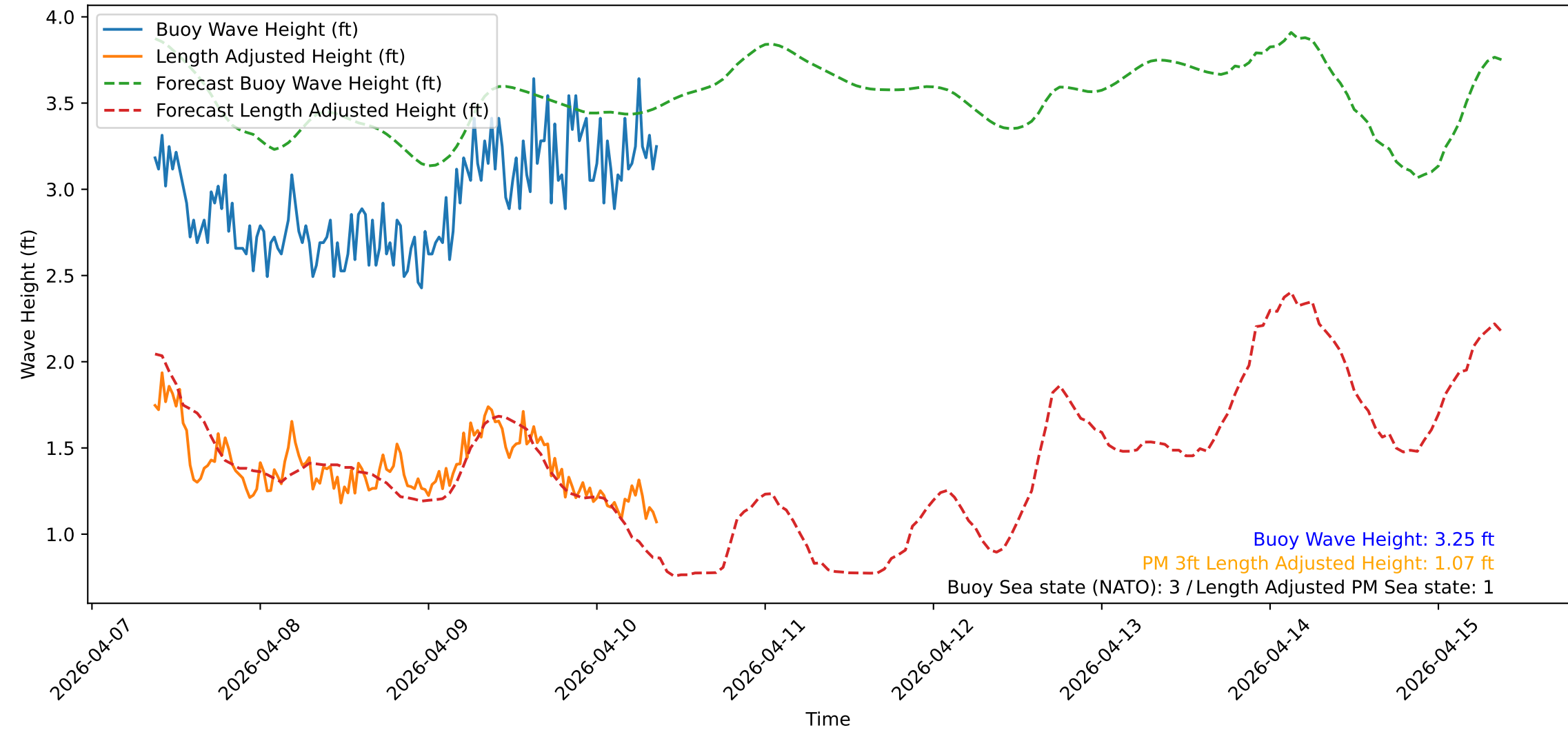
Wave Heights over Time for Oceanside Harbor at 2026-04-10 09:10:32
