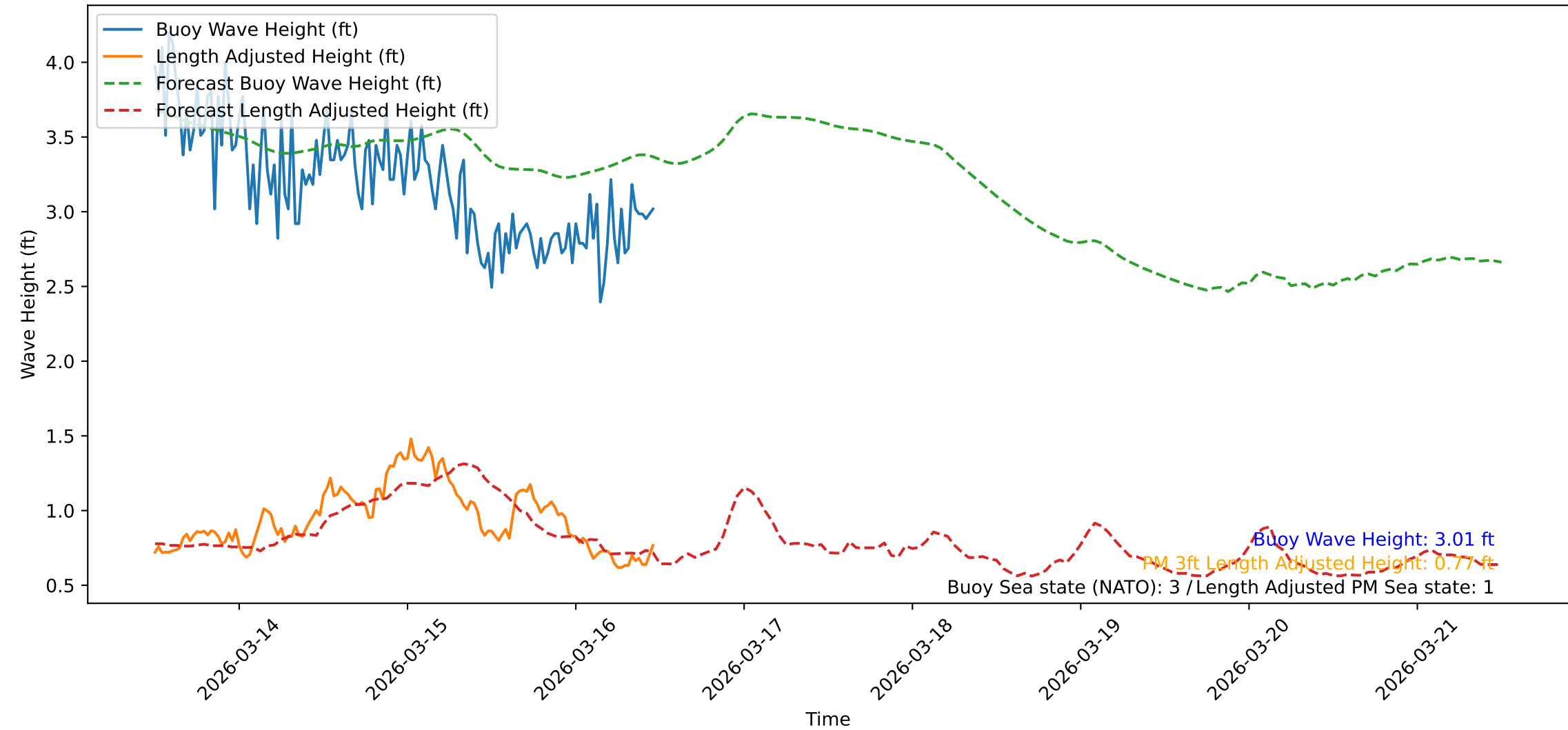
Wave Heights over Time for Oceanside Harbor at 2026-03-16 11:51:25
