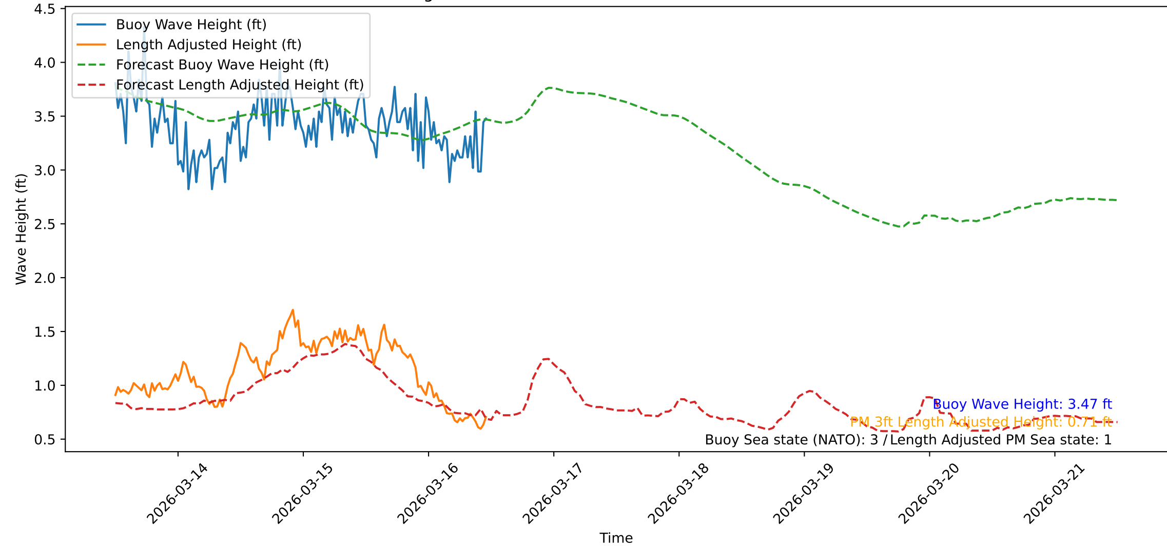
Wave Heights over Time for Green Beach at 2026-03-16 11:52:33
