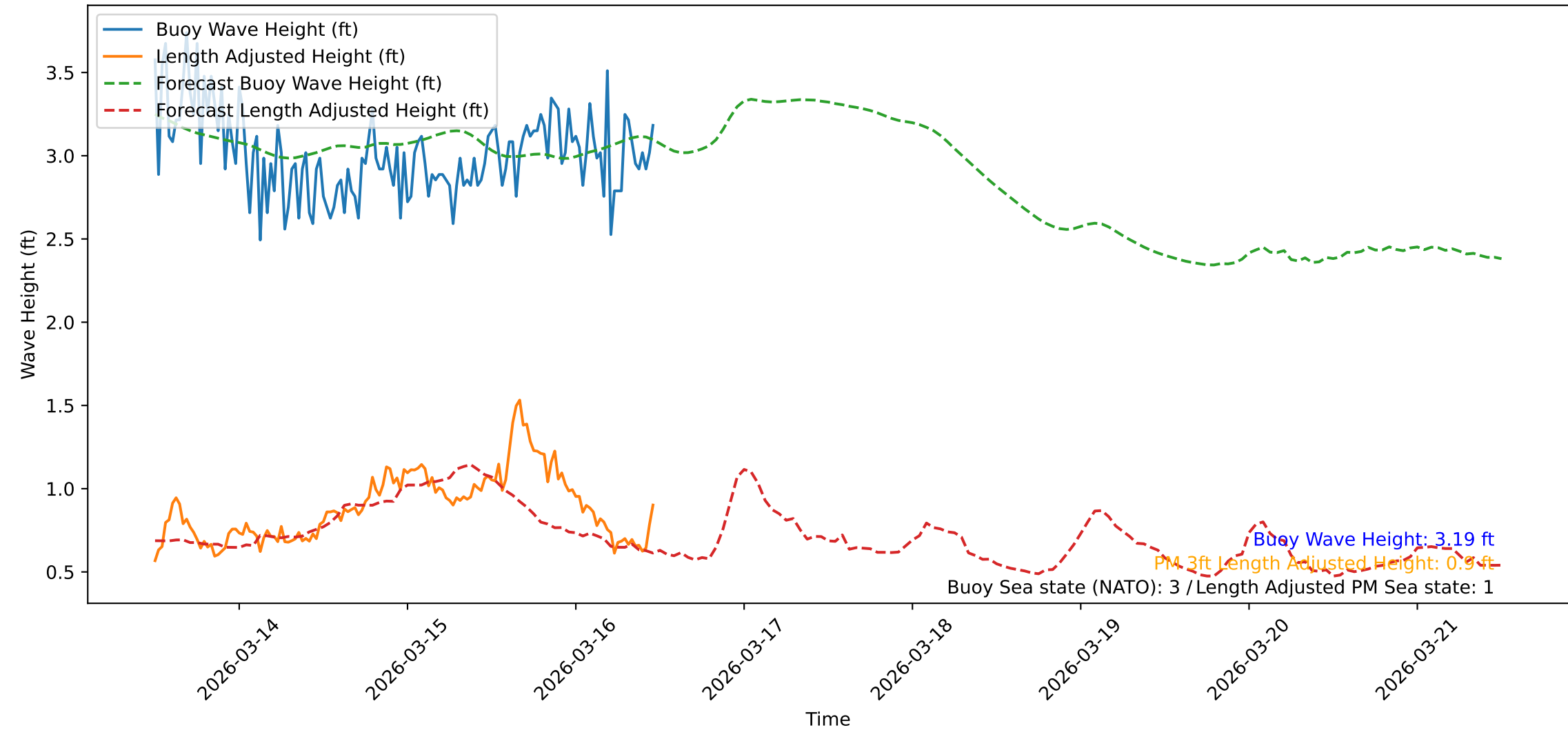
Wave Heights over Time for Red Beach at 2026-03-16 11:51:48
