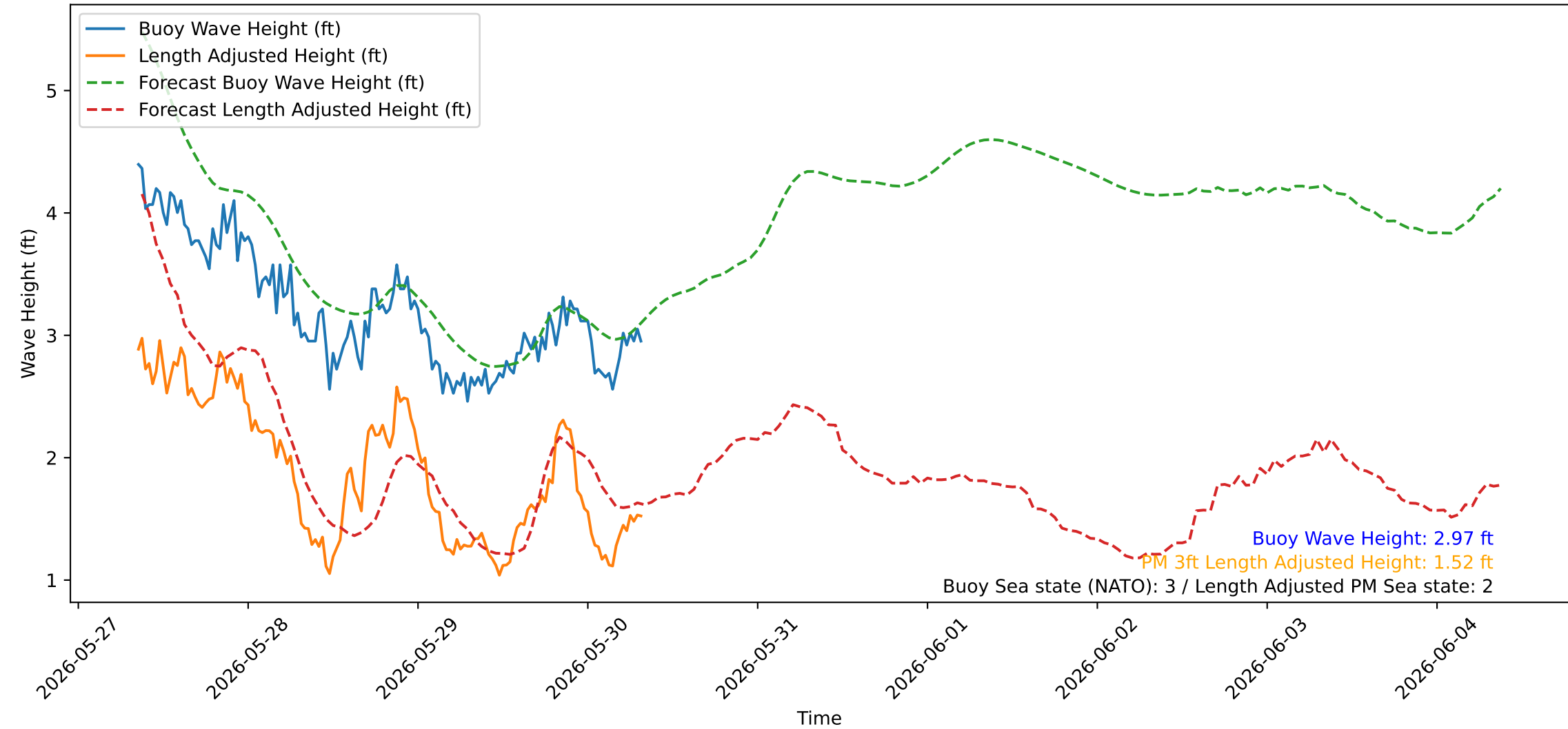
Wave Heights over Time for Green Beach at 2026-05-30 08:31:06
