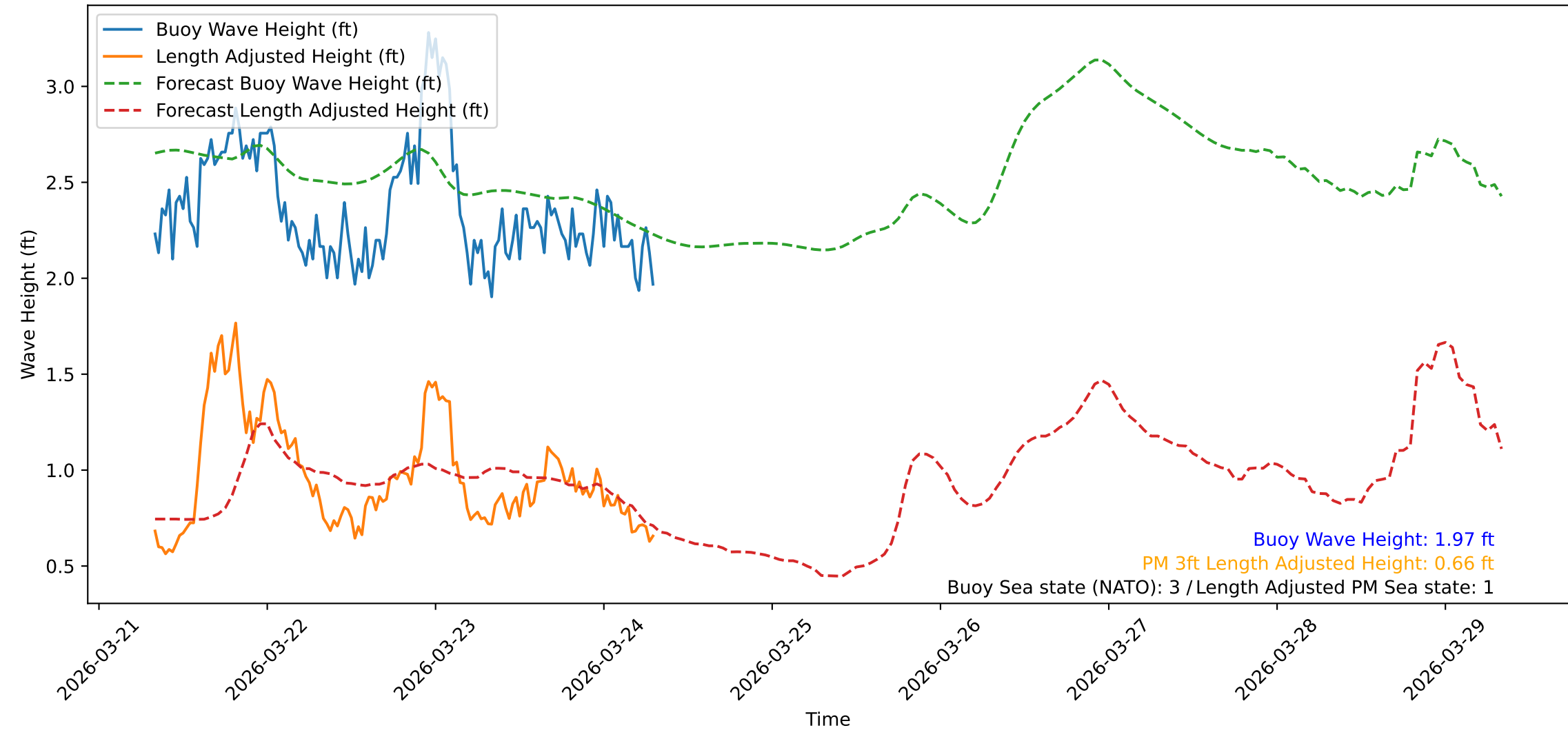
Wave Heights over Time for Green Beach at 2026-03-24 07:51:09
