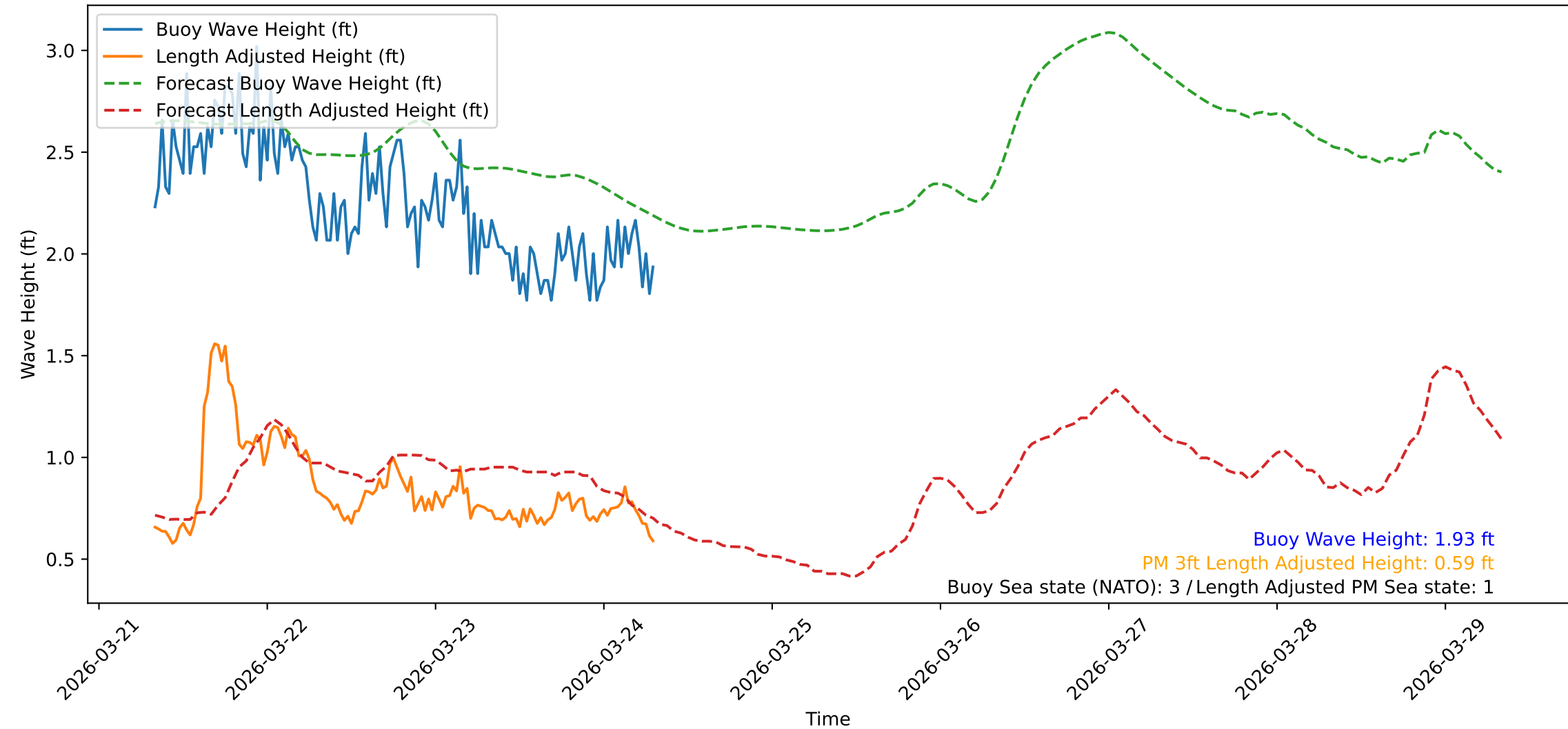
Wave Heights over Time for Oceanside Harbor at 2026-03-24 07:50:31
