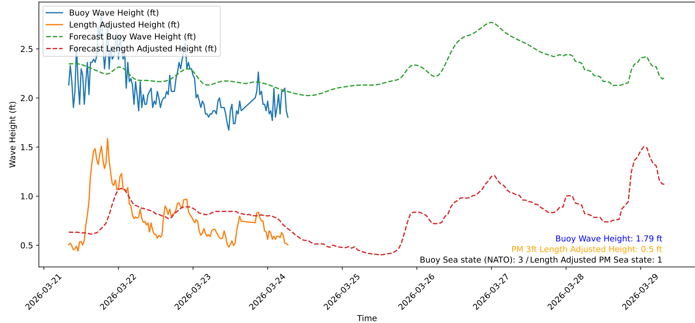
Wave Heights over Time for Red Beach at 2026-03-24 07:50:47
