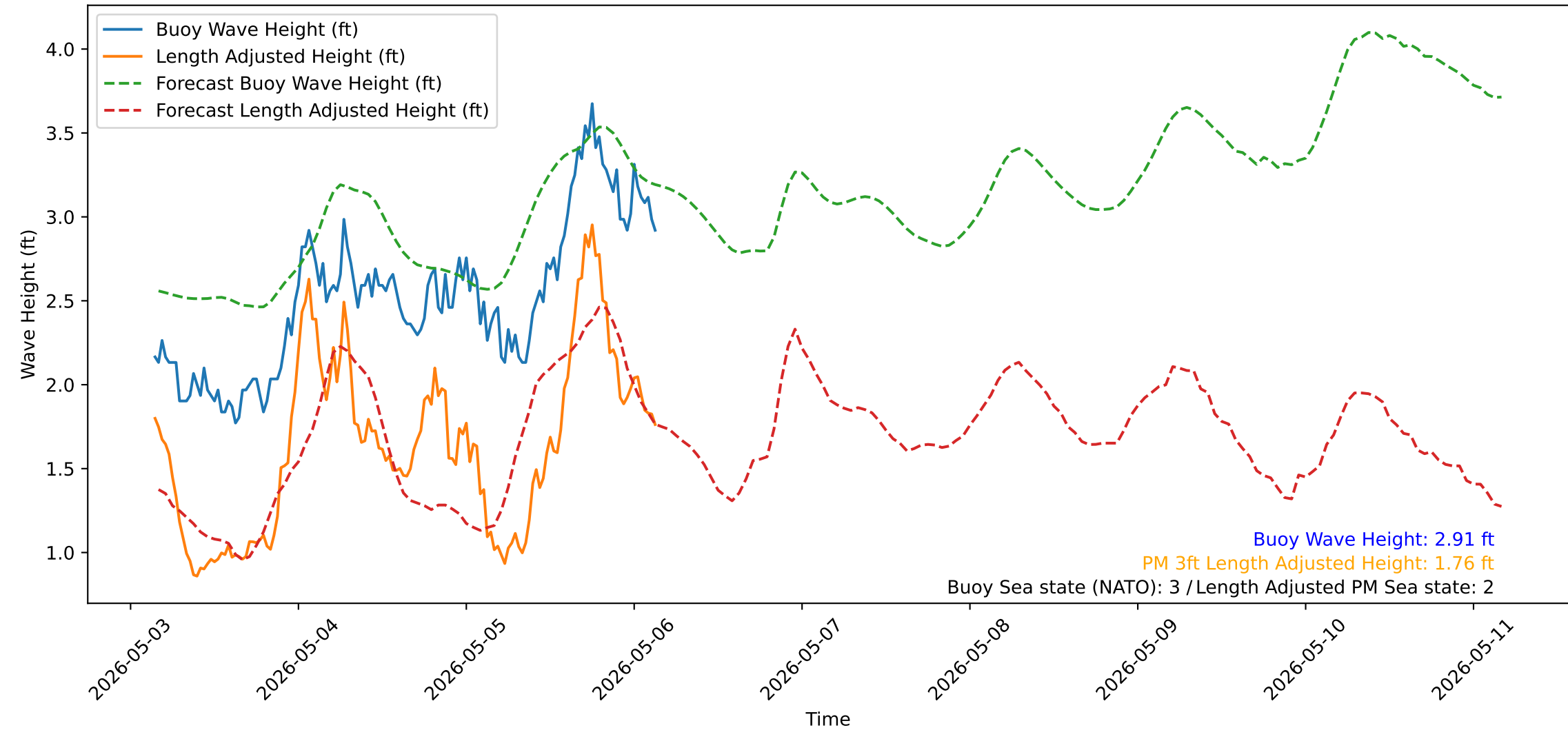
Wave Heights over Time for Green Beach at 2026-05-06 03:41:13
