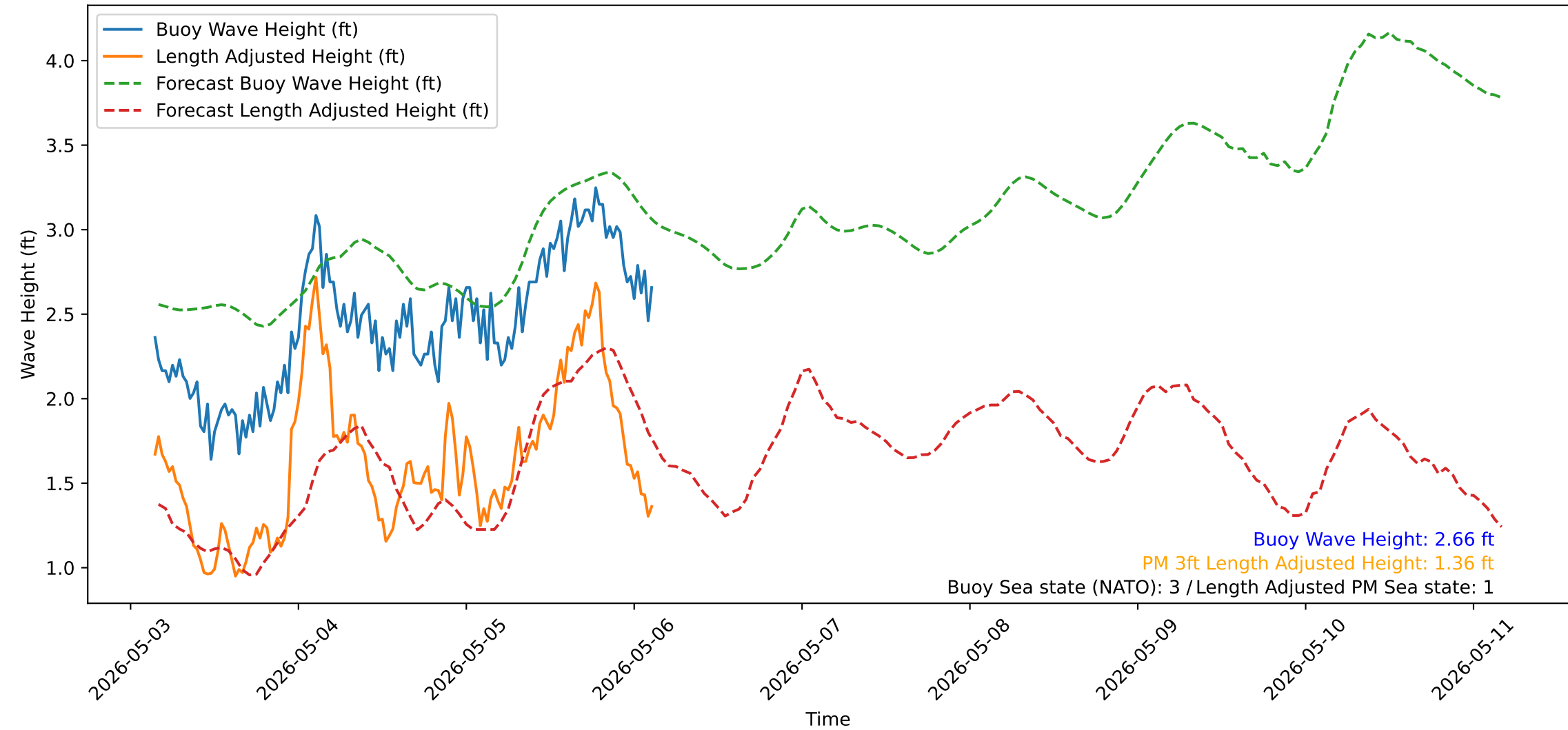
Wave Heights over Time for Oceanside Harbor at 2026-05-06 03:40:31
