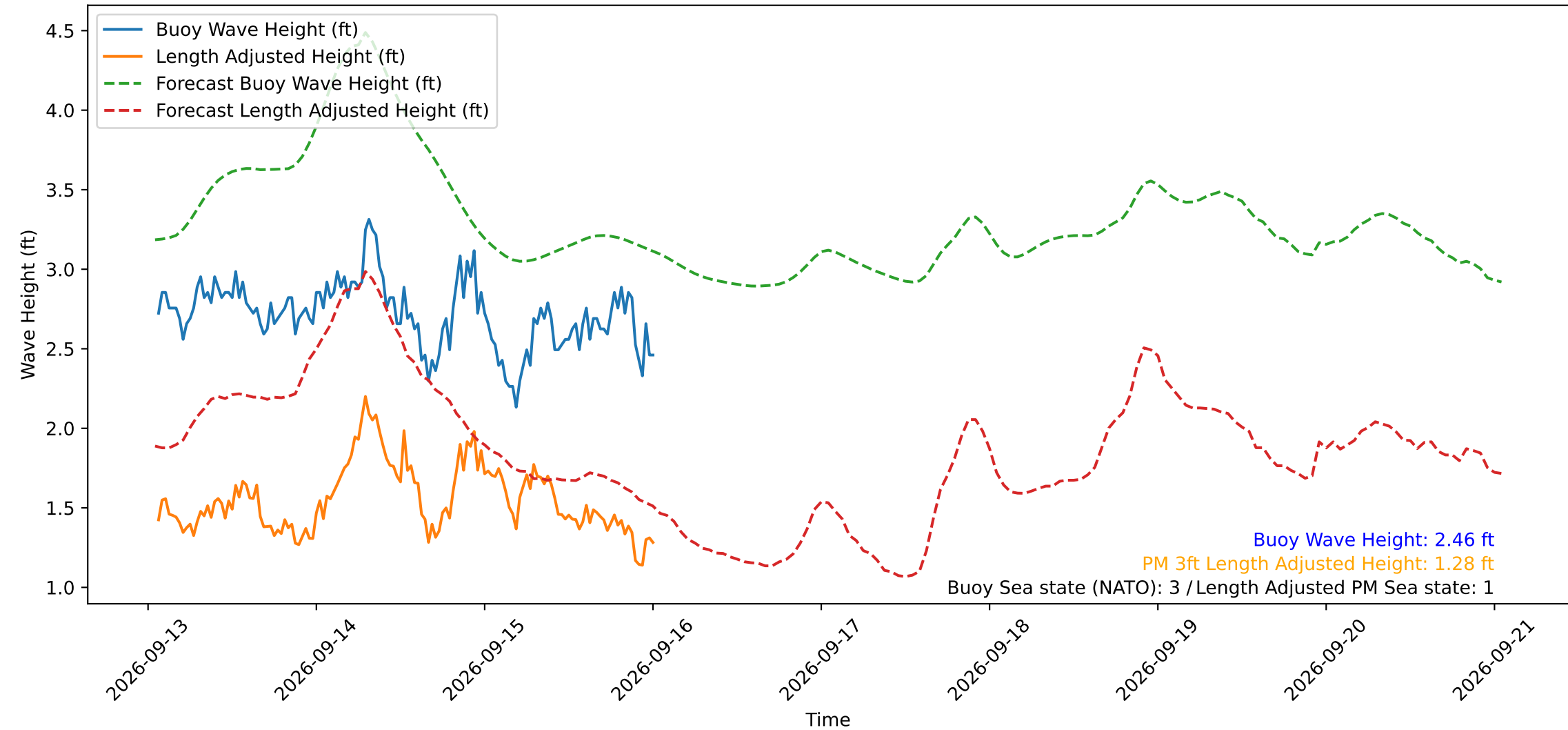
Wave Heights over Time for Green Beach at 2026-09-16 01:01:11
