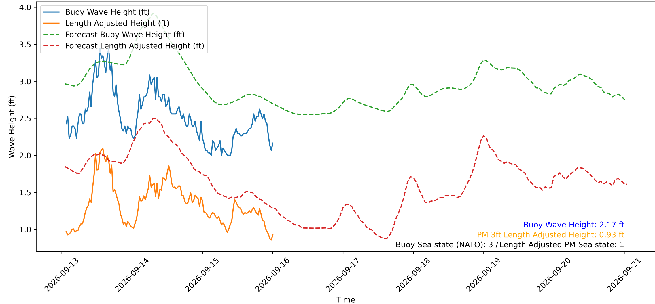
Wave Heights over Time for Red Beach at 2026-09-16 01:00:49
