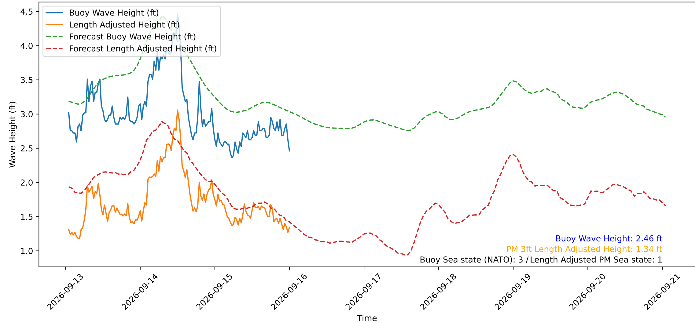
Wave Heights over Time for Oceanside Harbor at 2026-09-16 01:00:29
